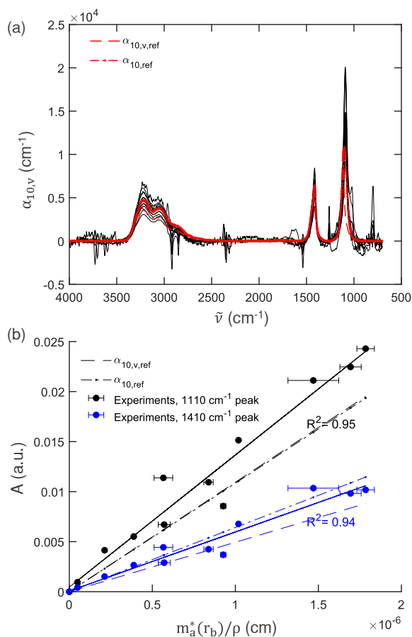
Figure 5. (a) Comparison of volume absorption coefficient ( \alpha_v ) from the experiments for IR measurement with an aperture of 6mm against the reference linear absorption coefficient ( \alpha_{\text{ref}} ) and volume absorption coefficient ( \alpha_{v,\text{ref}} ) for ammonium sulfate calculated using n and k (Earle et al., 2006). (b) Response of IR absorbance ( A ) against the effective deposition thickness (cm) of the total particle collected reference from CPC calculated using image analysis, for absorbance at the peak near 1110 \text{cm}^{-1} (for \nu_3(\text{SO}_4^{2-}) ) and at the peak near 1410 \text{cm}^{-1} (for \nu_4(\text{NH}_4^+) ).
