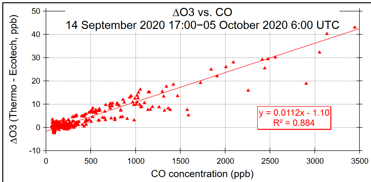
145 Figure 1: Difference in O 3 readings between the Thermo-Fisher and Ecotech UV instruments vs. CO for a 3-week period starting 14 September 2020. During this period, the Thermo-Fisher instrument gave readings that were up to 45 ppb higher than the Ecotech instrument. Values are hourly averages.
