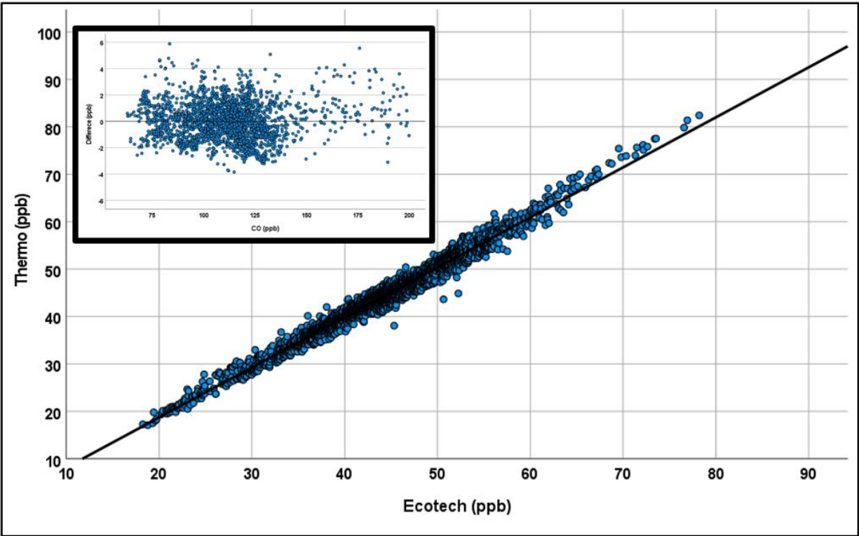
150 Figure 2: O 3 measured by the Thermo-Fisher 49c instrument vs. Ecotech instrument at MBO during non-smoke periods (defined as CO < 200 ppb). Data are hourly averages of all valid data for both instruments in 2020. The inset shows a difference plot (Thermo-Ecotech) vs. CO for the same data. The root mean squared error (difference) of the Thermo vs. Ecotech plot is 0.9 ppb, and the linear regression line has a slope of 1.055, a y-intercept of -2.4 ppb, and an R 2 of 0.98.
