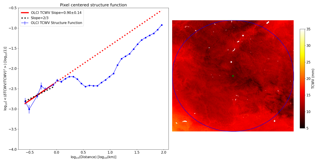
Figure 6. Pixel centered structure function for the OLCI COWa TCWV shown in the left plot together with its uncertainty in the vertical axis (blue curve), a linear fit of the points below 10^0 km (red curve) and a two-third slope line (black dots). The structure function covers the area inside the blue circle shown in the right TCWV image which has a radius of 100 km and it is centered in the green dot. This region is a zoom of the bottom right region highlighted in blue from Fig. 3. Cloudy classified pixels are plotted in white.
