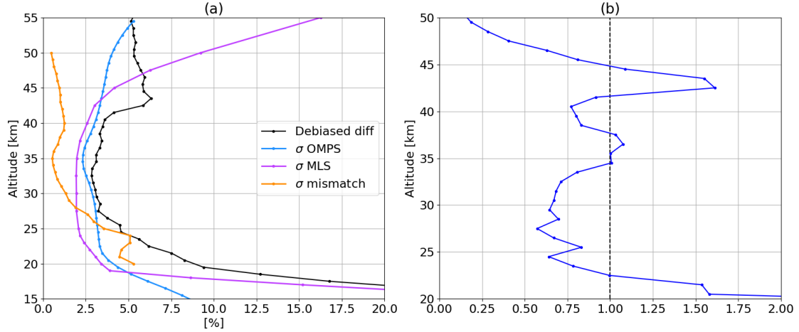
Figure 15. In panel (a), contributing terms from Eq. 16 and de-biased rms difference between OMPS-LP and MLS (numerator of Eq. 15). In panel (b), \chi^2 values obtained as validation metric for the combined OMPS-LP and MLS uncertainty.
