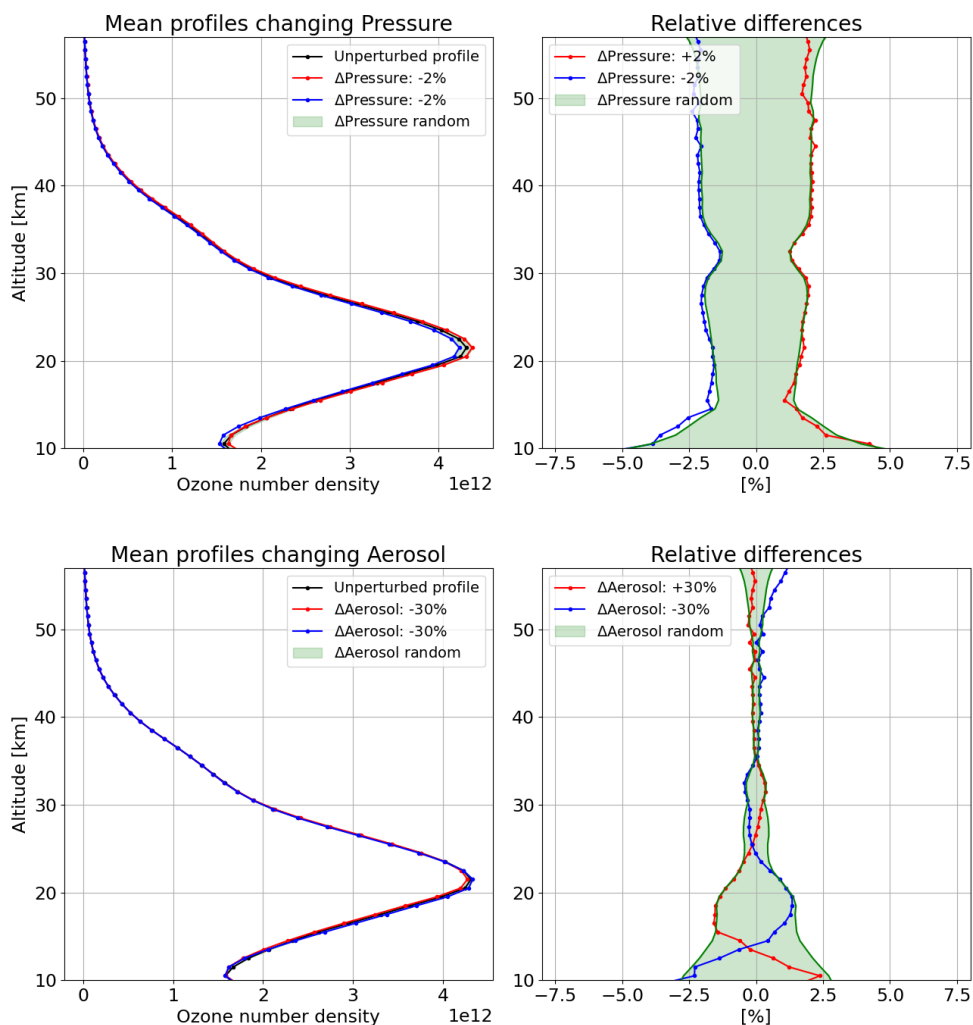
Figure 5. In the left panels the unperturbed ozone profile is shown together with the mean ozone profiles obtained by perturbing in the forward simulation left pressure and aerosol extinction by 2% and 30%, respectively, in a Monte Carlo - like approach. The green shaded area shows the standard deviation of the 50 profiles obtained with the second approach. In the right panels, \sigma_{x,pert\_fix} and \sigma_{x,pert\_rand} are shown in relative values.
