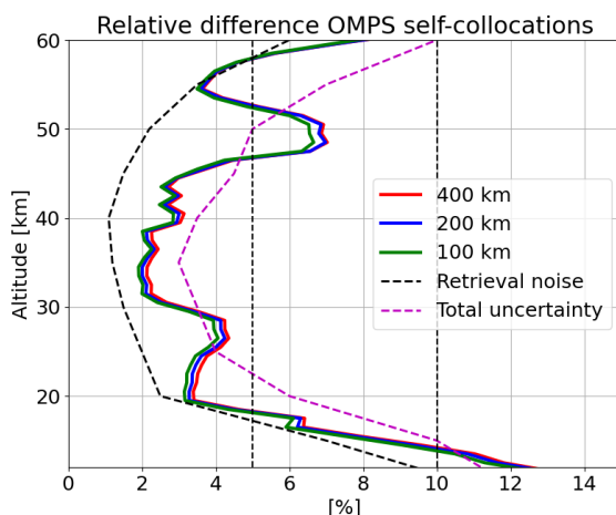
Figure 14. Relative difference between self-located OMPS-LP observations when changing the collocation criteria. Superimposed, typical retrieval noise and total random uncertainty for high latitudes.
