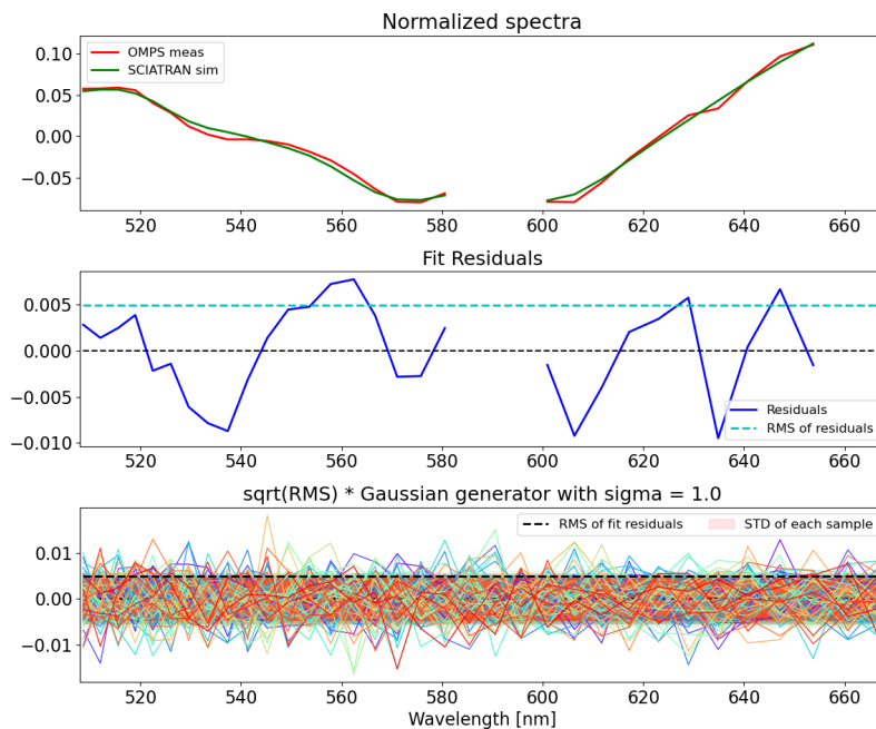
Figure 3. Example of spectra, fit residuals and randomly generated noise sequences in the Chappuis band. The square root of the fit residuals (rms) is equal to the standard deviation (STD) of each generated noise sample.
