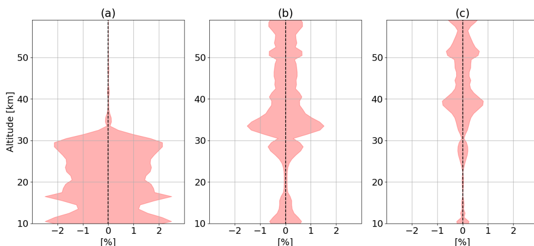
Figure 9. Standard deviation of 50 retrieved ozone profiles, using a perturbed cross section: in panel (a) adding a random bias of 2% (constant over wavelength) in the Chappuis band, and in panel (b) adding random noise with an amplitude of 2% in the UV. Panel (c): standard deviation of 50 ozone profiles after perturbing the temperature and pressure profiles to investigate the uncertainty from the cross section temperature dependence.
