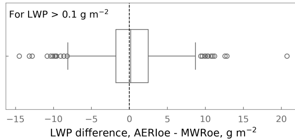
Figure 8. The differences in retrieved liquid water path (LWP) between all AERIOe the MWRoe retrievals ( LWP > 0.1 \text{ g m}^{-2} ). 50% of all retrievals fall within the central box, 90% of all retrievals fall within the box plot ‘whiskers’, and the remaining data are plotted as outliers (circles).
