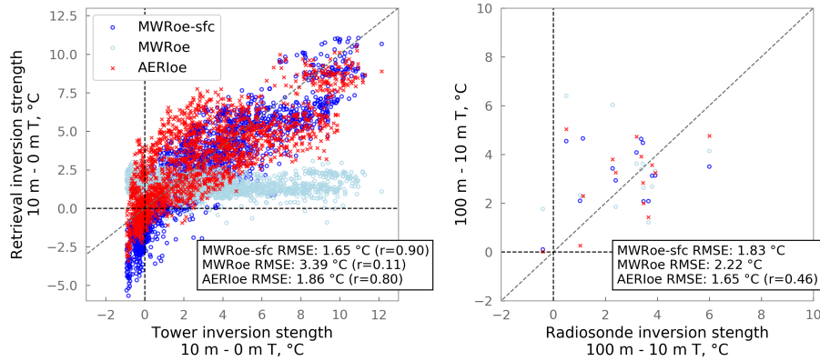
Figure 6. (a) Inversion strength (10 m – 0 m T) retrieved from the AERloe (red), the MWRoe (light blue), and the MWRoe-sfc (dark blue) versus observations from the tower mounted HMP155 probes. (b) The same as (a) except for the 100 m - 10 m inversion strength compared to observations from 14 coincident radiosonde profiles. On both subplots the diagonal grey dashed line represents perfect agreement and the horizontal and vertical dashed black lines at 0°C delineate when a surface based temperature inversion is present (right quadrants) versus absent (left quadrants). The root mean squared error (RMSE) values are included on the plots and the Pearson’s correlation coefficients (r) are only included when they are significant at the 90% confidence level.
