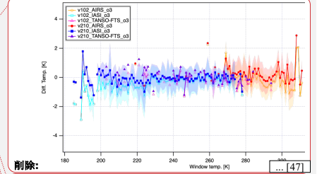
Figure 5: The channel-dependent brightness temperature difference in 1 K bins against atmospheric window temperature for SNO condition between TANSO-FTS-2 and AIRS/IASI/TANSO-FTS. (a) CO 2 spectral range, (b) CH 4 spectral range, (c) O 3 spectral range, (d) atmospheric window channel. The filled dots are the data points, and each shade presents a standard deviation (1σ) for each 1 K bin.
