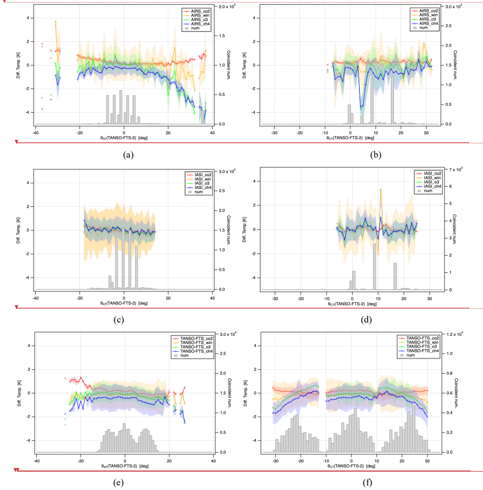
255 Figure 7: The channel dependent brightness temperature difference in 1^\circ angular bin average against TANSO-FTS-2 \theta_{ATV} (left) and \theta_{CTV} (right) for 20-SONO for AIRS, IASI and TANSO-FTS. The shaded areas present the deviation ( 1\sigma ) for each grid. The grey bars indicate the number of averaged data in each bin.
