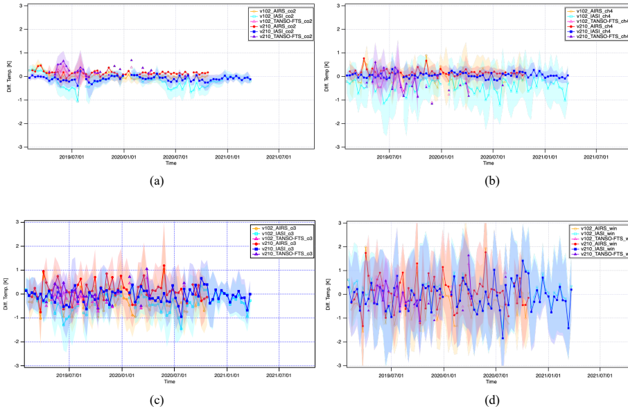
Figure 6: The channel-dependent brightness temperature difference for a ten-day average against atmospheric window temperature for SNO condition between TANSO-FTS-2 and AIRS/IASI/TANSO-FTS. (a) CO 2 spectral range, (b) CH 4 spectral range, (c) O 3 spectral range, (d) atmospheric window channels.
