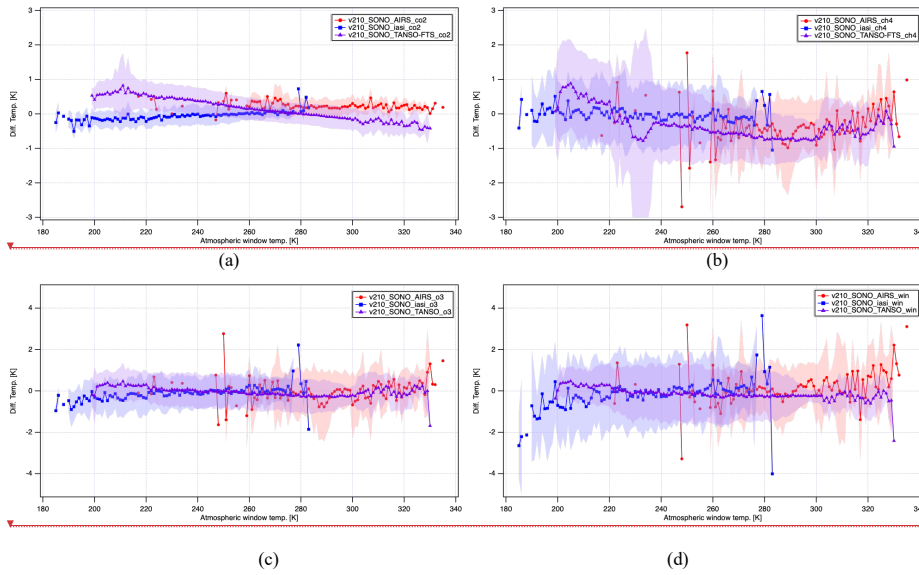
Figure 9: The channel-dependent brightness temperature difference in 1 K bins against window temperature for 20-SONO between TANSO-FTS-2 and AIRS/IASI/TANSO-FTS with the corresponding standard deviation (shaded area). (a) CO 2 spectral range, (b) CH 4 spectral range, (c) O 3 spectral range, (d) atmospheric window channel.
