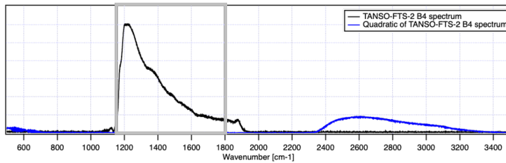
(b) Band 4 of TANSO-FTS-2
