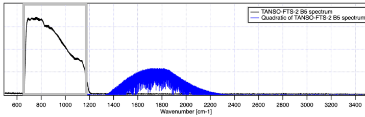
(c) Band 5 of TANSO-FTS-2
