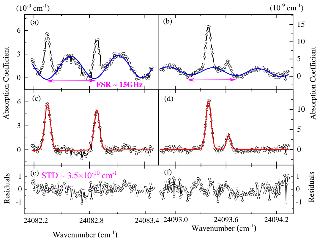
Figure 2. The recorded spectra of \text{H}_2^{16}\text{O} around (a) 24082\text{ cm}^{-1} and (b) 24093\text{ cm}^{-1} . Solid blue lines indicate the simulated fringes with a sine wave function. Spectra after subtraction of the simulated fringes are shown in (c) and (d). The absorption spectra of \text{H}_2\text{O} obtained from a Voigt profile fitting are shown in solid red lines and their fitting residuals were plotted in (e) and (f). The standard deviation of the fitting residuals is about 4 \times 10^{-10}\text{ cm}^{-1} .
