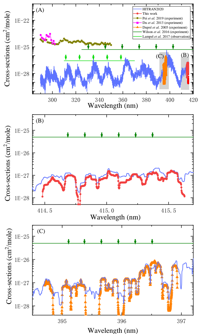
Figure 5. (A) An overview of cross-sections for water vapor obtained in this work and those reported in previous works, including the measurements by (Pei et al., 2019; Du et al., 2013; Dupré et al., 2005) and the upper limits by (Wilson et al., 2016; Lampel et al., 2017), as well as the calculations from (Gordon et al., 2022); (B) Zoomed plots for cross-sections determined in this work at 415 nm, and those simulated from HITRAN2020; (C) Zoomed plots for cross-sections simulated from (Dupré et al., 2005), and those from HITRAN2020. The simulated cross-sections plotted here are convoluted to a spectral resolution of 5 \text{ cm}^{-1} ( \approx 0.05 \text{ nm} ) except that results from (Pei et al., 2019) are given in 1 nm step sizes and (Du et al., 2013) are given in 5 nm step sizes.
