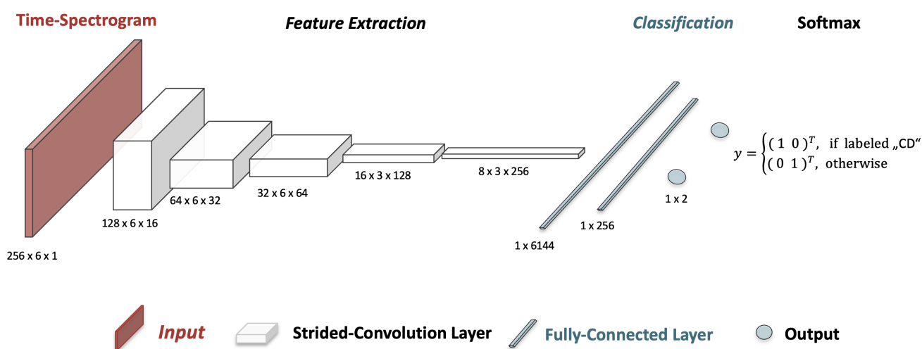
Figure 3. Illustration of the CNN architecture. The time-spectrogram serves as input to the VOODOO model. Five feature extraction layers follow the input layer performing strided-convolution operations. While the number of features which can be extracted increases from 16 to 256, the size of the features maps shrink from 128 by 6 to 8 by 3 pixel. The feature extraction is followed by two fully-connected layers with 8 \cdot 3 \cdot 256 = 6144 and 256 nodes. The output is a vector with two elements, with |y| = 1 .
