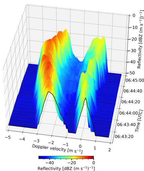
Figure 1. Time-spectrogram from Aug. 1, 2019 at 2400 m altitude in Punta Arenas, Chile. The bi-modal Doppler-spectra contain liquid cloud droplets the right-hand-side of the spectrum (slow moving) and ice crystals on the left side of the spectrum (faster moving). Cloudnet classification result for this particular time-range slice is "ice and supercooled liquid droplets" at -10^{\circ}\text{C} .
