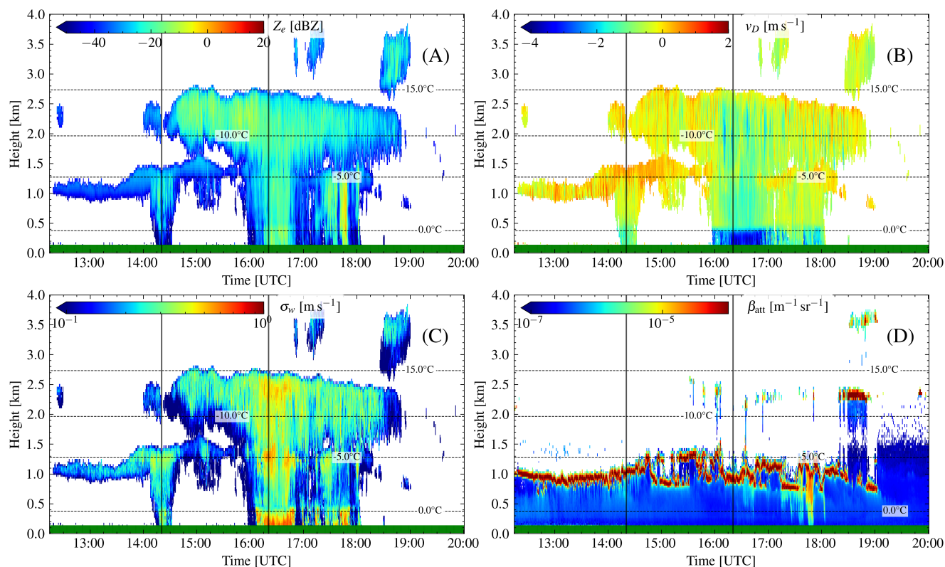
Figure A1. Case study of Dec. 30, 2020 in Leipzig, Germany. (A) radar reflectivity factor Z_e , (B) radar mean Doppler velocity \bar{v}_D , (C) radar spectrum width \sigma_w (D) ceilometer attenuated backscatter \beta_{att} . Dashed lines depict the isotherm lines from ECMWF temperature profiles. The green horizontal line at y -axis= 0 indicates no rain was measured at ground. Solid vertical lines mark locations of the range-spectrograms, shown in Fig.A4.
