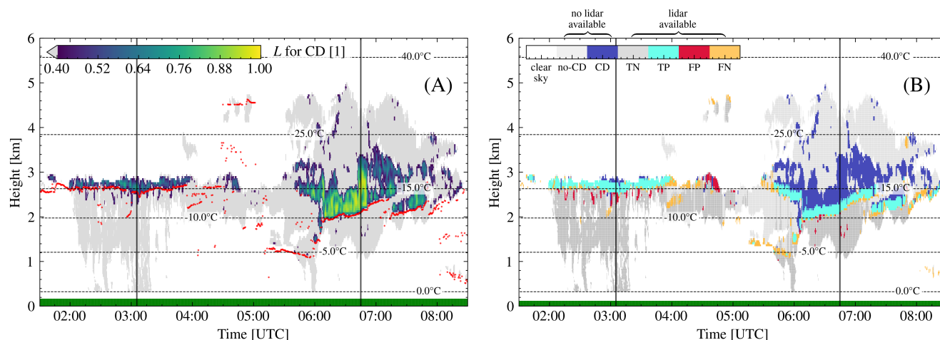
Figure 5. Probability for the presence of cloud droplets for case study of Aug. 1, 2019 in Punta Arenas, Chile. (A) VODOO output: probability for CD, (B) VODOO prediction status. Dashed lines depict the isotherm lines from ECMWF temperature profiles. Red dots in (A) indicate the first ceilometer CBH. The green horizontal line at y -axis=0 indicates no rain was measured at ground. Solid vertical lines mark locations of the range-spectrograms, shown in Fig.7.
