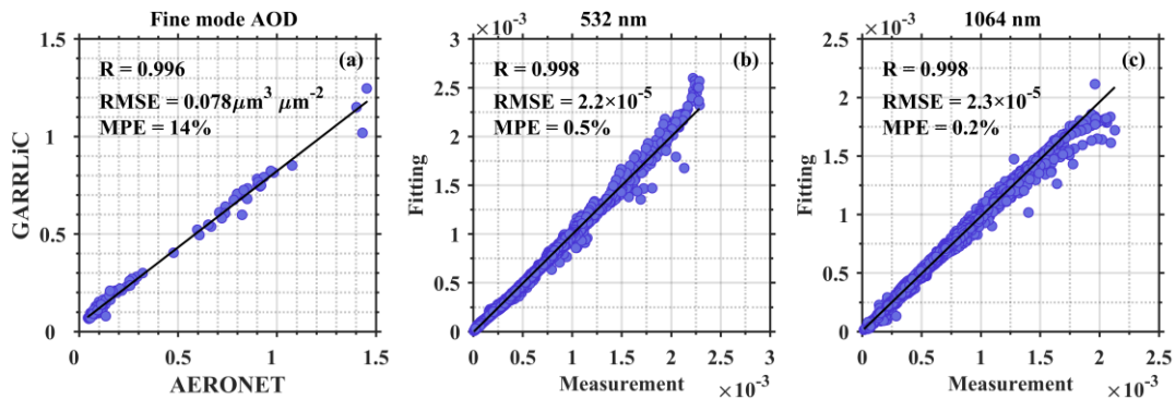
Figure 3. (a) The comparison of fine-fine -mode AOD between GARRLiC and AERONET; The comparison of lidar signal between the fit from GARRLiC and measurement at (b)532 nm and (c) 1064 nm.
