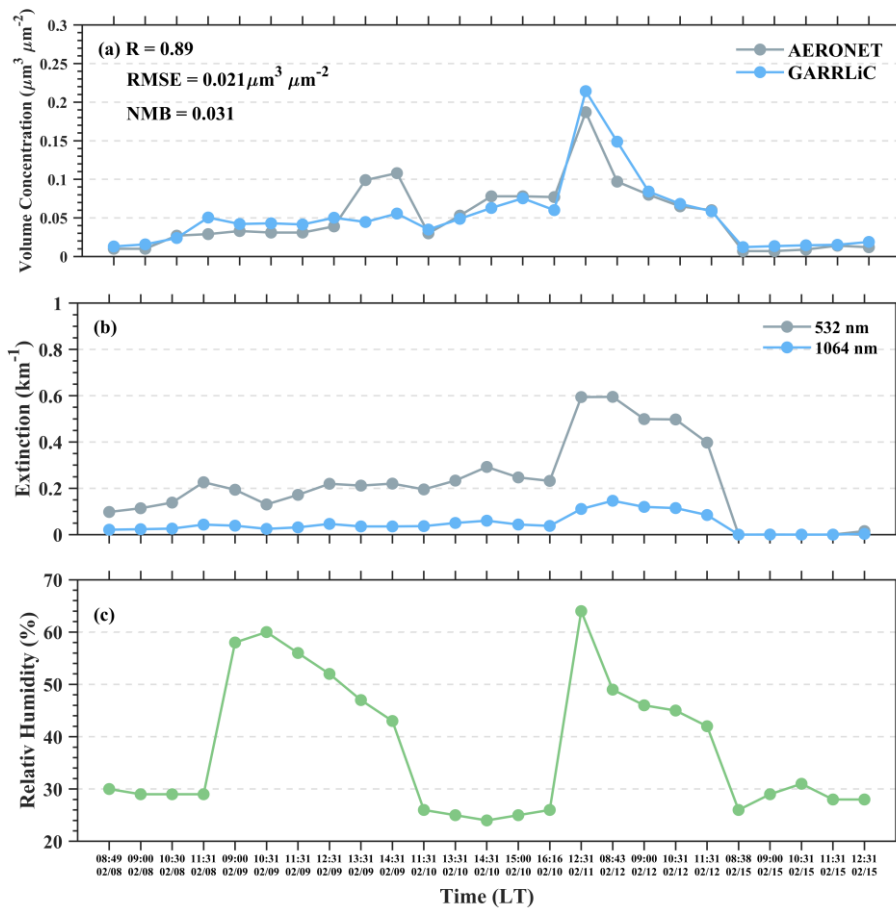
Figure 4. (a) The fine volume concentration from GARRLiC and AERONET; (b) The fine-fine -mode extinction at 532 nm and 1064 nm; (c) The RH from ERA5 at the available time on 8–15 February 2021.
