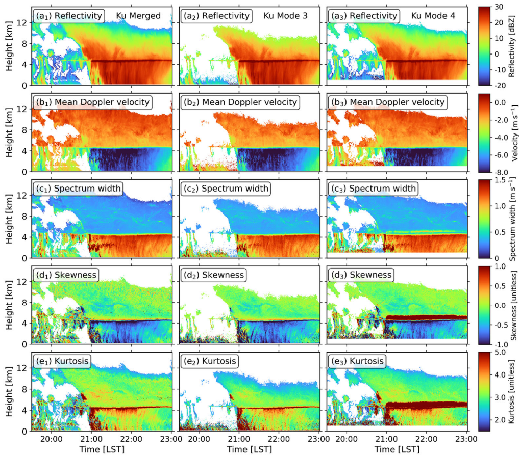
400 Figure 15. Time-height cross-section plots of Ku-band Doppler spectra moments from 19:30:19 to 23:01:26. The left column is estimated from the merged Doppler spectra, and the middle and the right columns are from the data recorded at modes 3 and 4, respectively. From top to bottom: (a) reflectivity; (b) mean Doppler velocity; (c) spectrum width; (d) skewness; (e) kurtosis.
