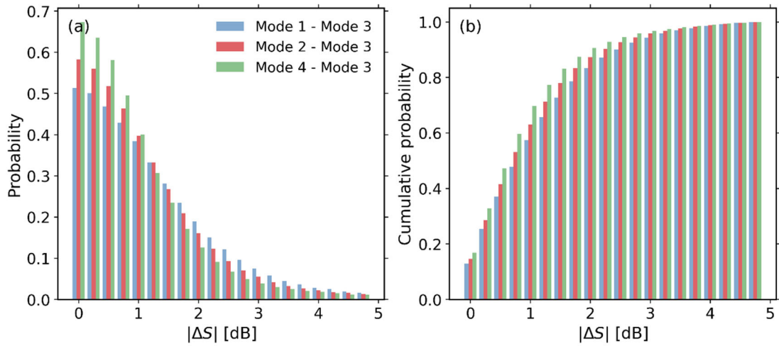
495 Figure A1. (a) Probability density and (b) cumulative distribution of spectral power ratio of meteorological signals between different modes at Ku-band.
