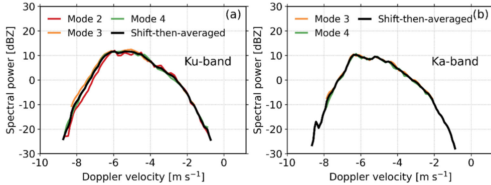
Figure 11. (a) Ku-band Doppler velocity spectra from modes 2, 3, and 4 recorded on 6 June 2020 at 22:52:08 LST at 2.34 km. The merged Doppler spectrum was derived from the Doppler spectra recorded at modes 2, 3, and 4 after shifting and averaging. Note that Ku-band radar observations at mode 1 were not used due to the power loss during coherent integration. (b) The same as in (a) but for Ka-band and observations at modes 3 and 4 were used.
