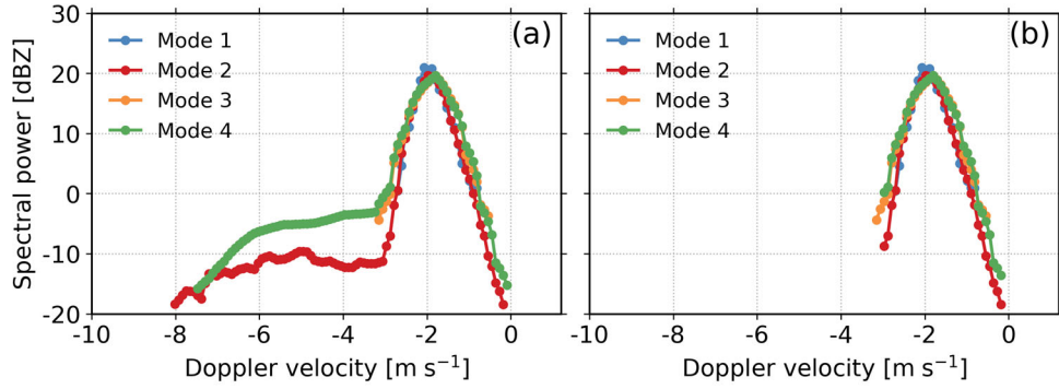
245 Figure 6. Ku-band Doppler power spectra recorded at different modes at 5.01 km on 6 June 2020 at 22:52:08 LST. (a) Noise-removed Doppler spectrum; (b) the same as (a) but after the removal of range sidelobe.
