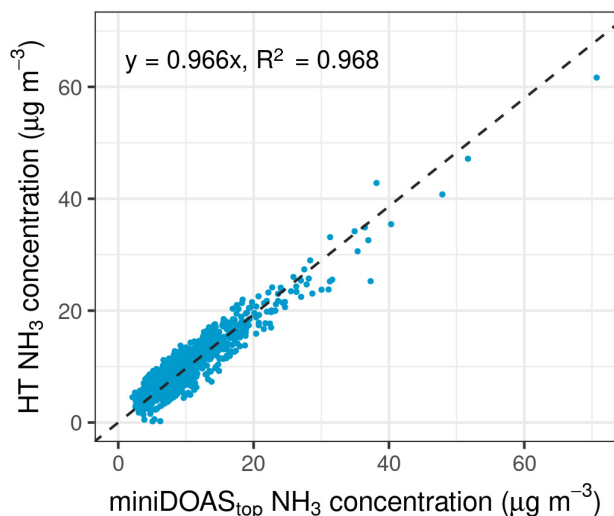
Figure 5 Scatter plot of the \text{NH}_3 concentrations from the miniDOAS top and the temperature corrected HT instrument during parallel measurements (correlation line was forced through the origin).
