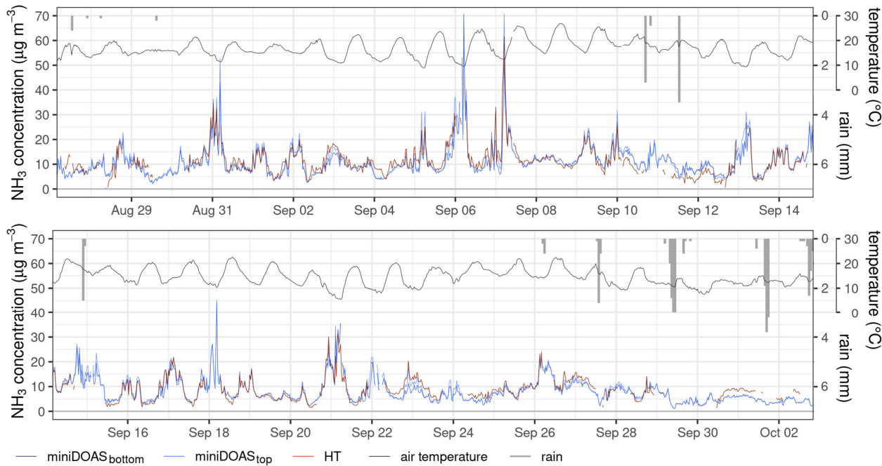
375 Figure 6. Time series of the measured, unfiltered \text{NH}_3 concentrations after temperature correction from the HT (red) and the miniDOAS instruments (dark blue for the bottom one; light blue for the top one) in \mu\text{g m}^{-3} , the hourly ambient temperature (black) in ^\circ\text{C} and the amount of rainfall (grey bars) in mm.
