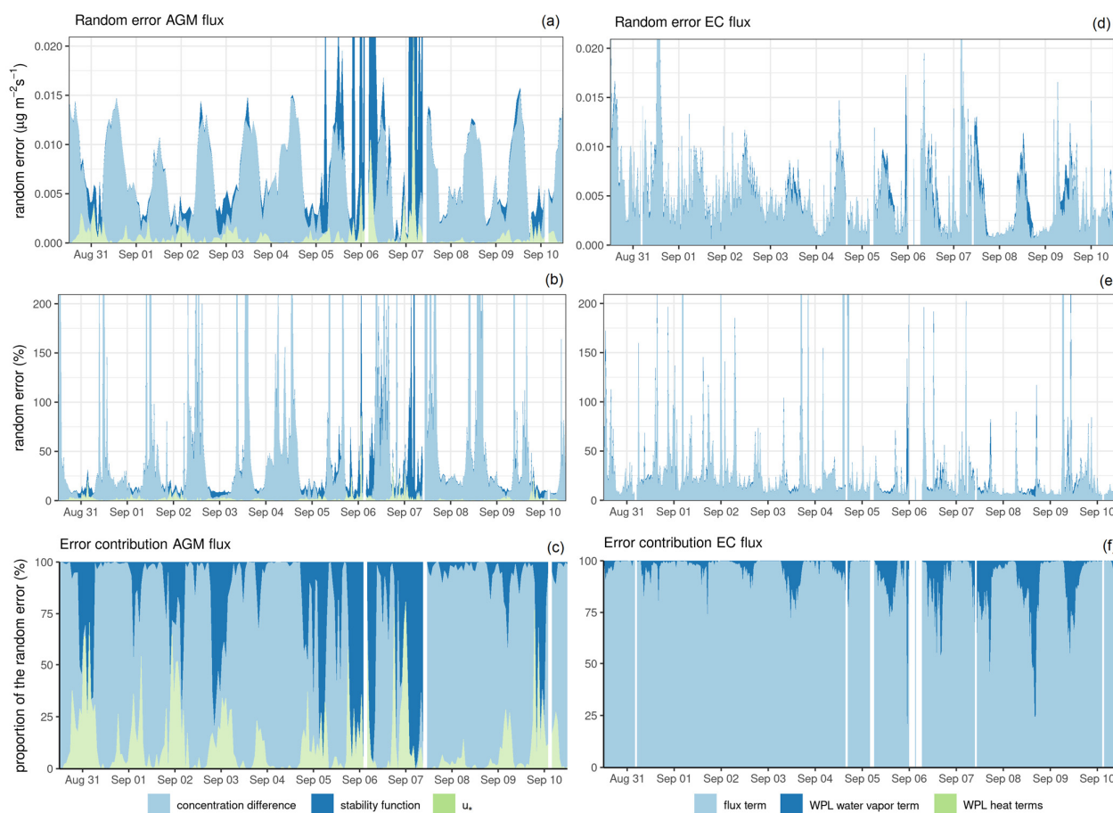
Figure 10. The absolute and relative random errors and the corresponding error contributions (in % of the random error) of the AGM (a, b, c) and EC (d, e, f) NH 3 fluxes from August 31 st to September 10 th . For the EC fluxes, the light blue component (flux term) refers to F1 in Eq. 4, based on fluxes determined using EddyPro, taking into account the damping correction and term A from Eq. 4.
