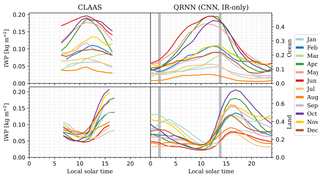
Figure 11. Monthly mean diurnal cycles for 2012 from CLAAS and the CNN, IR-only QRNN retrieval for the areas in Fig. 2. The QRNN expected value is used as the retrieval value. Local solar time (LST) approximated from UTC as LST = UTC + 12 \text{ hours} / 180^\circ \cdot \text{longitude} . The grey areas indicate the LST coverage of the DARDAR profiles in the training set. Note the different vertical axes.
