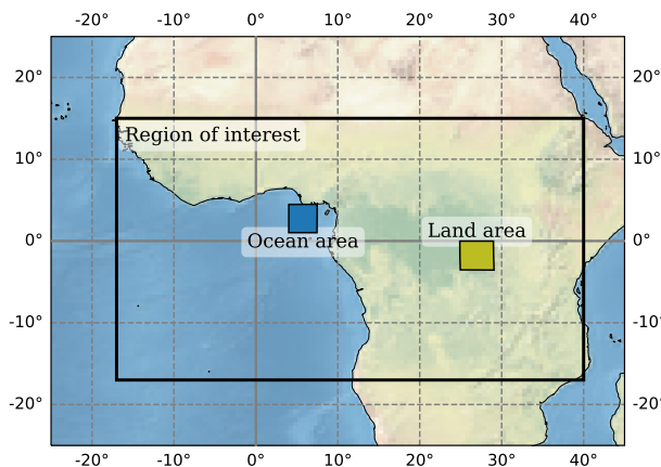
Figure 2. Region of interest used, and ocean and land areas used in the diurnal cycles comparison (Sect. 5.2). Ocean (land) area delimited by [1^\circ, 4.5^\circ] ( [-3.55^\circ, 0^\circ] ) in latitude and [4^\circ, 7.5^\circ] ( [24.95^\circ, 29^\circ] ) in longitude.
