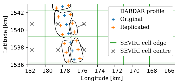
Figure 1. Illustration of the spatial resampling performed. The projection used is the SEVIRI projection. The DARDAR profiles are replicated from the profile in the centre of the track to the swath edges 700 m on each side. The curves enclose the profiles used to derive the averaged values in each cell.
