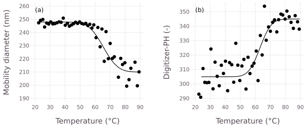
270 Figure 8: The phase transition of bisphere organic particles between 20-90 °C. Black lines correspond to those of a fitted logistic curve. (a) Phase transition of dimers for the nominal 166 nm glucose-sucrose particles versus temperature. The midpoint of the transition is T_{r\pm\sigma} = 65.5\pm 9.8 °C. (b) Temperature scans of Digitizer-PH for the nominal 166 nm glucose-sucrose particles versus temperature. The midpoint of the relaxation is T_{r\pm\sigma} = 63.1\pm 5.9 °C.
