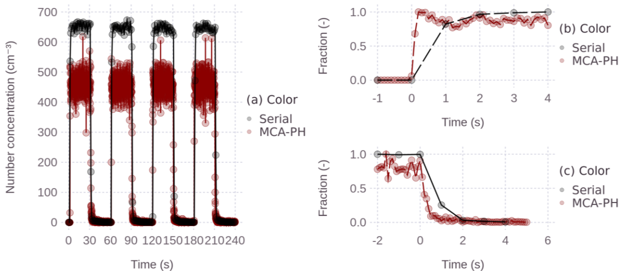
240 Figure 6: Left: time response curves were measured by the POPS data acquisition system and MCA data acquisition system. Right: zoomed-in view for one example up (top) and down (bottom) cycle. Time t = 0 s corresponds to the valve switch.
