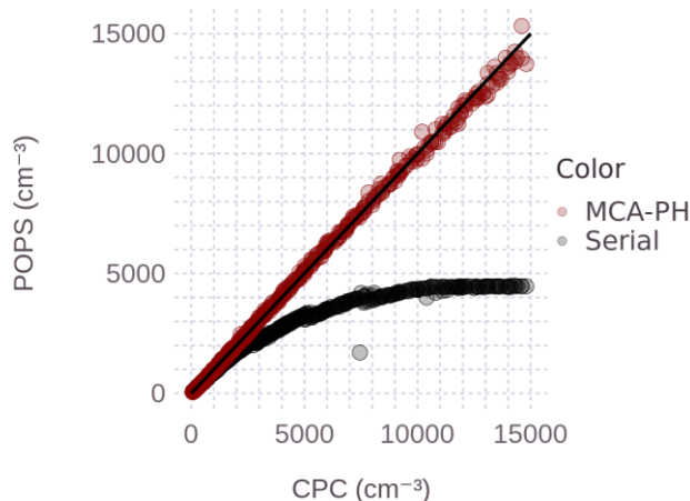
Figure 5: Relationship between CPC number concentration and POPS number concentration derived from the Serial and MCA-PH distributions. The solid black line corresponds to the 1:1 relationship.
