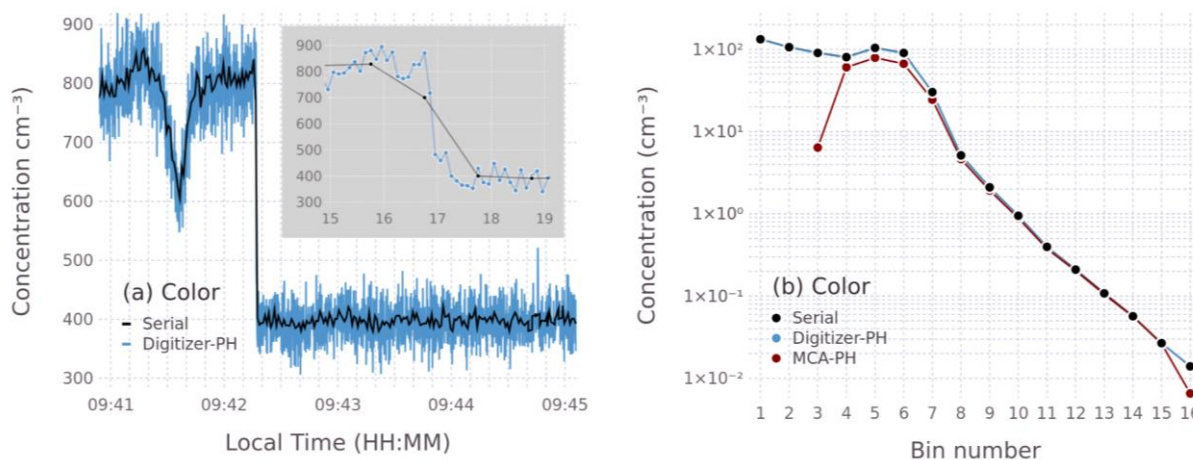
245 Figure 7: (a) Comparison of 1 Hz Serial concentration and 10 Hz Digitizer concentration. The inset is a magnified view corresponding to the transition between 9:42:15 and 9:42:19. (b) Comparison of the Serial distribution, Digitizer-PH distribution, and MCA-PH distributions. Serial and Digitizer-PH distributions are indistinguishable.
