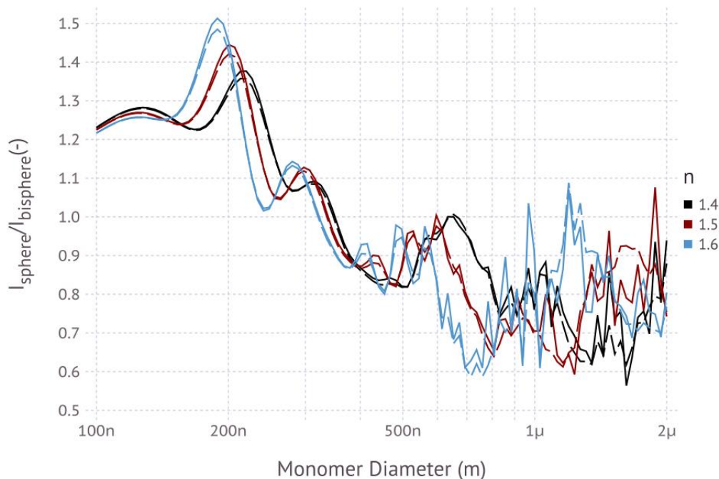
170 Figure 3: The intensity ratio of the uncoalesced bisphere particle and equivalent spherical particle as a function of monomer diameter and refractive index. Each line corresponds to a refractive index m = n + ki , where n is the real and k is the imaginary part. Colors correspond to variations in n . Solid lines correspond to k = 0 and dashed lines correspond k = 0.01 .
