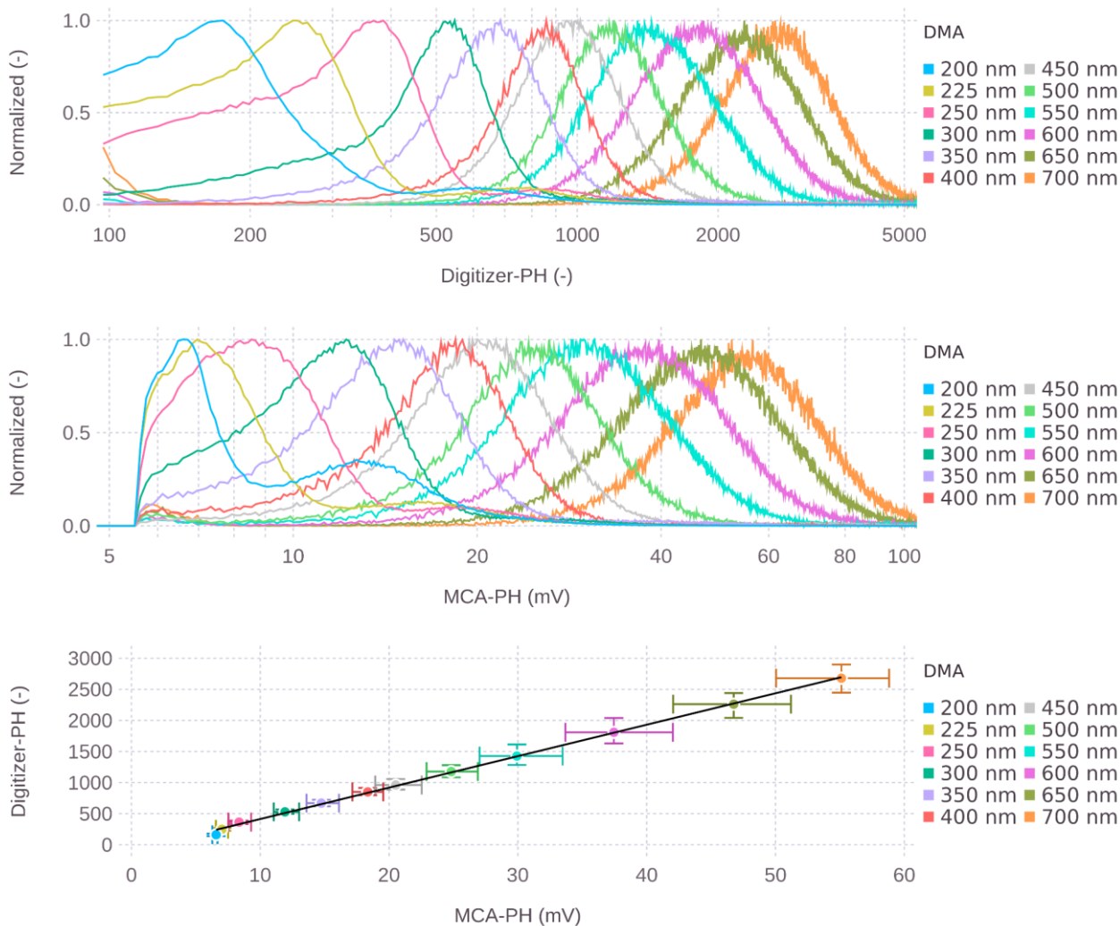
210 Figure 4: Top and middle panels: Digitizer-PH and MCA-PH histograms for dry size selected ammonium sulfate particles between 200 nm and 700 nm. The histograms were normalized such that the largest value equals unity. Bottom panel: comparison of Digitizer-PH and MCA-PH at the peak of the histogram. Error bars correspond to the 95% confidence interval of the mode determined via a curve fit of the data to a lognormal distribution. The line corresponds to linear regression with the equation \text{Digitizer-PH} = \text{MCA-PH} \cdot 50.59 - 92.57 .
