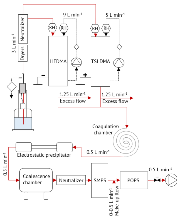
Figure 2: Schematic of the modified POPS instrument integrated into a dual tandem DMA setup. Symbols are as in Fig. 1.
