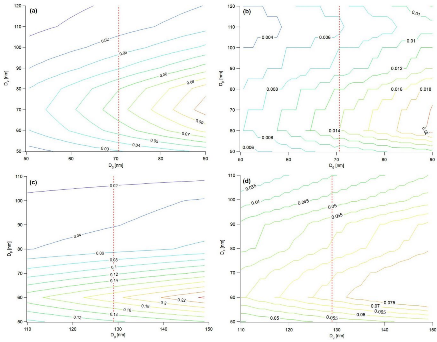
Figure 7: The deviation (Original value – Corrected value) of F_{act} (a) for Case I and (c) for Case II) and \kappa (b) for Case I and (d) for Case II) as function of D_g for log-normally fitted particle size distribution. Contour indicates the range of relative deviation and the value is marked on the contour (The redder the color of the contour, the greater the value). Red dashed line presents the original D_g value for each case ( D_g = 70.6 nm for Case I and D_g = 129.0 nm for Case II).
