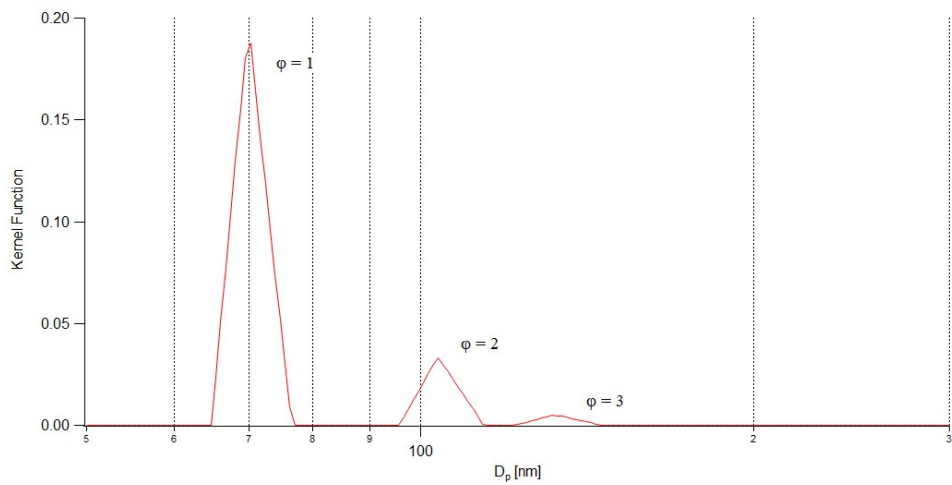
Figure 1: Kernel function for the DMA set size of 70 nm with different charges ( \varphi = 1, 2, 3 ). The sample/sheath flow rate is 1.5/10.
