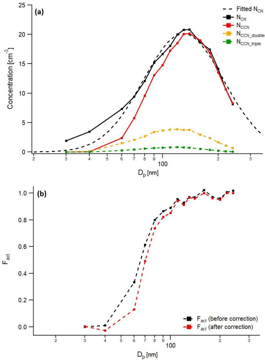
405 Figure 5: (a) Number size distribution of aerosol (black) and CCN (Red for total particle, Orange for doubly charged particle and Green for triply charged particle) and log-normally fitted particle number size distribution ( D_g = 129.0 nm and \sigma_g = 1.65 , black dashed line), and (b) activation curve before (black) and after correction (red) for Case II. Each dot indicates measurement point.
