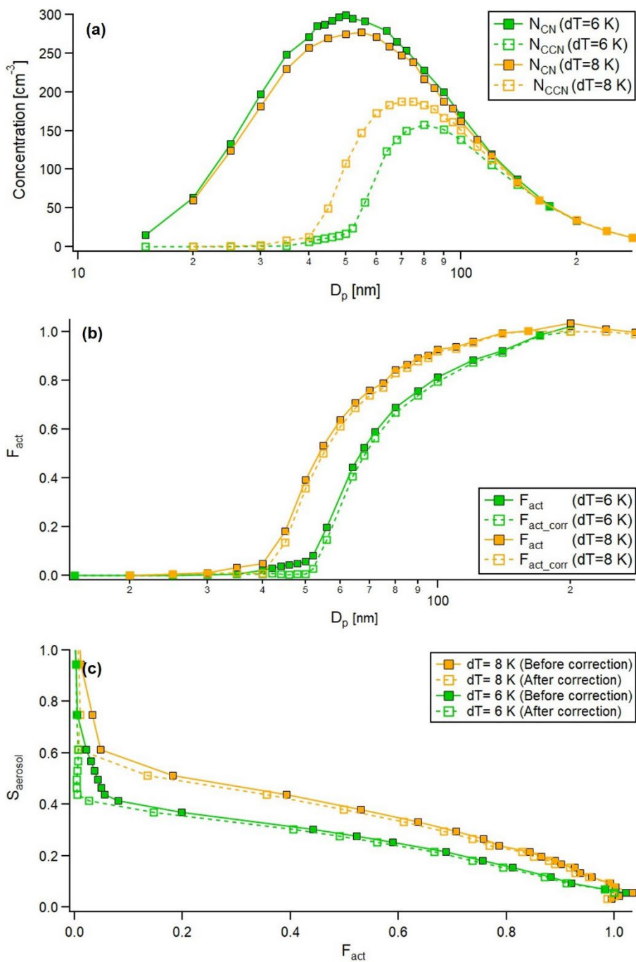
395 Figure 3: (a) Particle and CCN number size distribution (b) activation fraction ( F_{act} ) curve and (c) F_{act} - S_{aerosol} calibration curve for dT = 6 K (green) and 8 K (orange). Squares indicate measurement points. Solid line and dashed line with squares indicate results before and after the correction, respectively.
