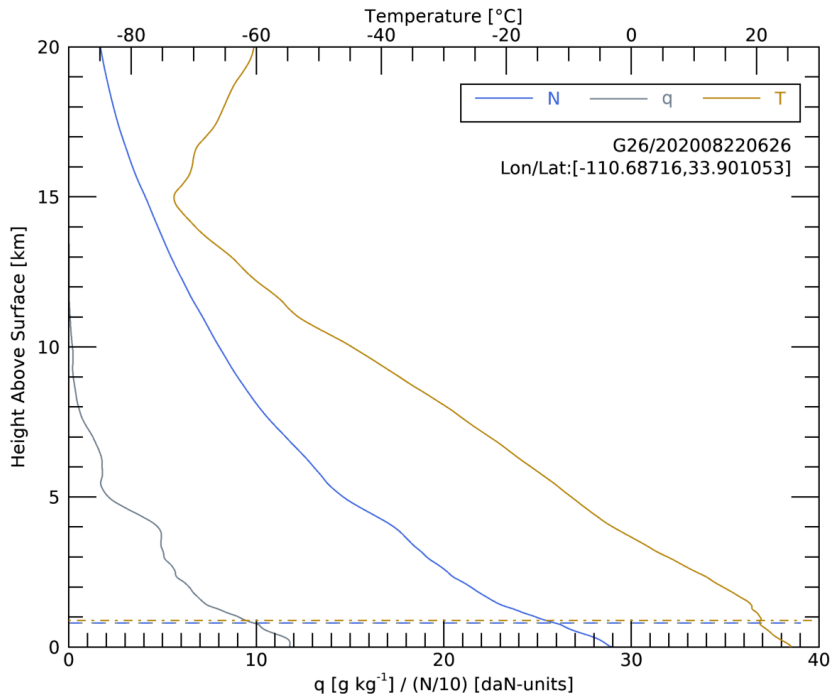
Figure 5. ERA5 vertical profiles of temperature ( T , gold), specific humidity ( q , grey), and refractivity ( N , blue) at 0600 UTC colocated with the World View G26 BRO case on August 22, 2020. Note that for display purposes, one-tenth of the refractivity ( N/10 ) was plotted. In addition, the collocation longitude and latitude of the BRO profile are indicated. Dashed lines indicate the planetary boundary layer height (PBLH) as determined by the gradient method from each variable (see text for details).
