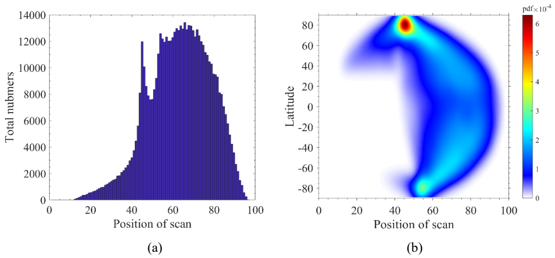
Figure 2. Statistical information of scan angle (a) and latitude (b) of MWHS observations in the collocation dataset.
