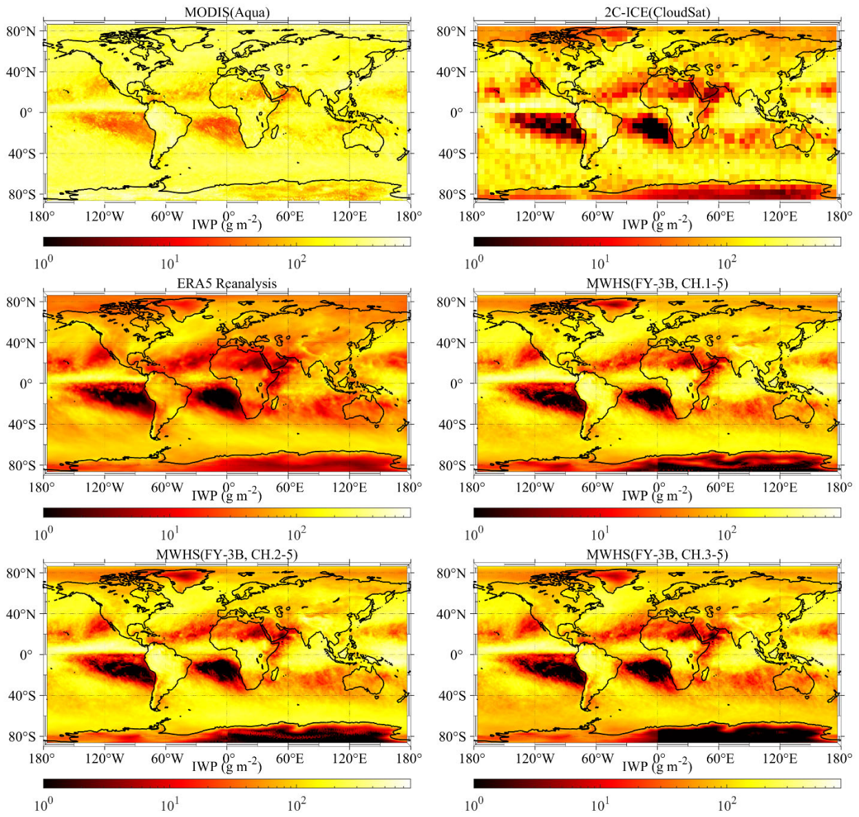
370 Figure 14. Global mean IWP maps for 2015 from MODIS, 2C-ICE, ERA5 and different channel combinations from MWHS. 2C-ICE is gridded on a 5^\circ grid, while the other products are gridded on a 1^\circ grid.
