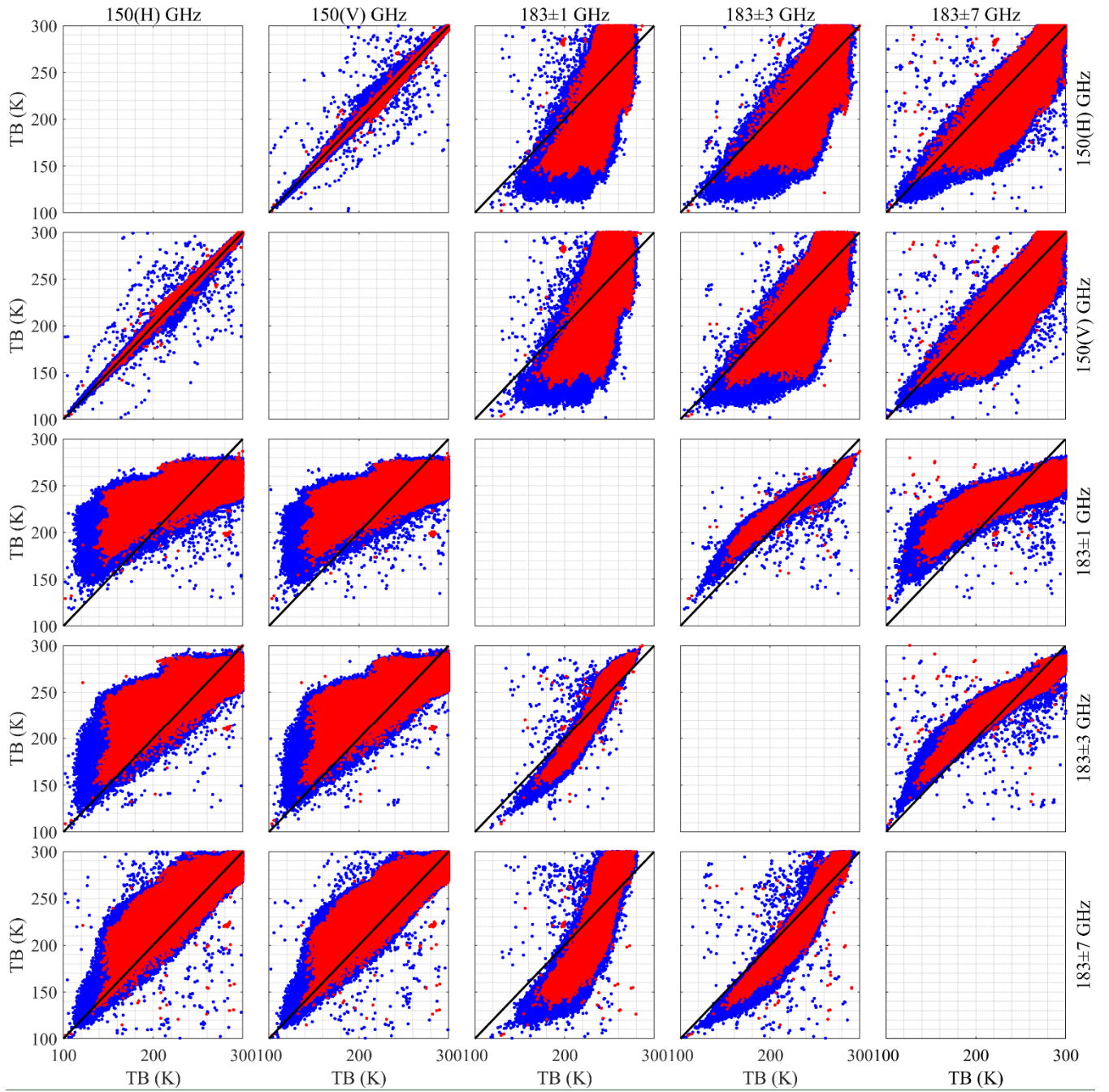
350 Figure 9.13. Measurement comparison from different channels of MWHS dataset in 2015 (blue) and the collocation dataset discussed above (red).
