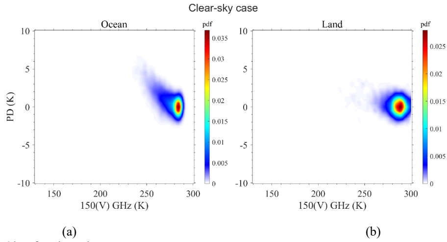
Figure 7. Same as Fig. 6 but for clear-sky scenes.
