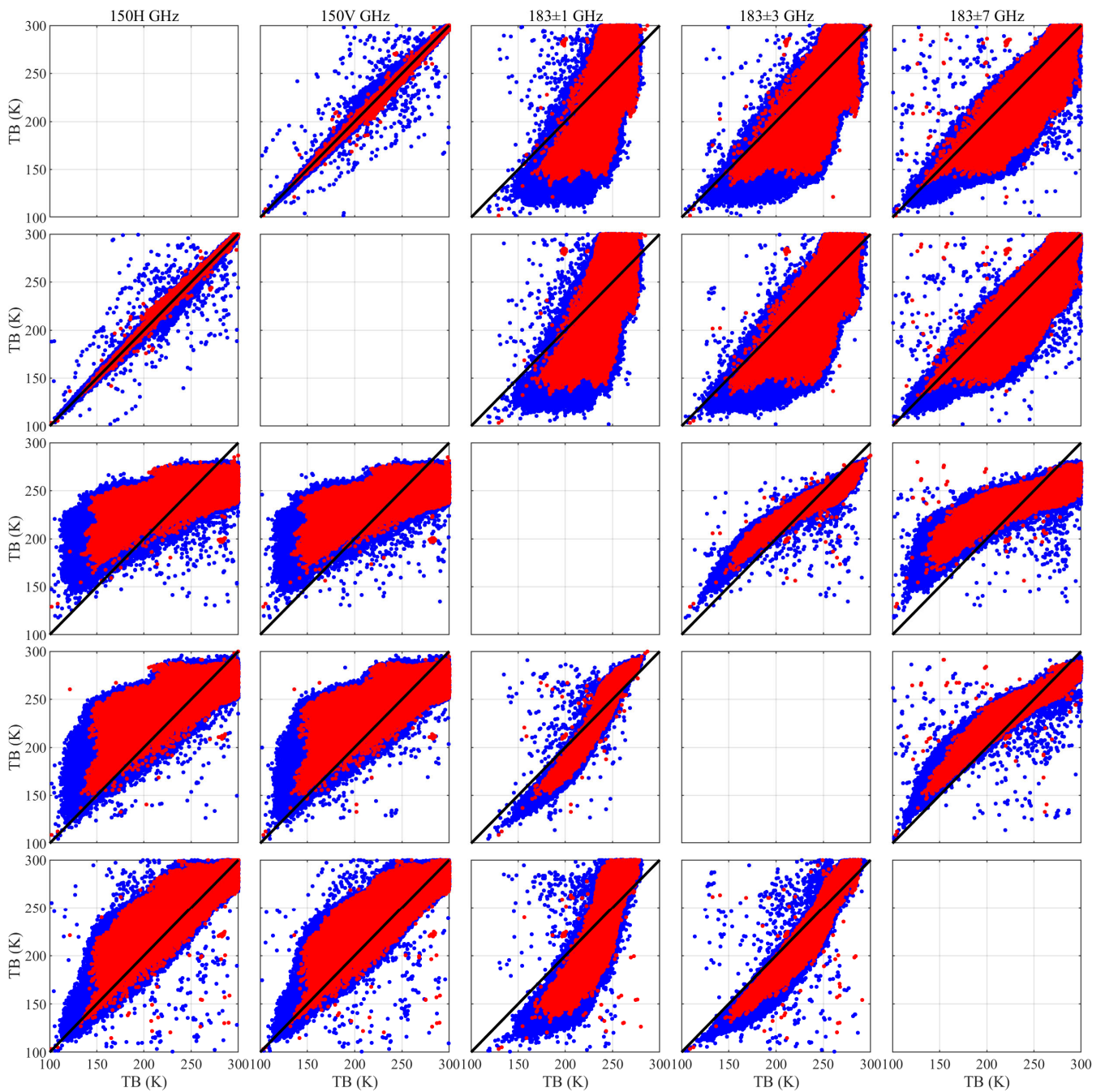
245 Figure 9. Measurement comparison from different channels of MWHS dataset in 2015 (blue) and the collocation dataset discussed above (red).
