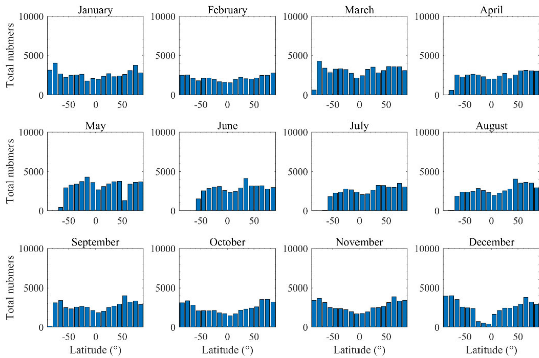
175 Figure 3. MWHS measurement distribution of month and latitude in the collocation dataset.
