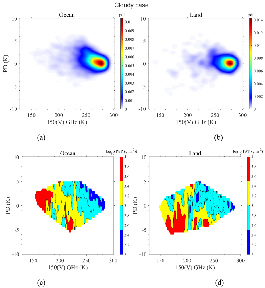
Figure 6. The PD-TB 150V density plots for the collocations in the cloudy scenes over the ocean (a) and land (b). (c) and (d) show the corresponding IWPs from 2C-ICE.
