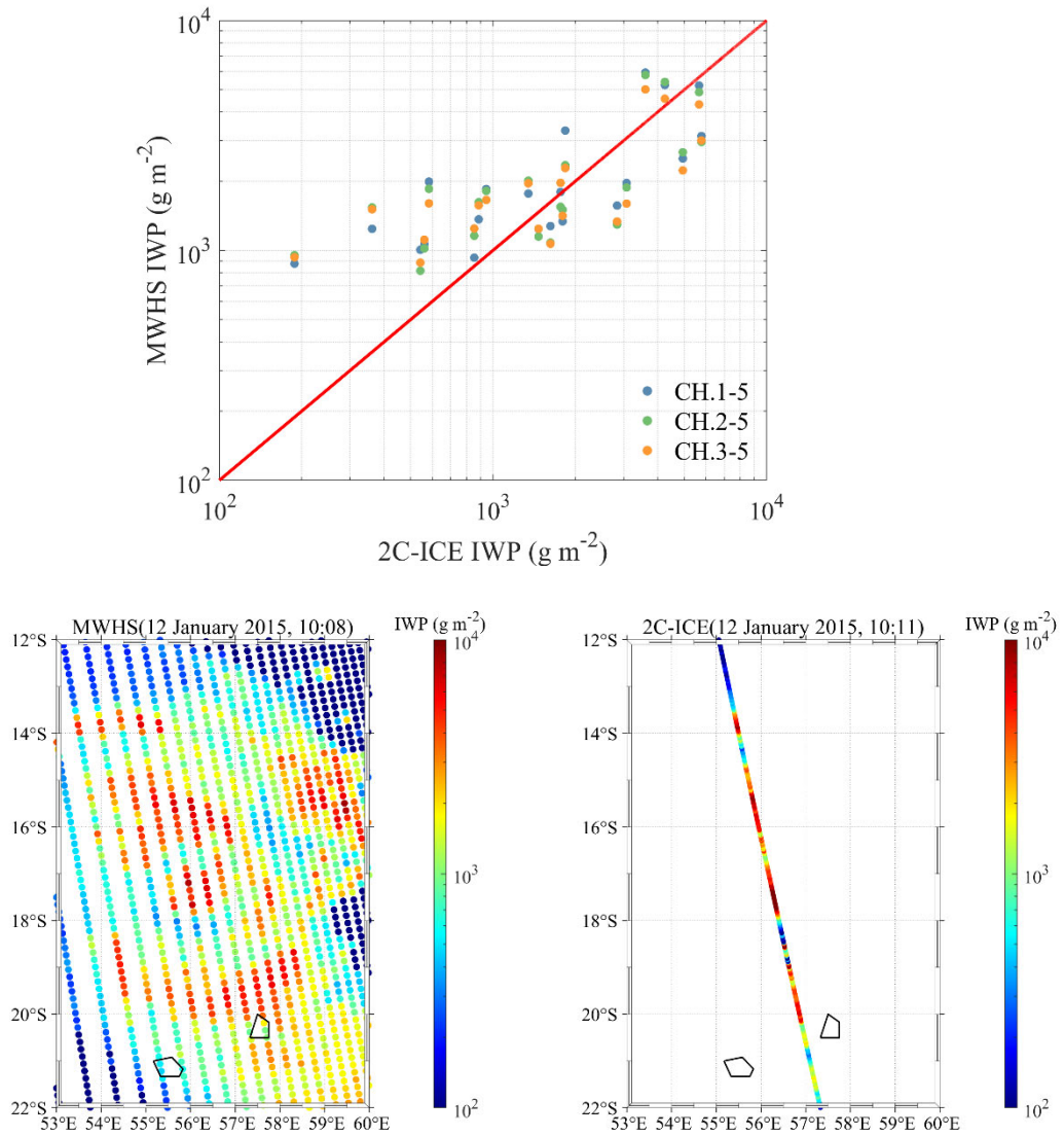
Figure 12. IWP comparison of MWHS and 2C-ICE at the tropical cyclone Bansi.
