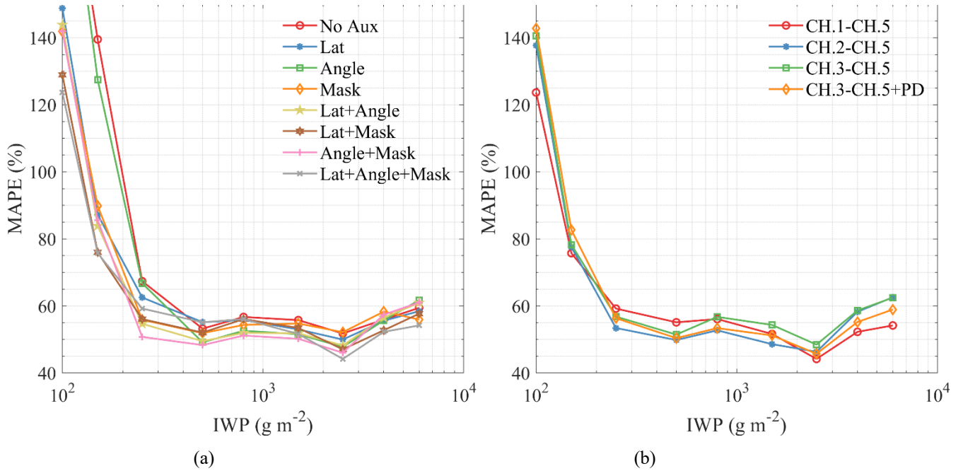
Figure 9. Comparison between the performance of the IWP retrieval networks using different auxiliary and channel combinations of input.
