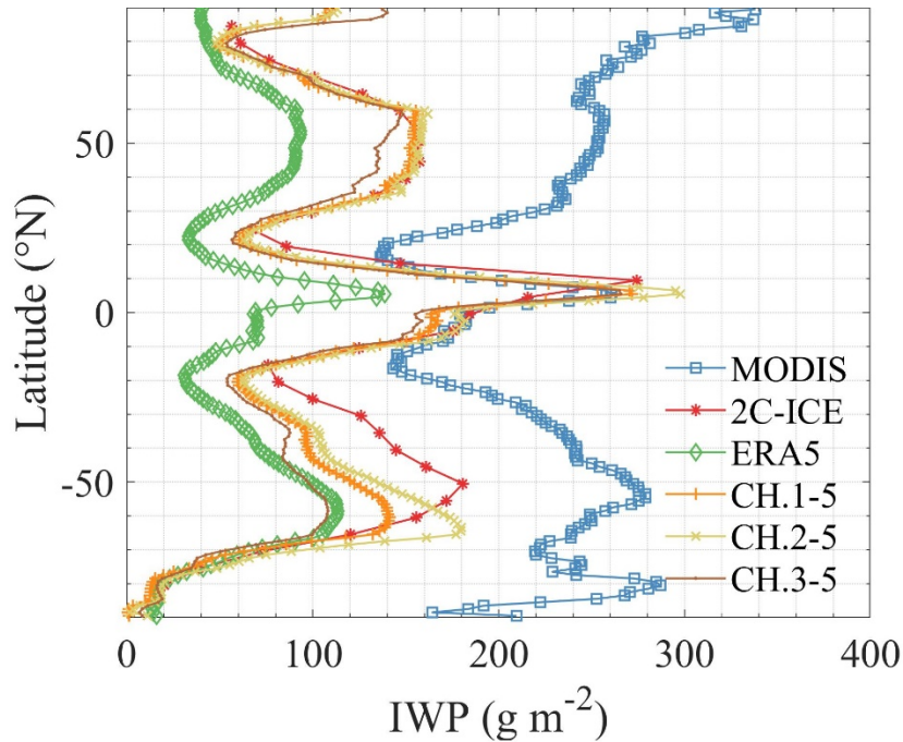
375 Figure 15. Zonal means of IWP for 2015 from MODIS, 2C-ICE, ERA5 and different channel combinations from MWHS. 2C-ICE is gridded on a 5° grid, while the other products are gridded on a 1° grid.
