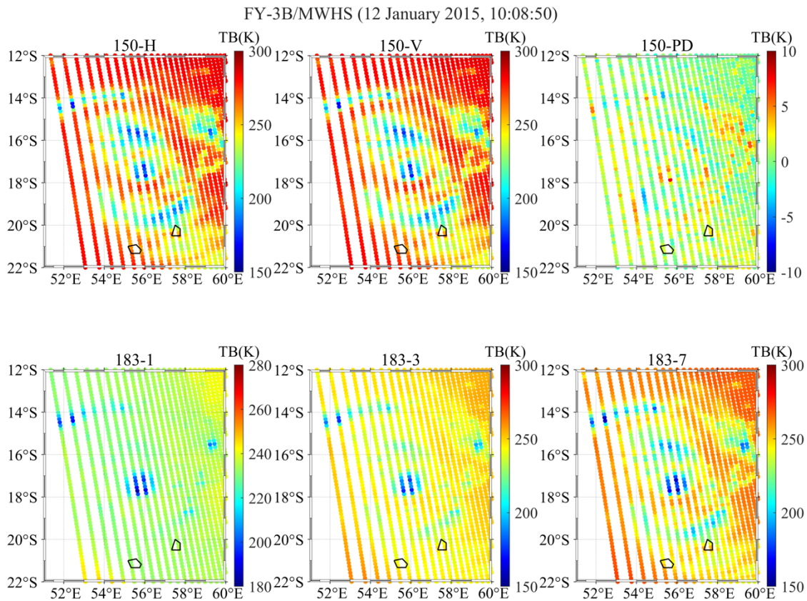
340 Figure 12. Tropical cyclone Bansi on 12 January 2015 as observed with FY-3B/MWHS channels.
