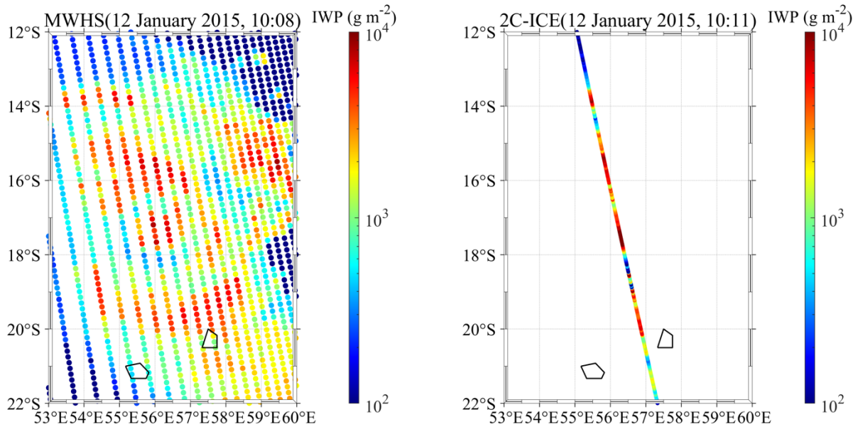
Figure 13. IWP comparison of MWHS and 2C-ICE at the tropical cyclone Bansi.
