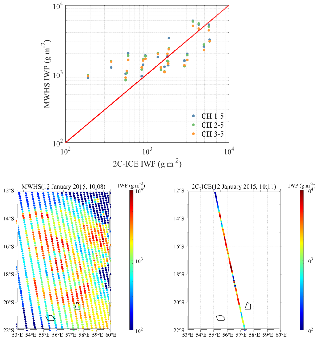
335 Figure 12. IWP comparison of MWHS and 2C-ICE at the tropical cyclone Bansi.
