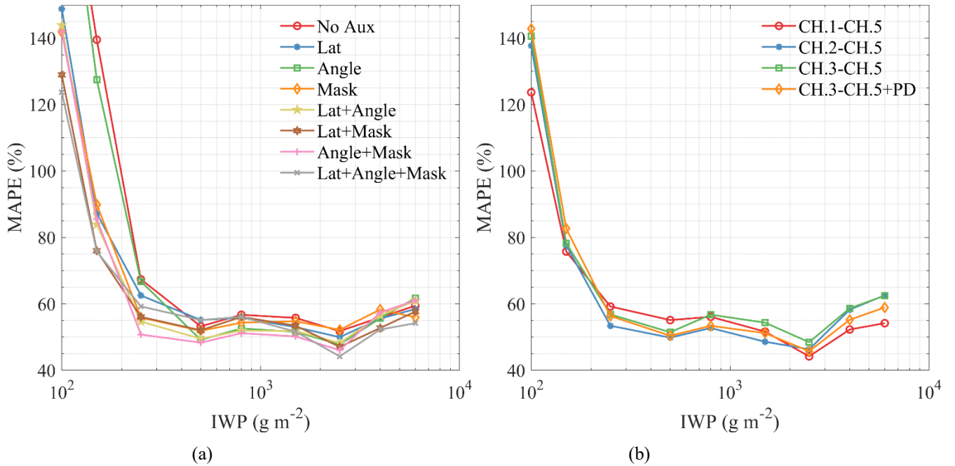
295 Figure 9. Comparison between the performance of the IWP retrieval networks using different auxiliary and channel combinations of input.
