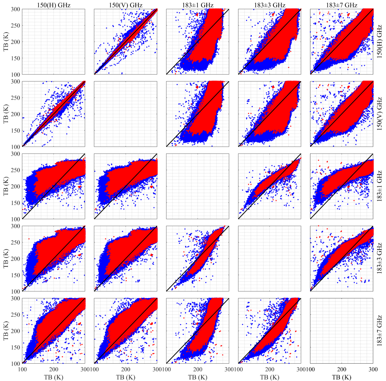
Figure 13. Measurement comparison from different channels of MWS dataset in 2015 (blue) and the collocation dataset discussed above (red).
