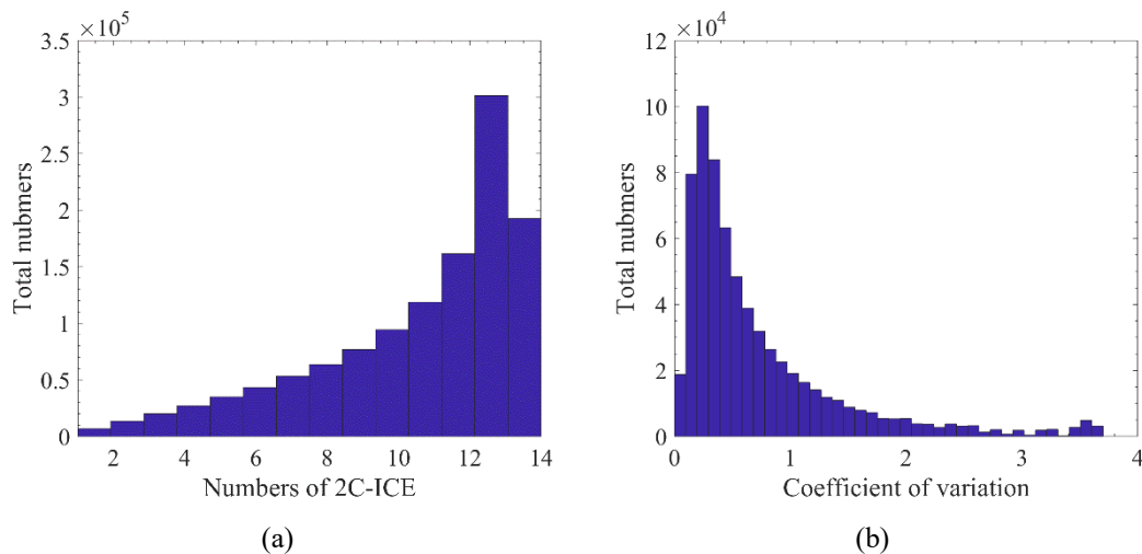
Figure 1. Statistical information of MWHS and 2C-ICE collocations in 2014. (a) Histogram of the number of 2C-ICE pixels within an MWHS pixel. (b) Histogram of the coefficient of variation of the collocations.
