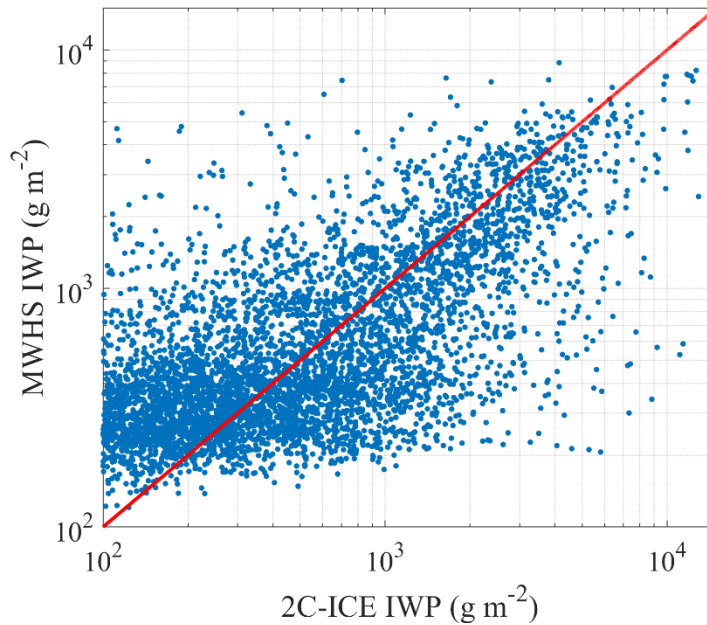
310 Figure 10. Comparison between 2C-ICE and MWHS IWP. The red line represents the diagonal 1:1 line. Clear-sky scenes are not shown.
