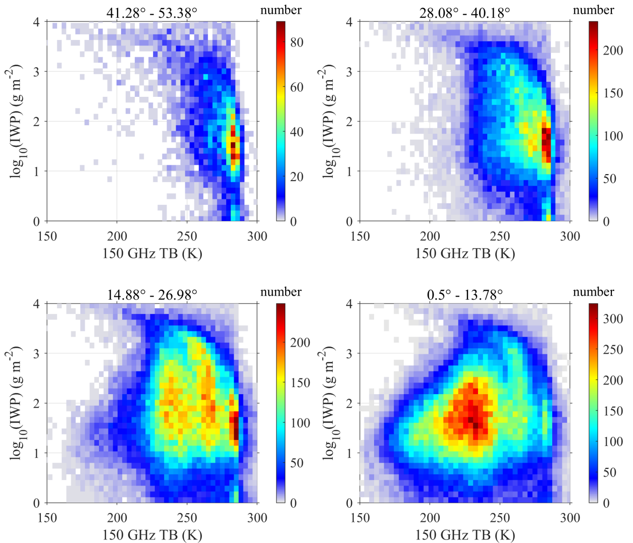
Figure 5. Statistical information of IWP and 150 (V) GHz TB for different scan angles.
