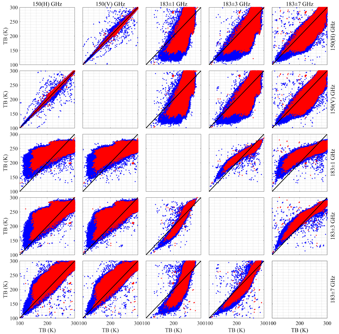
345 Figure 13. Measurement comparison from different channels of MWHS dataset in 2015 (blue) and the collocation dataset discussed above (red).
