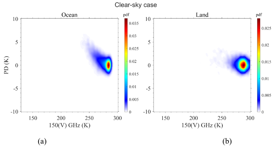
210 Figure 7. Same as Fig. 6 but for clear-sky scenes.
