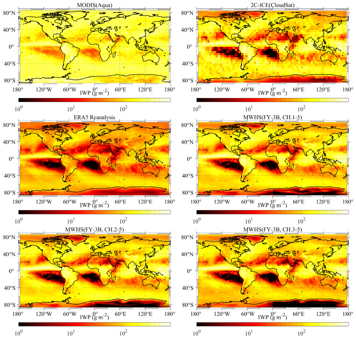
Figure 14. Global mean IWP maps for 2015 from MODIS, 2C-ICE, ERA5 and different channel combinations from MWHS. 2C-ICE is gridded on a 5° grid, while the other products are gridded on a 1° grid.
