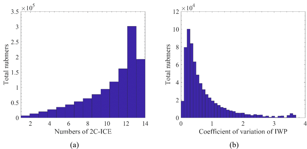
160 Figure 1. Statistical information of MWHS and 2C-ICE collocations in 2014. (a) Histogram of the number of 2C-ICE pixels within an MWHS pixel. (b) Histogram of the coefficient of variation of IWP in collocations.
