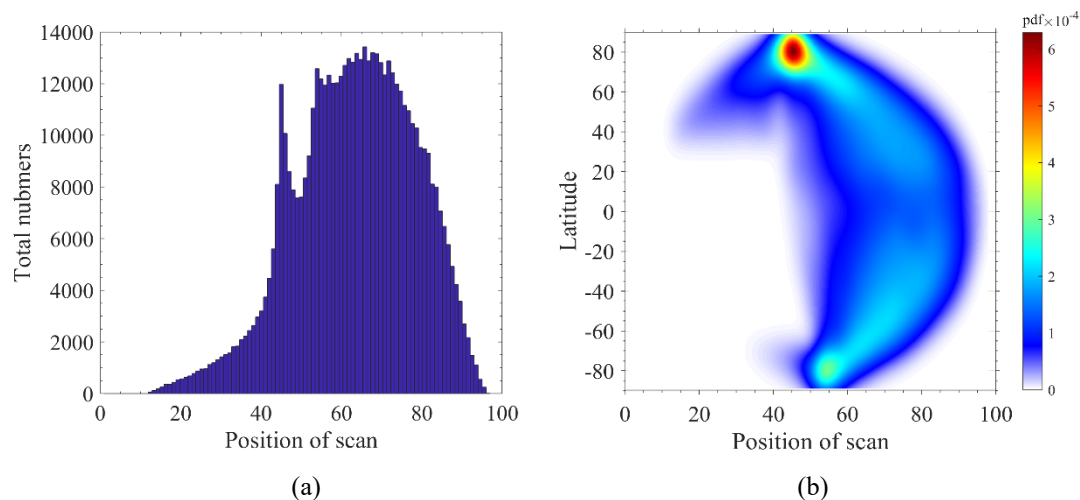
Figure 2. Statistical information of scan angle (a) and latitude (b) of MWS observations in the collocation dataset.
