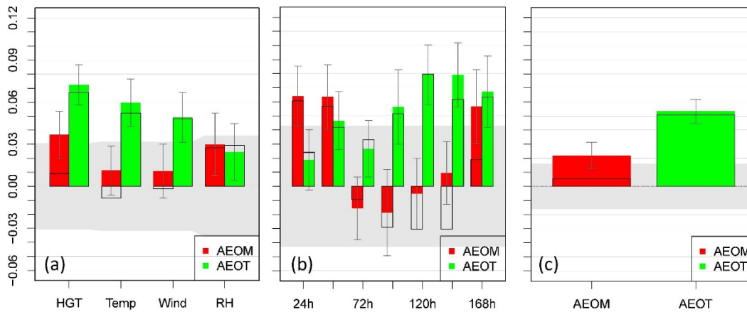
569 Figure 16. The Summary Assessment Metric (SAM) overall forecast scores for AEOM, and 570 AEOT versus BASE experiments in the North America (NA) region. The scores are shown for 571 (a) forecast parameters of temperature (Temp), geopotential height (HGT), vector-wind (Wind) 572 and relative humidity (RH), (b) lead times, and (c) overall performance of AEOM and AEOT. 573 The forecasts are verified to their self-analyses. Values above 0.0 demonstrate an increase in the 574 mean of the normalized distribution and improvement of the forecast versus the BASE, while the 575 shaded region represents the 95% significance level. The grey areas indicate the 95% confidence 576 level under the null hypothesis that there is no difference between experiments for this metric. In 577 addition, the estimated uncertainty at the 95% level is indicated by small error bars at the ends of 578 the color bars. Two normalizations are used, the ECDF (colors) and rescaled-minmax 579 normalization (black outline). Details in Hoffman et al. (2018). A value of 0.02, for example, 580 indicates the average normalized statistic over all statistics is better (greater) by 0.02 than BASE. 581 Under the null hypothesis that there are no differences, all SAMs would be 1/2, so a 0.02 582 improvement can be considered a 4% improvement ( 0.02/0.5 ) in normalized scores.
