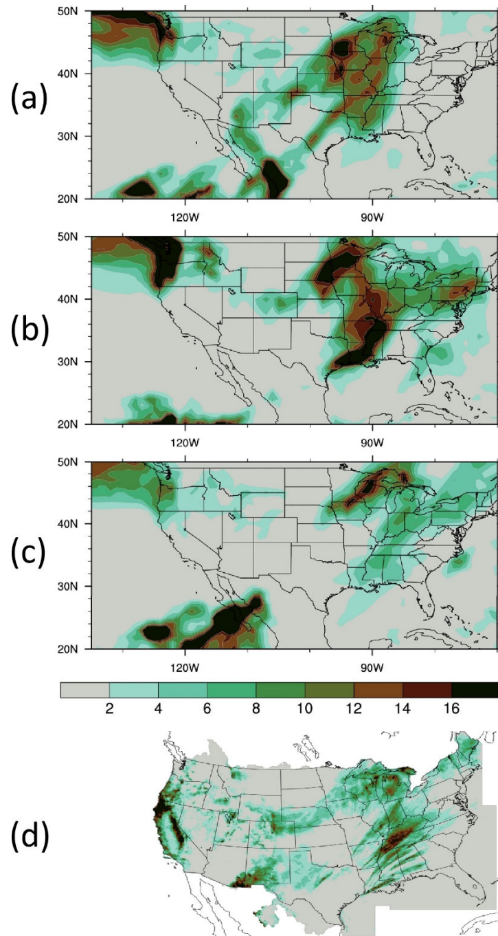
589 Figure 18, The 24-h accumulated precipitation (mm) for 156 h to 180 h, averaged for the 590 forecasts validated from 1200 UTC 26 to 28 November 2019 for (a) BASE, (b) AEOM, (c) 591 AEOT, and (d) the NCEP precipitation raingauge data analysis.
