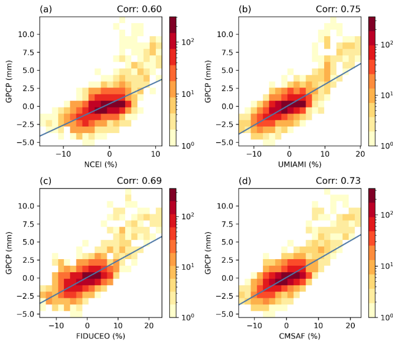
Figure 7: Histograms of UTH anomalies of the four datasets vs. anomalies of GPCP precipitation during the peak six months of the 2015-16 El Niño. The blue line represents the linear regression line. The correlations between UTH anomalies and GPCP precipitation anomalies are labelled at the top of the panels.
