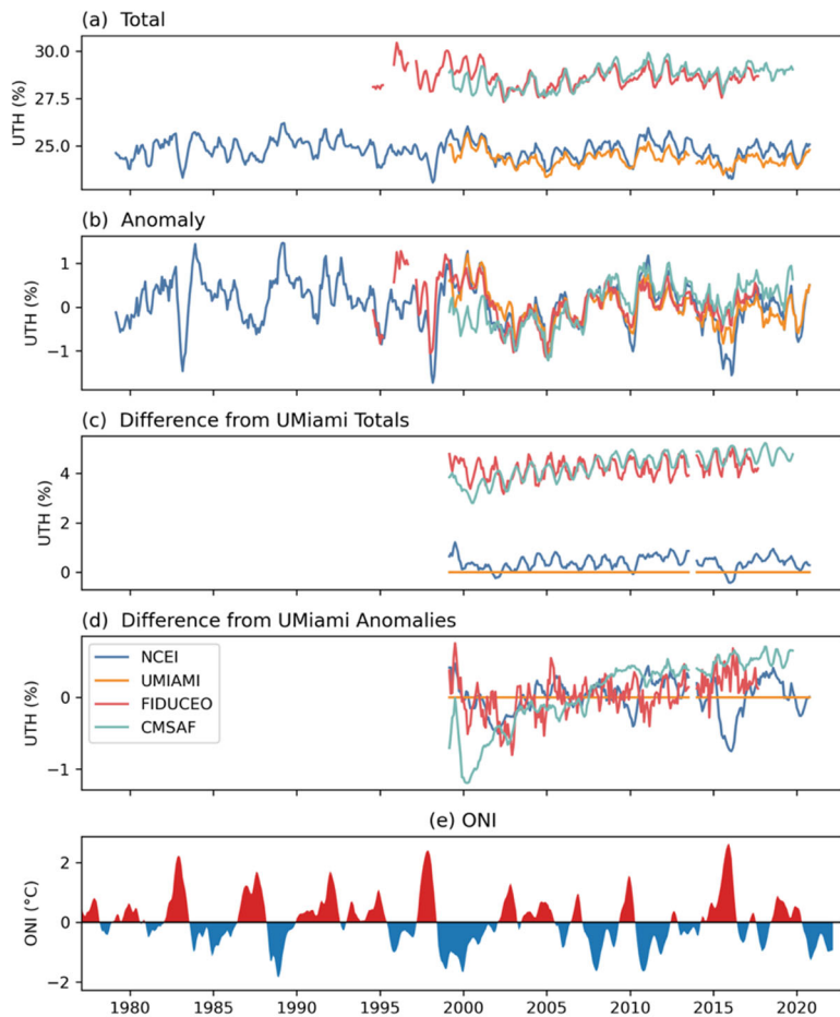
Figure 1: Time series of UTH (%) averaged over 20°S–20°N for (a) the averaged values of UTH, (b) the corresponding anomalies relative to the 2000–2015 climatology, (c) the differences of UTH values relative to the values of UMIAMI, and (d) the differences of anomaly values relative to those of UMIAMI. A five-month moving average is applied to the UTH time series to reduce short-term fluctuations. Panel (e) shows the time series of ONI.
