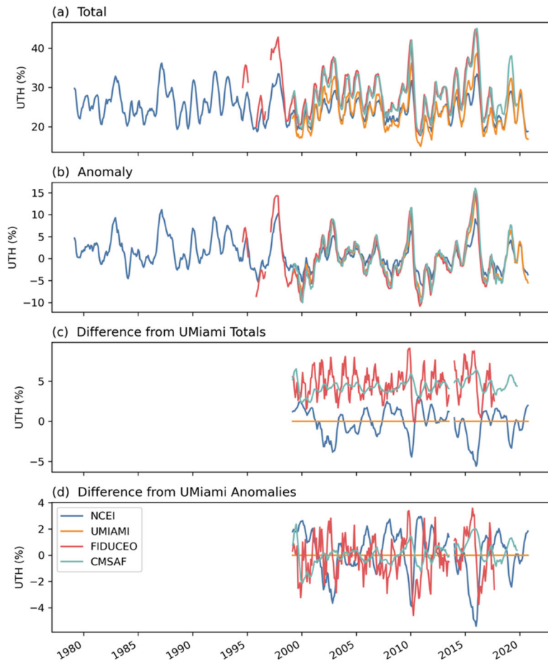
Figure 2: Time series of UTH (%) averaged over the Niño 4 region for (a) the averaged values of UTH, (b) the corresponding anomalies relative to the 2000-2015 climatology, (c) the differences of UTH values relative to the values of UMIAMI, and (d) the differences of anomaly values relative to those of UMIAMI. A five-month moving average is applied to the UTH time series to reduce short-term fluctuations.
