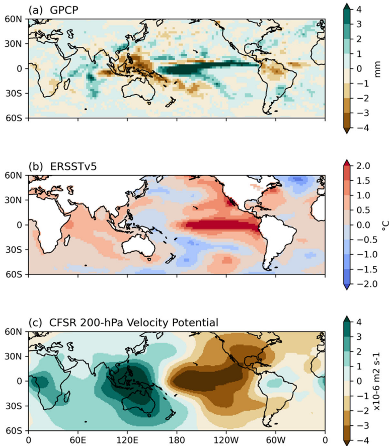
330 Figure 56: Anomalies of GPCP precipitation, ERSSTv5 SST, and CFSR 200-hPa velocity potential during the peak six months of the 2015-16 El Niño event. The box shows the Niño 4 domain in the central Pacific (5°S–5°N, 160°E–150°W).
