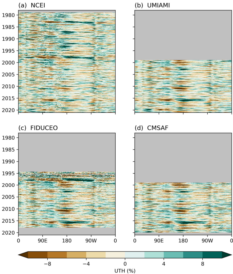
265 Figure 3: Time versus longitude section of UTH monthly anomaly. The analysis is based on an average of data between 5°N and 5°S.
