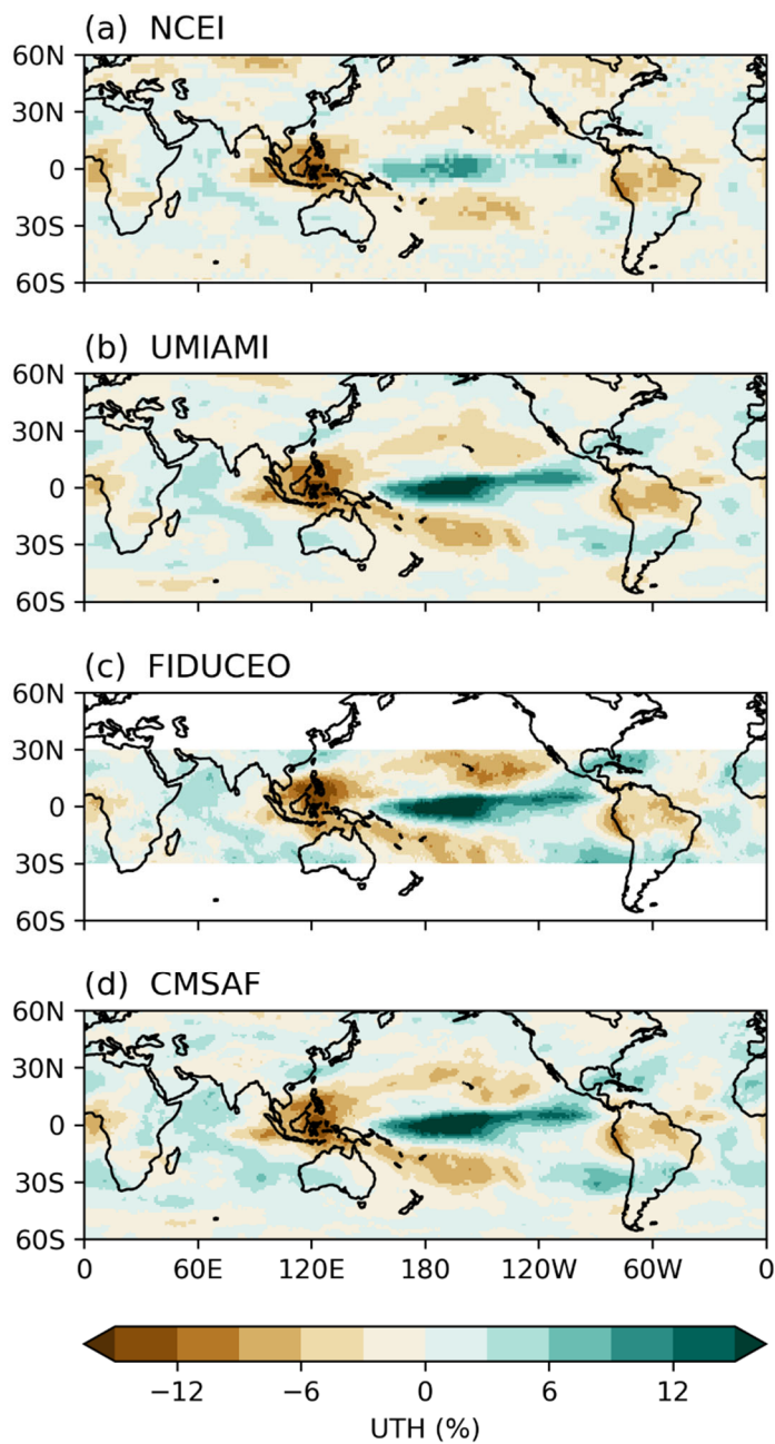
325 Figure 45: Anomalies of UTH during the peak six months of the 2015-16 El Niño event. The box shows the Niño 4 domain in the central Pacific (5°S–5°N, 160°E–150°W).
