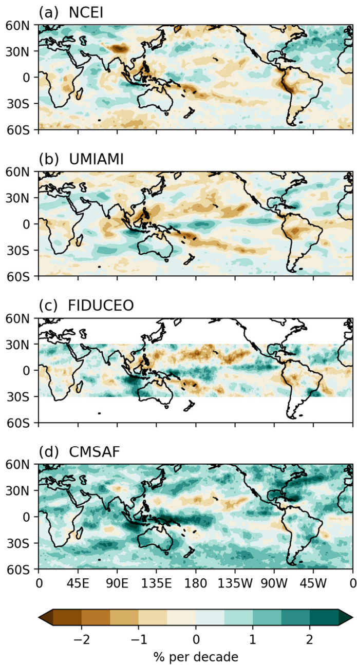
395 Figure 812: Change rates of the four UTH datasets during the common period 1999 to 2017.
