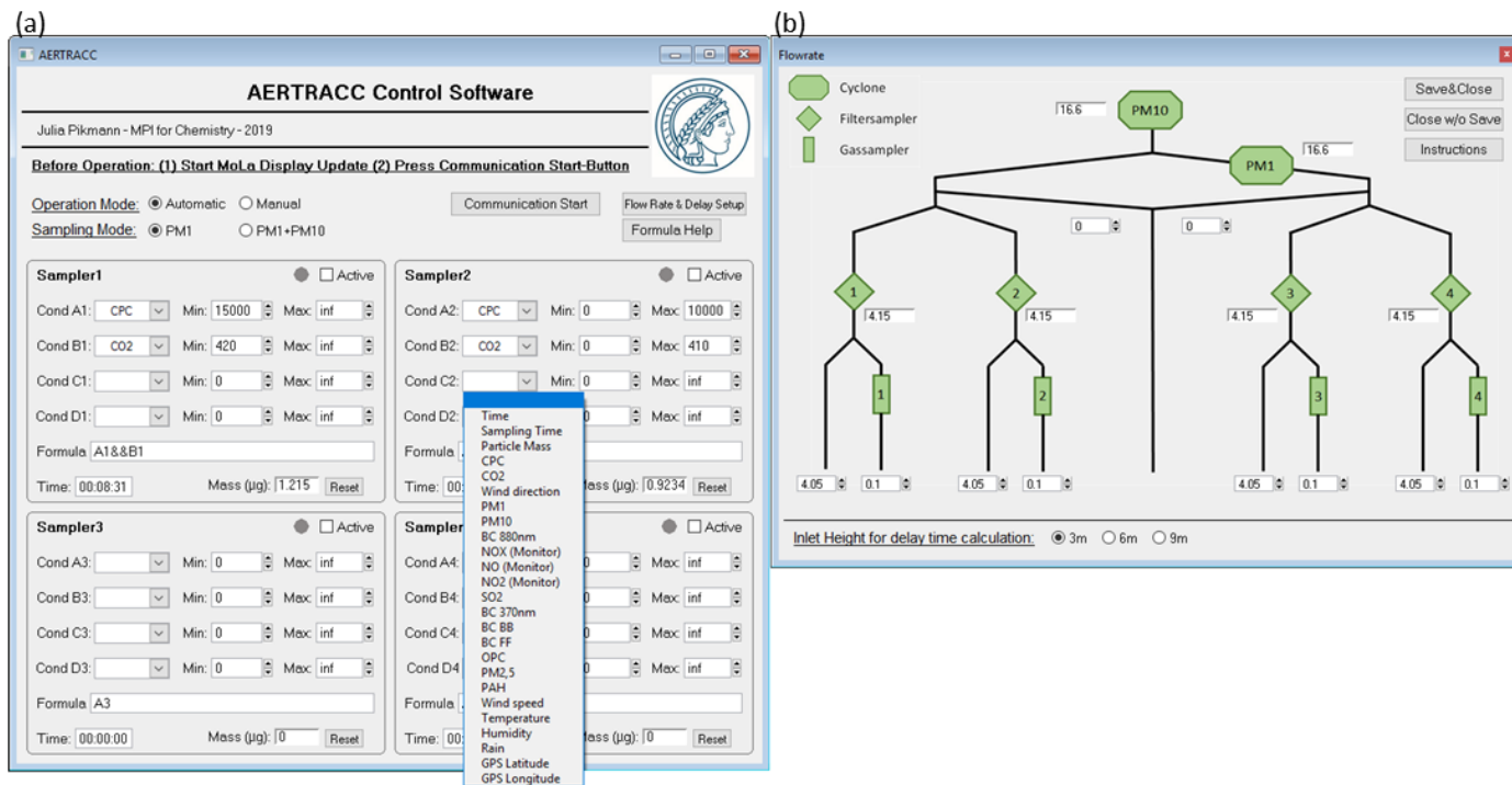
240 240 Figure 2: User interface of the AERTRACC software with main window (a) and flowrate sub-window (b).
