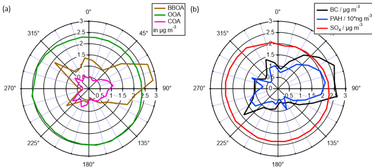
405 Figure 3: Concentrations of the organic aerosol types (a) as well as BC, PAH and SO 4 (b) dependent on local wind direction averaged over 15° sectors. The Pizza oven was located in the direction of 70° relative to MoLa.
