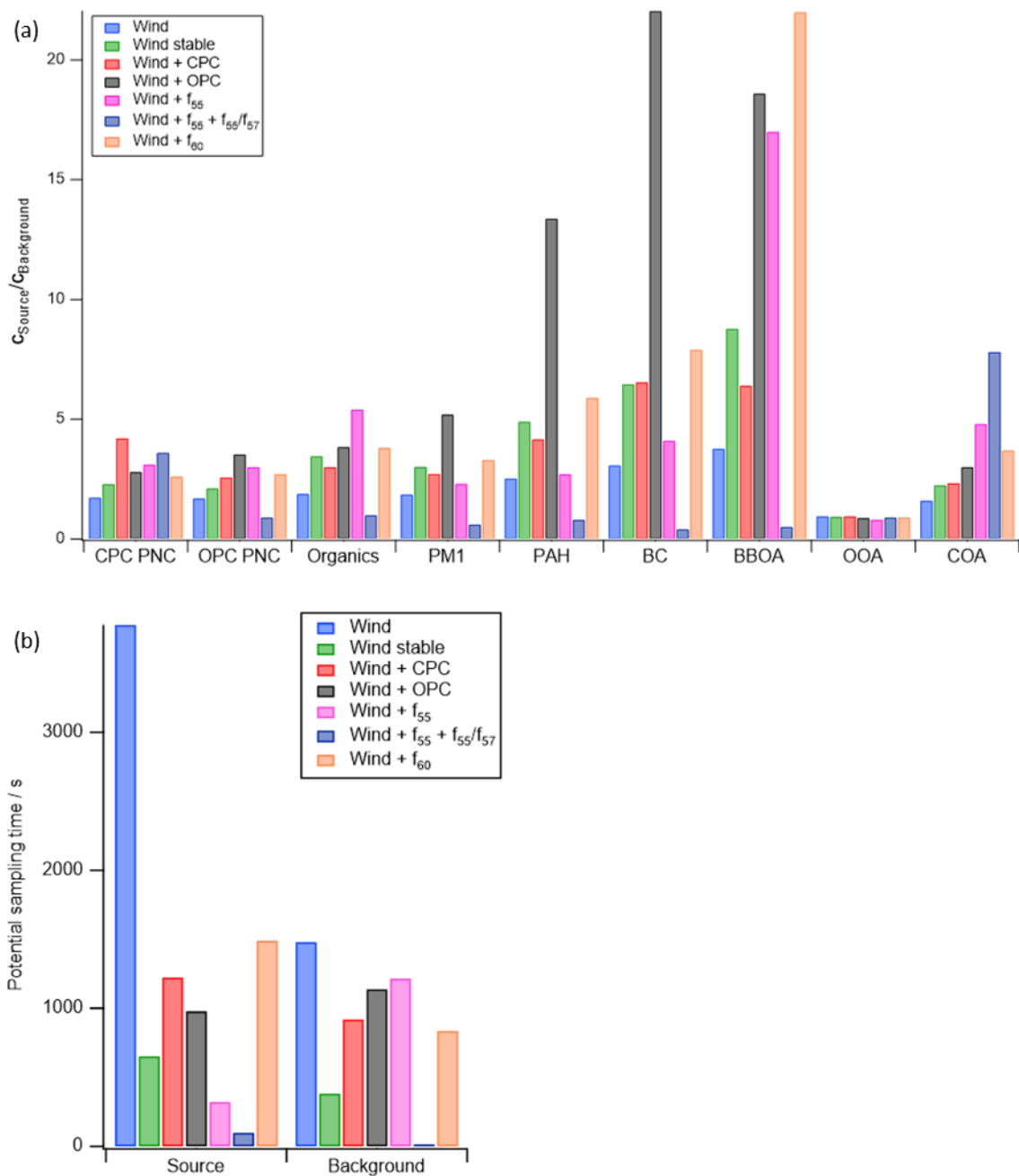
Figure 5: Ratio of averaged mass concentration and PNC of "source" and "background" aerosols, according to the seven different sampling scenarios (a), and related potential source emission and background aerosol sampling times (b).
