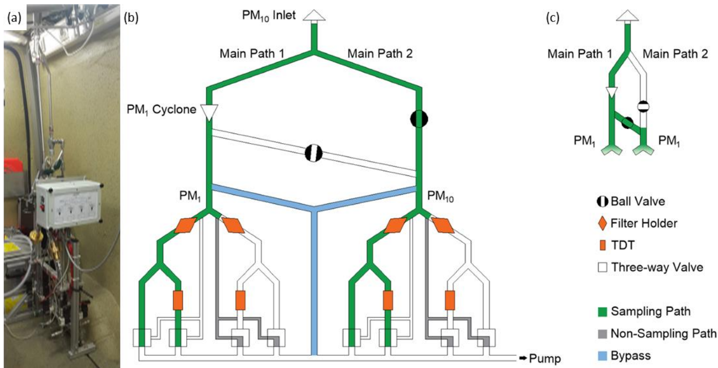
Figure 1: Photo (a) and scheme (b+c) of the AERTRACC sampler with active flow paths marked in green for sampling flows, in grey for non-sampling flows, and in blue for bypass flows (b: sampling mode \text{PM}_1+\text{PM}_{10} , c: sampling mode \text{PM}_1 only). Needle and dosing valves are located in each path directly upstream of the pump and are not shown in the scheme.
