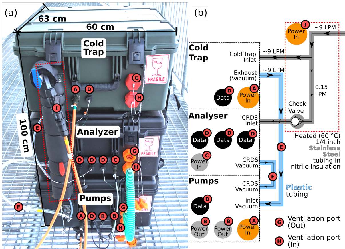
Figure 1. Overview of the ISE-CUBE system. (a) ISE-CUBE in stacked configuration (from top to bottom): Cold Trap expansion module; Analyzer module; and Pump module. (b) Flow diagram for the entire ISE-CUBE system, including flow rates and connectors. A heated inlet assembly (red dotted area in both) connects the three modules for common gas transmission. See text for details.
