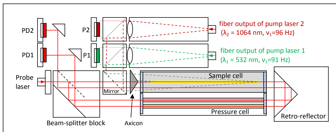
Figure 1. Schematic representation of the PTAAM-2 \lambda setup.
