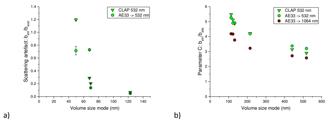
Figure 14. Scattering artefact of filter photometers the CLAP and the AE33 for different sizes of ammonium sulfate particles (a). Multiple scattering parameter C for different sizes of soot (b). For most measurements, the standard error was smaller than the symbol.
