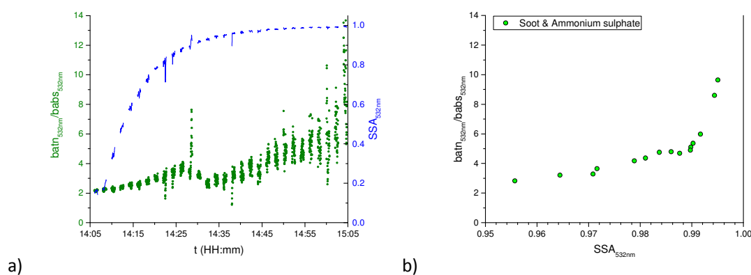
Figure 15. Measurement of externally mixed diesel soot and ammonium sulphate. The ratio between the AE33 attenuation coefficient and the PTAAM-2λ absorption coefficient and single-scattering albedo as a function of time (a). There was a filter change for the AE33 at 14:28. Attenuation to absorption ratio as a function of the single-scattering albedo (b).
