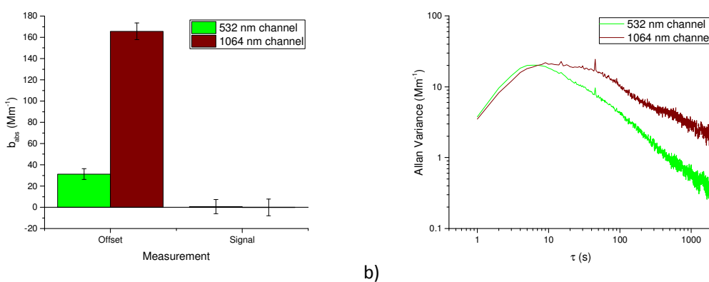
Figure 10. Average value and standard deviation of the offset and signal for filtered air (a); Allan variance (b).
