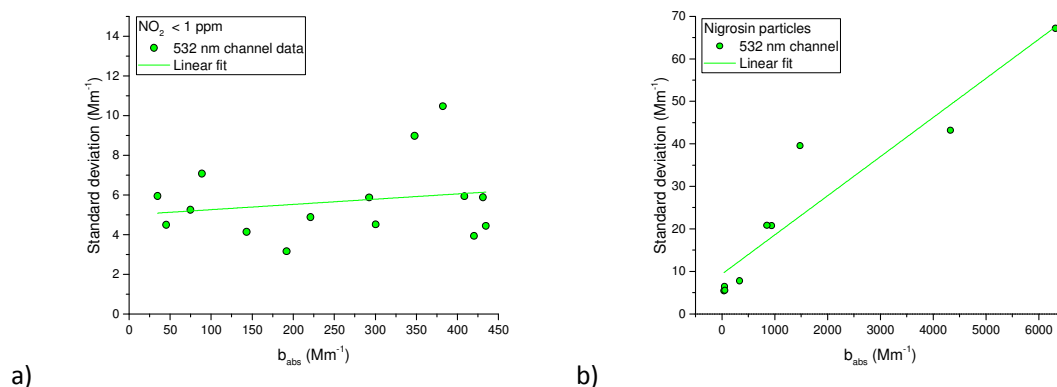
Figure 12. Standard deviation of the 532 nm channel data during measurement of NO 2 (a) and nigrosin (b).
