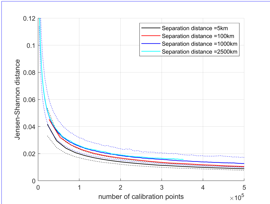
Figure 9. Impact of the separation distance of points in the pairs of Z-PDFs on the J-S distances as a function of the number of points for the PDFs of W-band calibrating targets. The four continuous coloured lines correspond to the median of the J-S distances for different separation distances, as indicated in the legend. The black and the blue dashed lines correspond to the 5 th and 95 th percentiles for the 5 and the 1000 km separation distances.
