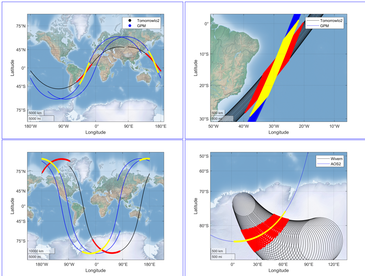
Figure 2. Quasi-intersection footprints between the inclined Tomorrow.io and the Ka-DPR radar (top panels) and the AOS2 polar W-band radar and the conically scanning Wivern radar (bottom panels) according to criterion #7. The left panels represent the ground tracks of the two orbits whereas the right panels depict the details of the two radar footprints at the ground in the region where the ground tracks intersect.
