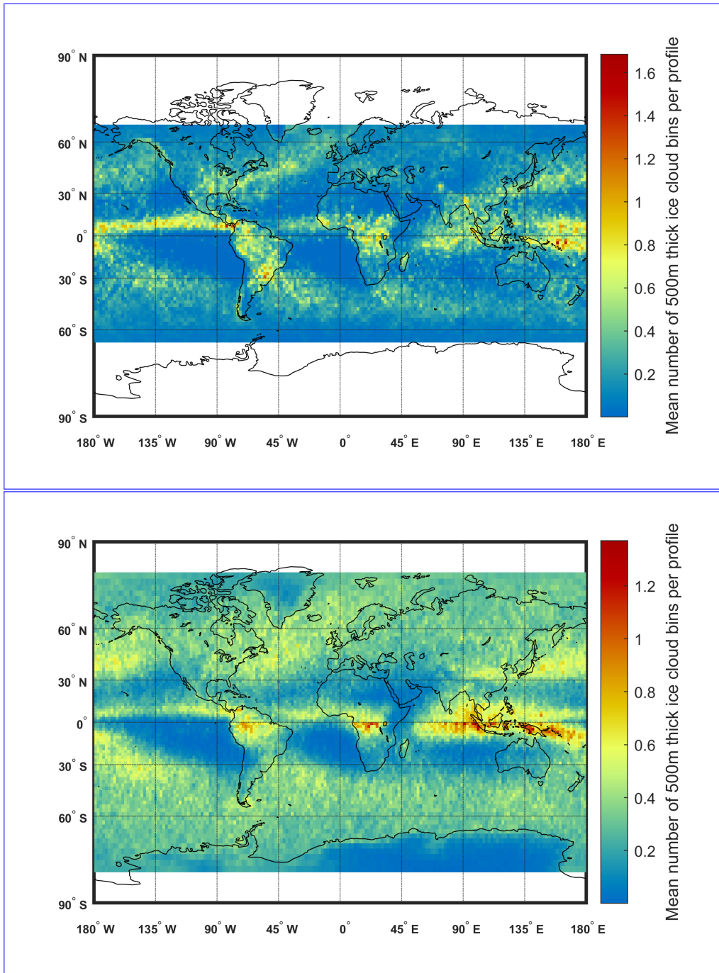
Figure 5. Global distribution of the mean number of 500 m-thick radar range bins per profile of Ka-band (top) and of 500 m-thick bins of W-band (bottom) ice calibrating clouds as derived by 4 years of GPM and CloudSat data, respectively. The resolution is 2^\circ \times 2^\circ . For a given 2^\circ \times 2^\circ a mean number of 500 m thick ice cloud bins per profile equal one means that for any vertical profile collected in that region, an average of one 500 m thick calibrating ice cloud bin will be detected.
