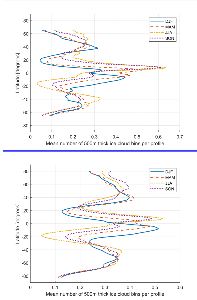
Figure 6. Zonal variability of the mean number of 500 m thick radar range bins per profile for Ka-band and W-band ice calibrating clouds, respectively. Four different seasons are plotted, as indicated in the legend. The same datasets adopted to produce Fig. 5 have been used.
