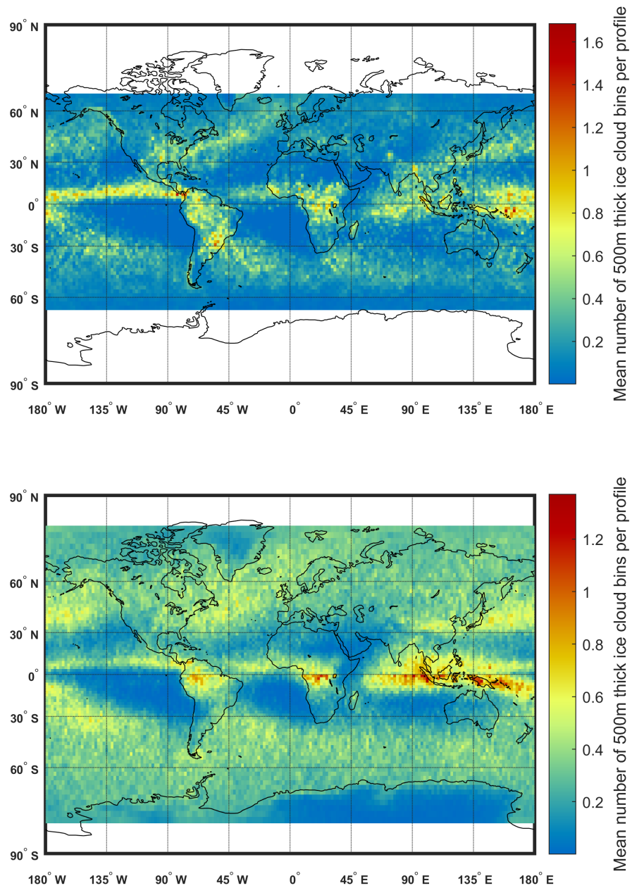
Figure 5. Global distribution of the mean number of 500 m-thick radar range bins per profile of Ka-band (top) and W-band (bottom) ice calibrating clouds as derived by 4 years of GPM and CloudSat data, respectively. The resolution is 2^\circ \times 2^\circ . For a given 2^\circ \times 2^\circ a mean number of 500m thick ice cloud bins per profile equal one means that for any vertical profile collected in that region, an average of one 500m thick calibrating ice cloud bin will be detected.
