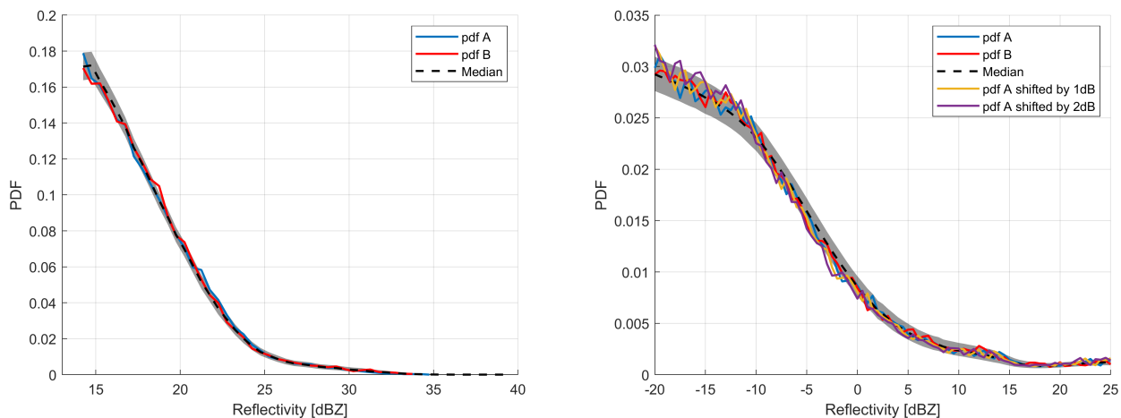
Figure 7. Envelope (5-95 th percentile) of Z-PDFs for the Ka-band ice calibrating clouds (left panel) and for the W-band ice calibrating clouds (right panel) for two sets of cloud reflectivities sampled with a separation of 500 km. The black line represents the median Z-PDF whereas the blue and red curve represent two PDFs randomly selected. Both PDFs have been built with about 50,000 calibration points (Tab. 4 can be used to compute the time needed to collect such sample according to the different configurations and quasi-coincidence criteria). For the W-band PDF the effect of a positive bias of 1 and 2 dB is also shown.
