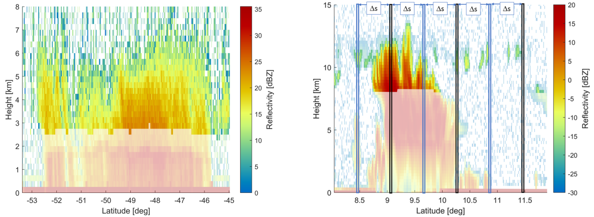
Figure 4. Example of GPM Ka-band (left) and CloudSat W-band (right) reflectivity profiles over a mid-latitude and a tropical system, respectively. The regions with bright colors represent the points that are used as natural target calibrating points. In the right panel the procedure adopted in step 3 is illustrated (see description in Sect. 2.3 for details). Each dashed box represent a 5 km along track slice. The reflectivities of the calibrating points are clustered together in correspondence to the black and blue boxes, which are separated by a given distance \Delta s (for this specific example of the order of 500 km).
