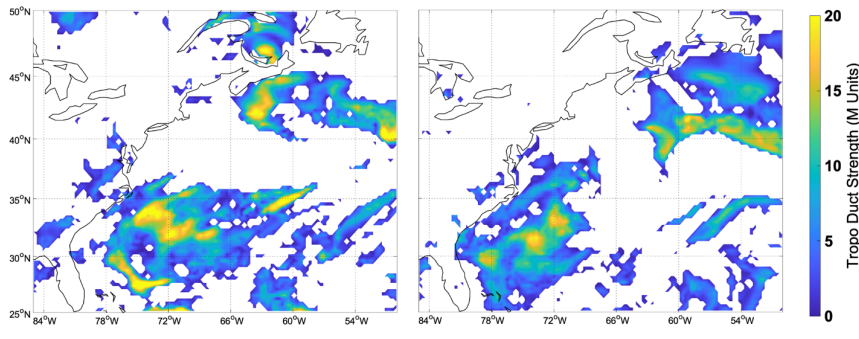
115 Figure 4 shows tropospheric ducting maps of modified refractivity (in M units) based on temperatures, pressures and humidities in ERA5 reanalysis data. The left panel shows 19 UT on 14 July 2021, while the right panel shows 14 UT on 13 July 2021.
