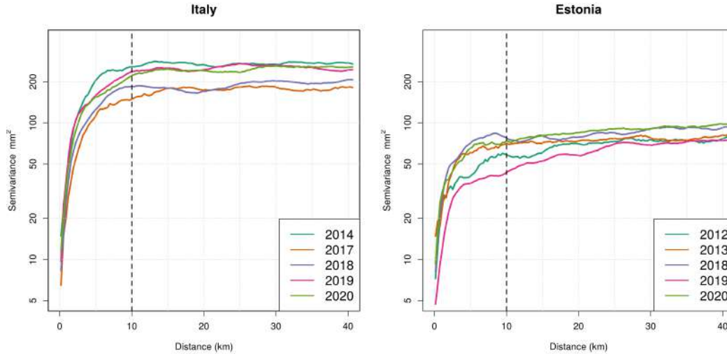
Figure 2. Empirical variograms for hourly rainfall annual maxima based on R(Z_h, K_{dp}) hourly rainfall estimations in Italy Area 1 (left) and Estonia (right).
