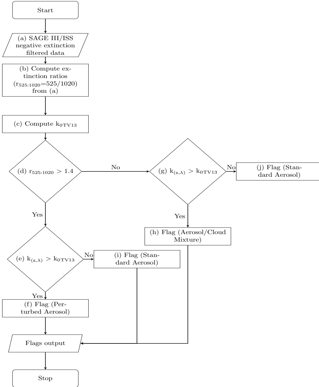
Figure 5. Flow chart of TV13* method. k_{(z,\lambda)} in the flow chart represents extinction coefficient at altitude "z" and wavelength " \lambda ", whereas k_{0TV13} = k_a + 3.0 \cdot MAD . k_{0TV13} is computed following TV13 by using extinction measurements with r_{525:1020} > 2 . It should be noted that the steps involved ((b) through (j)) in the flowchart is same as TV13 method, except that the seasonal data between 1999-2005 were used for the method presented in TV13. For our analyses, instead of seasonal data, we use monthly data collected between 2017 and 2021.
