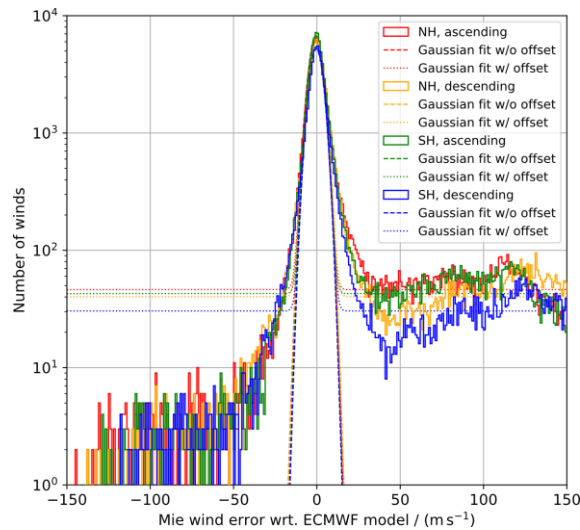
Figure 4. Histograms of the L2B Mie-cloudy wind error against ECMWF model background data from the period between 20 and 25 March 2022 for Northern/Southern Hemisphere and ascending/descending orbits. The dashed and dotted lines represent Gaussian fits without and with offset, respectively.
