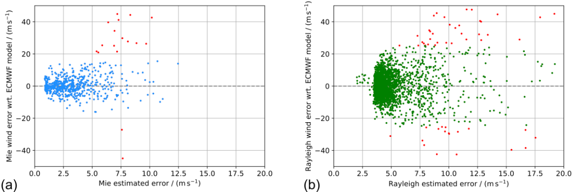
Figure 3. L2B Mie-cloudy (a) and Rayleigh-clear (b) wind error with respect to the ECMWF model background winds versus the L2B EE for the 11 underflights of the AVATAR-T campaign. The red data points represent outliers as identified by the modified Z-score ( |Z_m| > 3.5 ). Note that there are many more Mie outliers with errors greater than \pm 50 \text{ m}\cdot\text{s}^{-1} .
