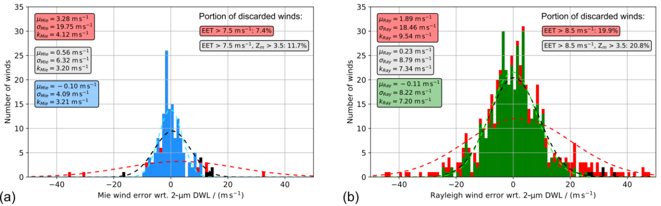
Figure 10. Histograms of the Mie-cloudy (a) and Rayleigh-clear (b) wind error with respect to the 2-μm DWL wind data acquired during the AVATAR-T campaign. The blue and green columns denote the histogram after discarding winds with \text{EE} > 7.5 \text{ m}\cdot\text{s}^{-1} (Mie) and \text{EE} > 8.5 \text{ m}\cdot\text{s}^{-1} (Rayleigh), and subsequent application of a QC based on the modified Z-score (threshold: 3.5). The red columns indicate the winds that are filtered out by the EE threshold, while the black columns describe wind data that are additionally filtered out by the modified Z-score. The statistical parameters given in the boxes refer to the three different subsets (red: all data; grey: EE filter only; blue/green: EE filter plus modified Z-score filter).
