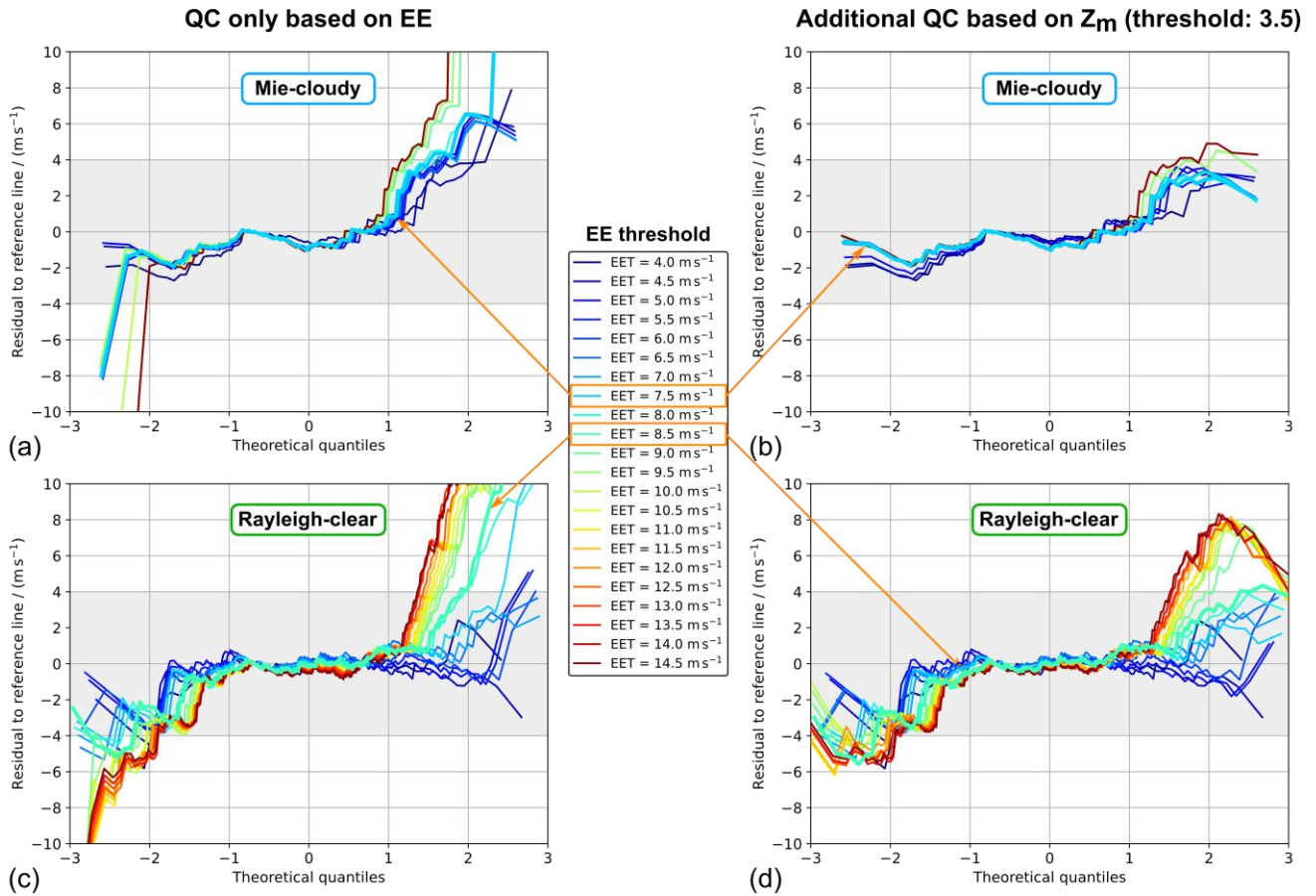
Figure 9. Residual L2B Mie-cloudy (top row) and Rayleigh-clear wind speed error (bottom row) after subtraction of the quartile reference line from the normal quantile plot based on the comparison to 2- \mu\text{m} DWL wind data from the AVATAR-T campaign. The residuals are calculated for different EE thresholds (EET), as indicated by the colour scale. In panels (a) and (c) no additional outlier removal was applied, whereas the plots in panels (b) and (d) are obtained after additional QC based on the modified Z-score ( |Z_m| > 3.5 ). The curves corresponding to the EE thresholds that are deemed reasonable to provide robust statistical results (Mie: 7.5 \text{ m}\cdot\text{s}^{-1} , Rayleigh: 8.5 \text{ m}\cdot\text{s}^{-1} ) are plotted by thick lines.
