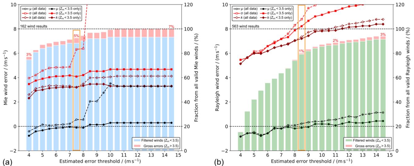
540 Figure 8. Same as Fig. 6, but for the statistical comparison of L2B Mie-cloudy (a) and Rayleigh-clear winds (b) against 2- \mu\text{m} DWL wind data. The EE thresholds that are deemed reasonable to provide robust statistical results are highlighted by orange frames (see also Fig. 9).
