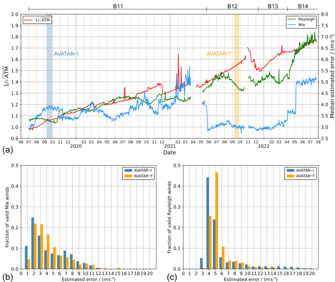
Figure 1. Temporal evolution of the reciprocal square-root of the of the atmospheric signal level ( 1/\sqrt{\text{ATM}} ) (red), normalized to the value from 26 July 2019, and the L2B Rayleigh-clear (green) and Mie-cloudy EE (blue) during the FM-B period (median per day). The baselines of the L2B product from which the data were extracted are indicated by the horizontal bars on the top of the plot. The lower panels depict the distribution of the Mie (b) and Rayleigh EE (c) for the periods and locations of the two DLR validation campaigns AVATAR-I (blue) and AVATAR-T (orange). The campaign periods are indicated by blue- and orange-shaded stripes in panel (a).
