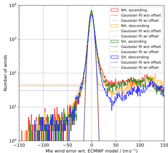
370 Figure 4. Histograms of the L2B Mie-cloudy wind error against ECMWF model background data from the period between 20 and 25 March 2022 for Northern/Southern Hemisphere and ascending/descending orbits. The dashed and dotted lines represent Gaussian fits without and with offset, respectively.
