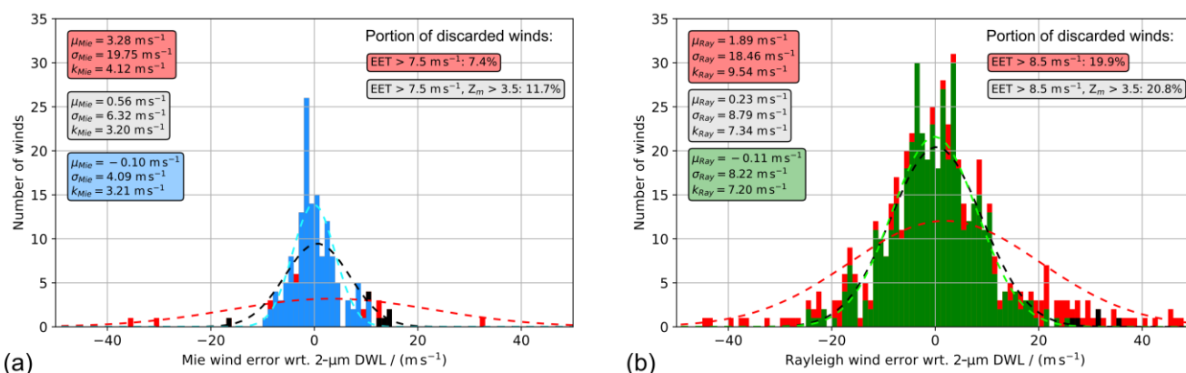
Figure 10. Histograms of the Mie-cloudy (a) and Rayleigh-clear (b) wind error with respect to the 2- \mu\text{m} DWL wind data acquired during the AVATAR-T campaign. The blue and green columns denote the histogram after discarding winds with EE > 7.5 \text{m}\cdot\text{s}^{-1} (Mie) and EE > 8.5 \text{m}\cdot\text{s}^{-1} (Rayleigh), and subsequent application of a QC based on the modified Z-score (threshold: 3.5). The red columns indicate the winds that are filtered out by the EE threshold, while the black columns describe wind data that are additionally filtered out by the modified Z-score. The statistical parameters given in the boxes refer to the three different subsets (red: all data; grey: EE filter only; blue/green: EE filter plus modified Z-score filter).
