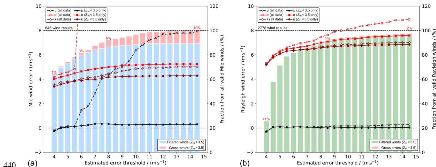
Figure 6. Results from the statistical comparison of L2B Mie-cloudy (a) and Rayleigh-clear winds (b) against ECMWF model background wind data from the AVATAR-T campaign depending on the EE threshold without and with outlier removal based on the modified Z-score. The bar plots depict the portion of filtered winds after QC ( |Z_m| < 3.5 ) (blue and green bars) and gross errors ( |Z_m| > 3.5 , red bars) from all wind results that are flagged valid in the L2B product and pass the specified EE threshold. The portion of gross errors is indicated above the bars. The dashed lines and open symbols refer to the statistical results (mean bias \mu , standard deviation \sigma , scaled MAD k ) without removing the gross errors from the datasets, while the solid lines represent the statistical parameters after QC based on the modified Z-score.
