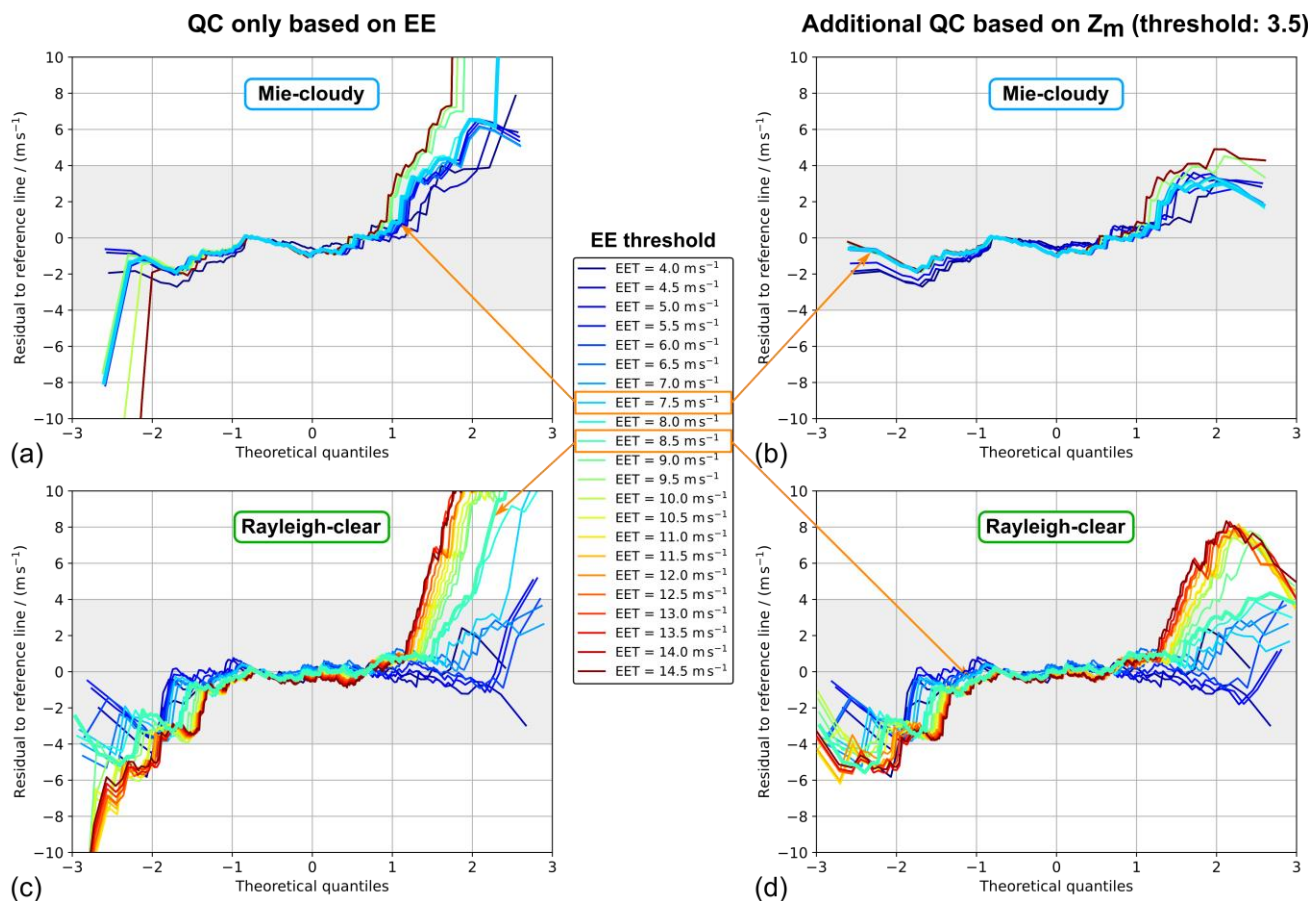
Figure 9. Residual L2B Mie-cloudy (top row) and Rayleigh-clear wind speed error (bottom row) after subtraction of the quartile reference line from the normal quantile plot based on the comparison to 2- \mu\text{m} DWL wind data from the AVATAR-T campaign. The residuals are calculated for different EE thresholds (EET), as indicated by the colour scale. In panels (a) and (c) no additional outlier removal was applied, whereas the plots in panels (b) and (d) are obtained after additional QC based on the modified Z-score ( |Z_m| > 3.5 ). The curves corresponding to the EE thresholds that are deemed reasonable to provide robust statistical results (Mie: 7.5 \text{ m s}^{-1} , Rayleigh: 8.5 \text{ m s}^{-1} ) are plotted by thick lines.
