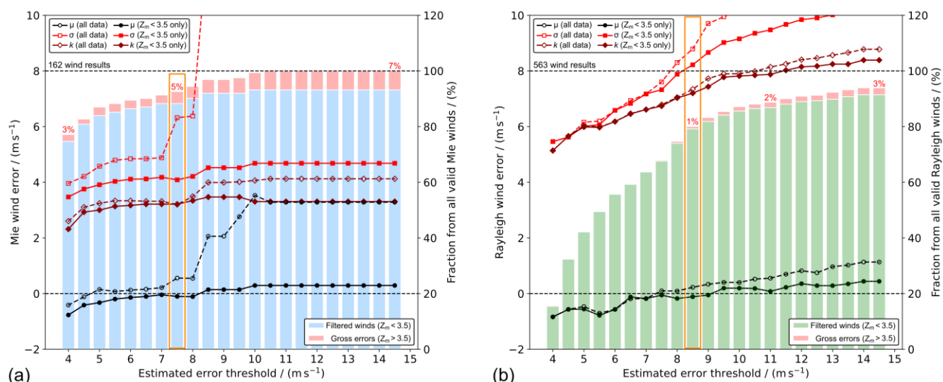
Figure 8. Same as Fig. 6, but for the statistical comparison of L2B Mie-cloudy (a) and Rayleigh-clear winds (b) against 2- \mu\text{m} DWL wind data. The EE thresholds that are deemed reasonable to provide robust statistical results are highlighted by orange frames (see also Fig. 9).
