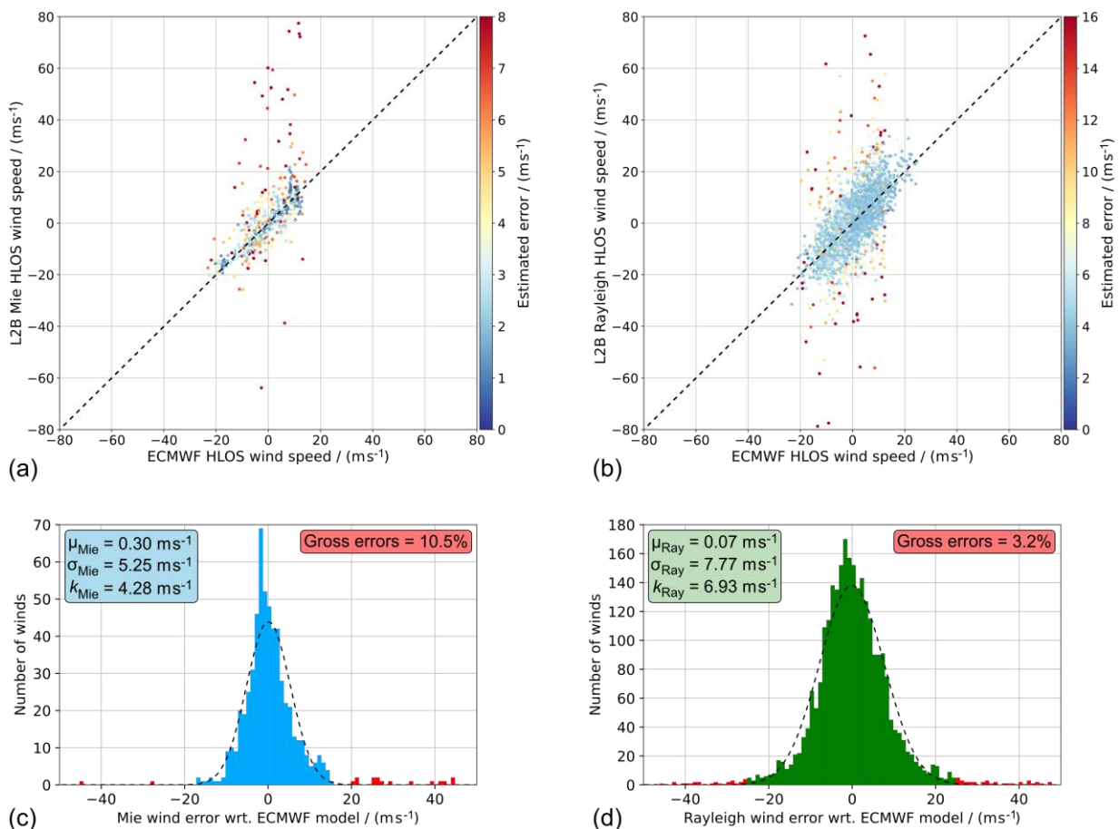
285 Figure 2. Scatterplots comparing the L2B Mie-cloudy (a) and Rayleigh-clear (b) wind results against ECMWF model winds from the 11 underflights of the AVATAR-T campaign. The colour-coding describes the L2B EE of the wind results. The statistical parameters without and with outlier removal using the modified Z-score are given in Table 2. (c,d) Histograms of the respective wind errors (L2B minus ECMWF model) in bins of 1 \text{ m s}^{-1} . The red bars indicate gross errors as identified by the modified Z-score. The dashed lines represent Gaussian fits of the error distributions after outlier removal. The statistical parameters after outlier removal are given in the insets.
