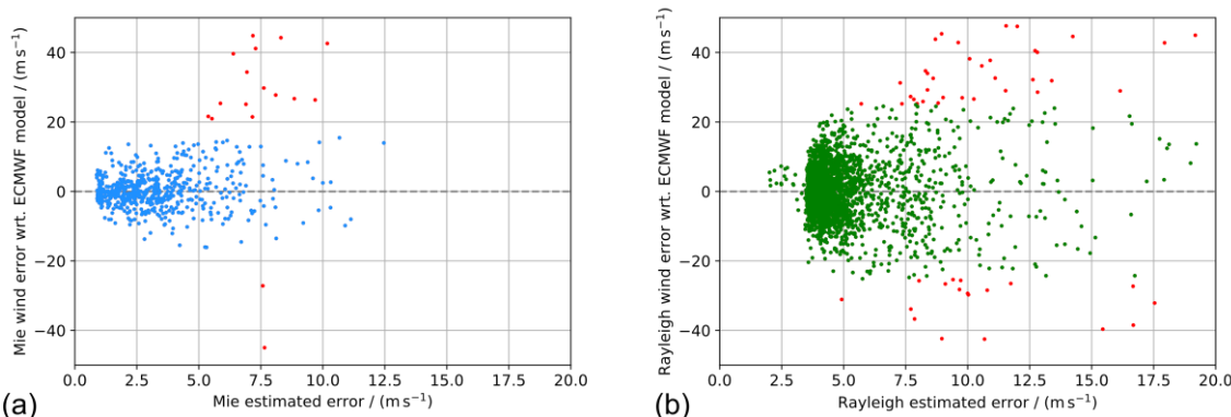
330 Figure 3. L2B Mie-cloudy (a) and Rayleigh-clear (b) wind error with respect to the ECMWF model background winds versus the L2B EE for the 11 underflights of the AVATAR-T campaign. The red data points represent outliers as identified by the modified Z-score ( |Z_m| > 3.5 ). Note that there are many more Mie outliers with errors greater than \pm 50 \text{ m}\cdot\text{s}^{-1} .
