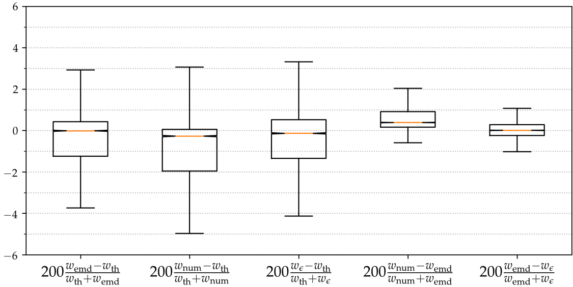
Figure 5. Comparison of the different ways to compute the Wasserstein distance over the Gaussian puffs database. Relative errors in percent between w_{\text{emd}} , w_{\text{th}} , w_{\text{num}} , and w_{\epsilon} (e). The orange line is the median. Box boundaries are defined by the first and the third quartiles. The whiskers are set at 150% of the inter-quartile range
