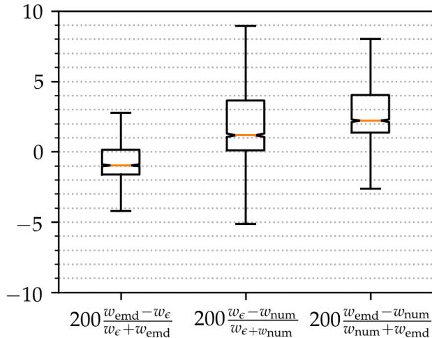
Figure 7. Comparison of the different ways to compute the Wasserstein distance over the realistic database. Relative errors in percent between w_{\text{emd}} , w_{\text{num}} , and w_{\epsilon} ( e ). The orange line is the median. Box boundaries are defined by the first and the third quartiles. The whiskers are set at 150% of the inter-quartile range
