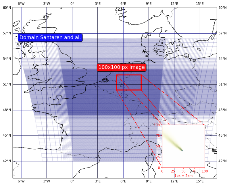
Figure 6. Experimental setup. Simulation domain The simulation grid from Santaren et al. (2021) is in blue, centred on Belgium. Example The zoom in red corresponds to the vicinity around the Neurath power plant. An example of an the Neurath power plant CO 2 plume image used in red is also displayed.
