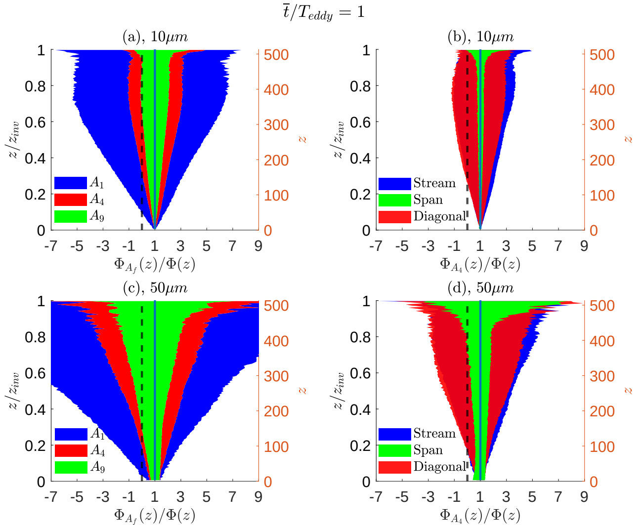
Figure 8. Vertical profiles of flux ranges in sampled (a,b) 10\mu m and (c,d) 50\mu m aerosol particle fluxes for a time-averaged duration of 1T_{eddy} . The directional sampling (b,d) are for a sampling area of A_4 . Colors from Fig. 6 correspond to those in the current figure. The dashed black line is the zero value reference of net flux, while the solid black line is the reference value for the sampled aerosol particle flux equal to the true, domain-wide LES aerosol particle flux.
