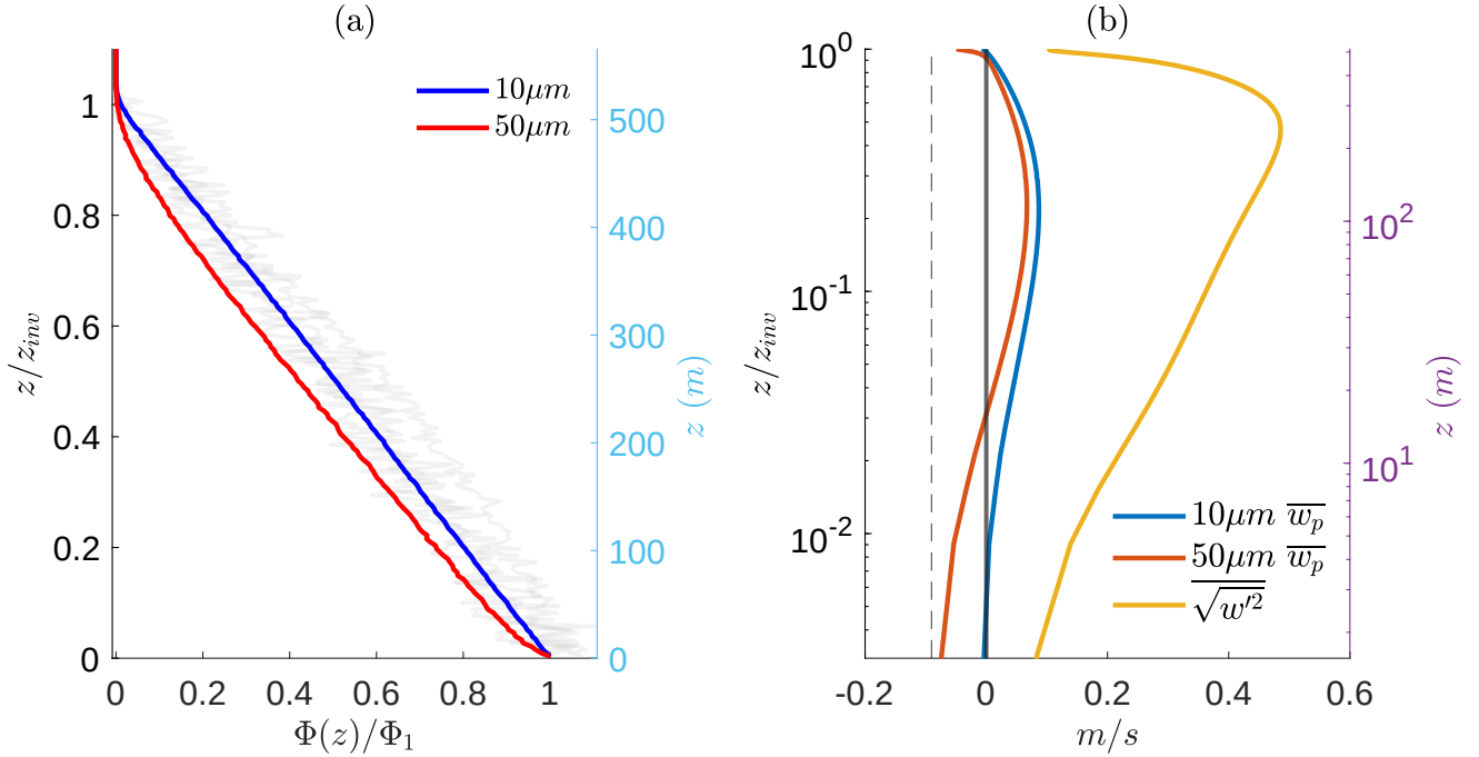
Figure 3. (a): Vertical flux profile for 10 and 50\mu m particles normalized by the respective flux at the first grid point ( \Phi_1 ). The 3 faded profiles are the instantaneous net fluxes at the start, middle, and end of the averaging time for 10\mu m particles. (b): Comparison of mean particle velocity for both sizes and the standard deviation of the flow vertical velocity at different heights (left vertical axis is scaled by the inversion height and the right side is the dimensional height). The dashed line is the gravitational settling velocity for 50\mu m particles.
