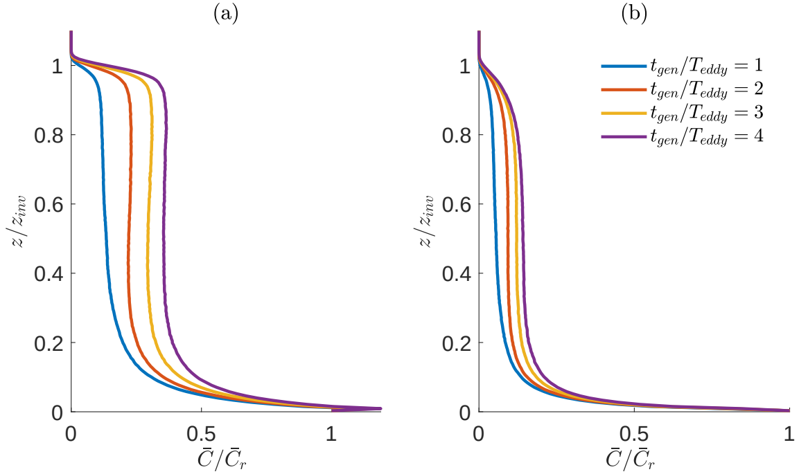
Figure 2. Normalized concentration profiles for (a) 10\ \mu\text{m} and (b) 50\ \mu\text{m} diameter aerosols, at intervals of t_{\text{gen}}/T_{\text{eddy}} . The term t_{\text{gen}} is the time since the initiation of surface aerosol generation; T_{\text{eddy}} is the largest eddy time scale, a function of the inversion height and convective velocity scale: it is approximately 12 minutes.
