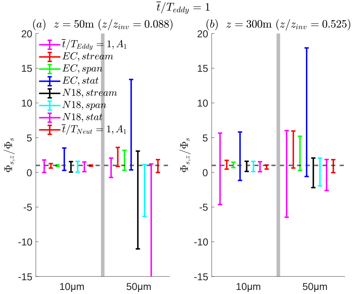
Figure 14. Summary of the various methods for inferring effective surface fluxes from (a) z/z_{inv} = 0.088 and (b) z/z_{inv} = 0.525 . The left side of the abscissa in each plot is for 10\mu\text{m} diameter aerosol particles, and the right side represents 50\mu\text{m} sizes. The first legend entry corresponds to the sub-region sampling analysis in Section 3.2. The second set of legend entries is the eddy covariance (EC) and streamwise (as stream), spanwise (as span), and stationary (as stat), corresponding to the simulated instrumentation. The next set of legends corresponds to the Nissanka et al. (2018) model as N18, in which the elevated concentration is constrained by the simulated instrumentation. The last legend item is the surface flux variation from a neutral stability condition for \bar{t}/T_{neut} = 1 . Aside from the last legends, the data is based on an averaging time of 1T_{eddy} . The dashed reference line represents \Phi_{s,z}/\Phi_s = 1 , meaning that the inferred surface flux matches the LES surface flux.
