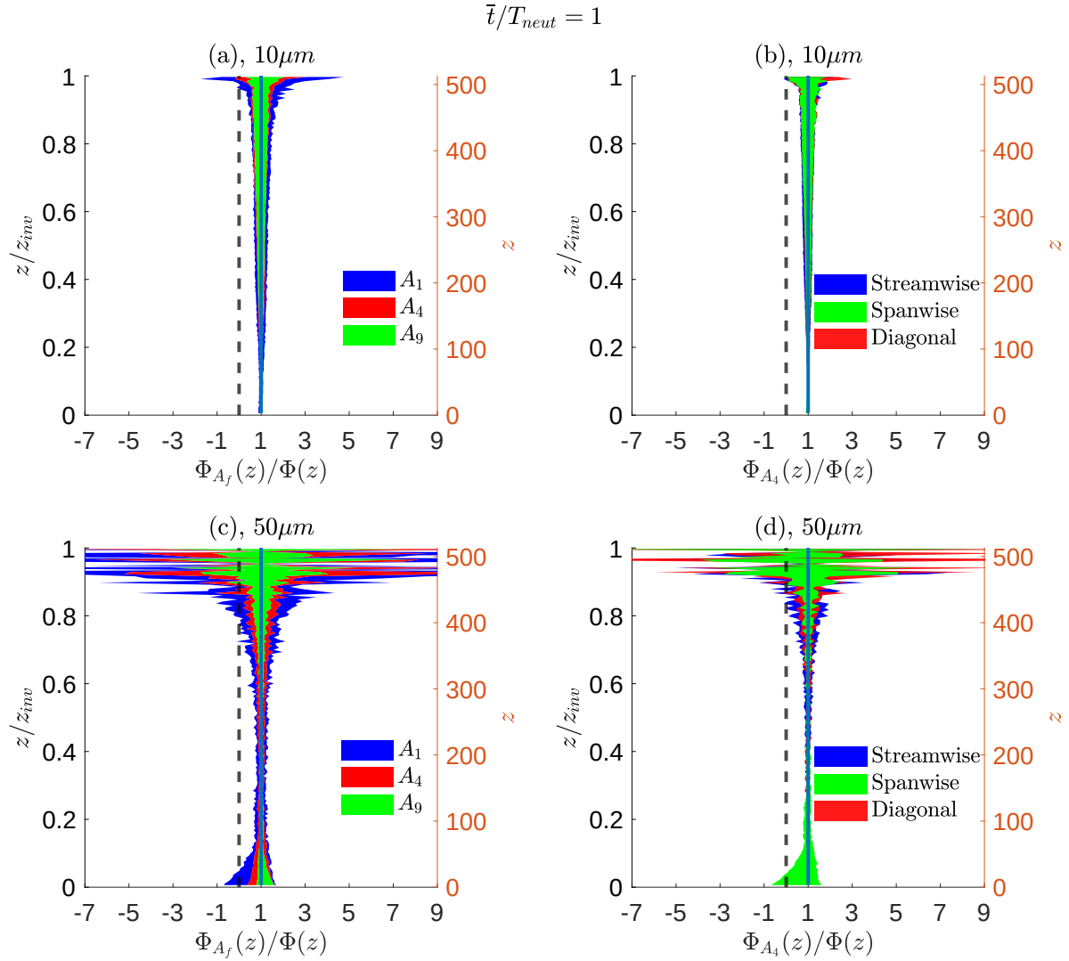
Figure 13. Vertical profiles of predictive flux ranges for 10\,\mu m (a, b) and 50\,\mu m (c, d) aerosol particle sizes. Left subplots (a, c) are different subsampling sizes and the right subplots (b, d) are directional subsampling given A_4 . The panel layout and configurations are identical to Fig. 8.
