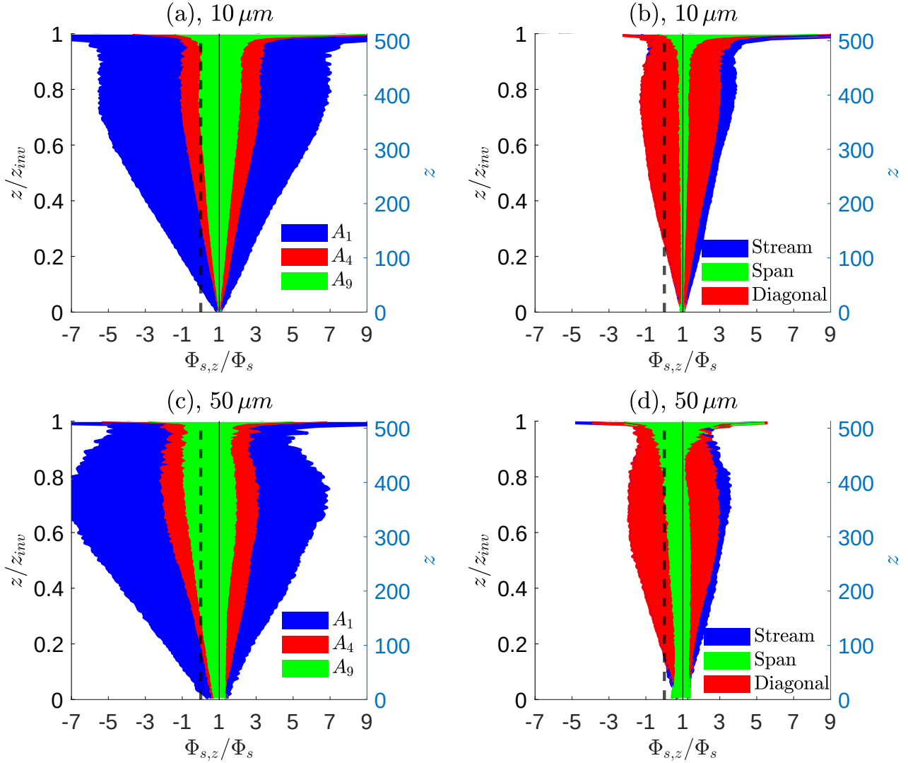
Figure 9. Inferred effective surface fluxes \Phi_{s,z} normalized by the true effective surface flux \Phi_s as a function of sampling height for 10\,\mu\text{m} (a,b) and 50\,\mu\text{m} (c,d) aerosol particles. Elevated fluxes are used to infer surface fluxes via linear extrapolation. The left subplots (a,c) illustrate variability due to area coverage, and the right subplots (b,d) illustrate directional sampling for the same total area A_4 .
