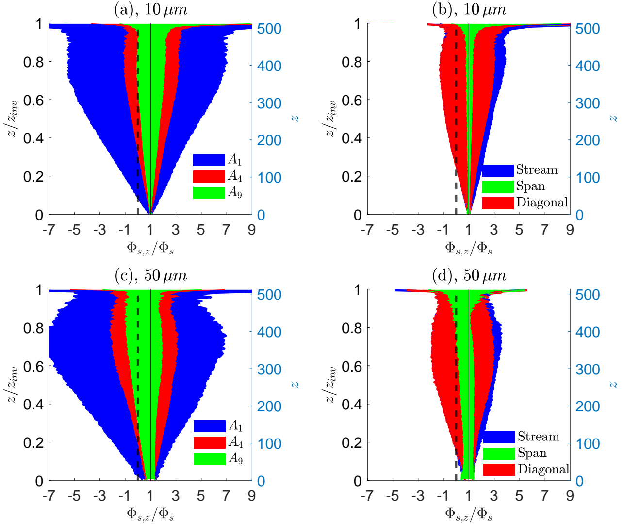
Figure 9. Inferred effective surface fluxes \Phi_{s,z} normalized by the true effective surface flux \Phi_s as a function of sampling height for 10\,\mu\text{m} (a,b) and 50\,\mu\text{m} (c,d) aerosol particles. Elevated fluxes are used to infer surface fluxes via linear extrapolation. The left subplots (a,c) illustrate variability due to area coverage, and the right subplots (b,d) illustrate directional sampling for the same total area A_4 .
