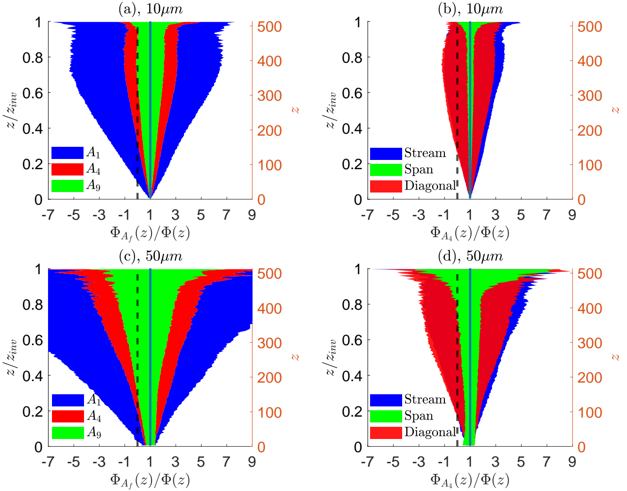
Figure 8. Vertical profiles of flux ranges in sampled (a,b) 10\mu m and (c,d) 50\mu m aerosol particle fluxes for a time-averaged duration of 1T_{eddy} . The directional sampling (b,d) are for a sampling area of A_4 . Colors from Fig. 6 correspond to those in the current figure. The dashed black line is the zero value reference of net flux, while the solid black line is the reference value for the sampled aerosol particle flux equal to the true, domain-wide LES aerosol particle flux.
