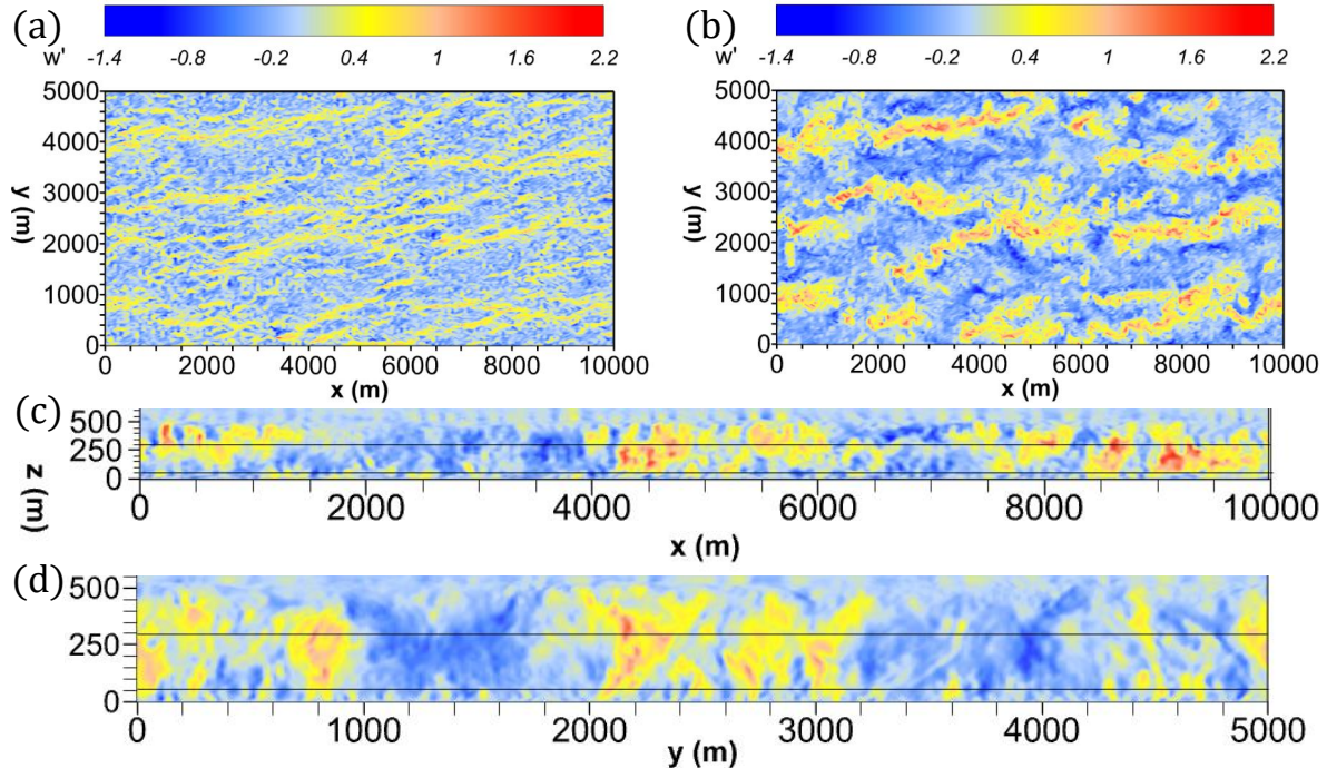
Figure 4. Image of instantaneous vertical velocity contours for a x - y top-down view (a,b), x - z streamwise side view (c), and y - z spanwise side view (d). The x - y top-down views are at (a): z/z_{inv} = 0.083 (or 50m) and at (b): z/z_{inv} = 0.525 (or 300m). x is the streamwise direction of the flow. The solid black lines across (c) and (d) are the heights of (a) and (b) plane visualizations.
