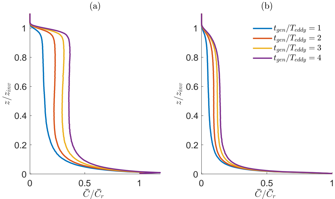
Figure 2. Normalized concentration profiles for (a) 10\ \mu\text{m} and (b) 50\ \mu\text{m} diameter aerosols, at intervals of t_{gen}/T_{eddy} . The term t_{gen} is the time since the initiation of surface aerosol generation; T_{eddy} is the largest eddy time scale, a function of the inversion height and convective velocity scale: it is approximately 12 minutes.
