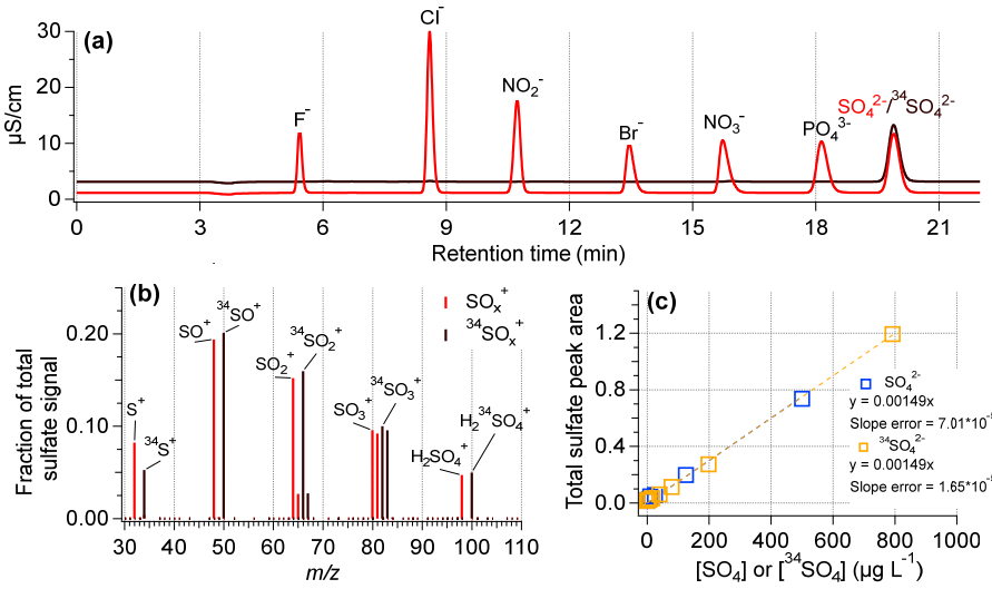
Figure 2. Assessment of the instrumental response to \text{SO}_4 and ^{34}\text{SO}_4 . a) IC chromatograms of an anion standard mix (in light red) and a ^{34}\text{SO}_4^{2-} standard. The \text{SO}_4^{2-} and ^{34}\text{SO}_4^{2-} concentrations were 3 \text{ mg L}^{-1} in each solution. b) HR-AMS mass spectra for a solution
