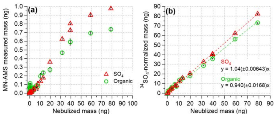
270 Figure 3. a) The MN-AMS measured mass of organics and SO 4 compared to the expected mass of sucrose and SO 4 . The ratio between the two values gives the nebulization efficiency of each component. The MN-AMS measured mass is not linearly proportional to the nebulized mass, but this can be corrected with internal standardization (as in Fig. 1b)-3b). The ratio between the two values gives the nebulization efficiency of each component. b) The 34 SO 4 -normalized mass of organics and SO 4 compared to the nebulized mass.
