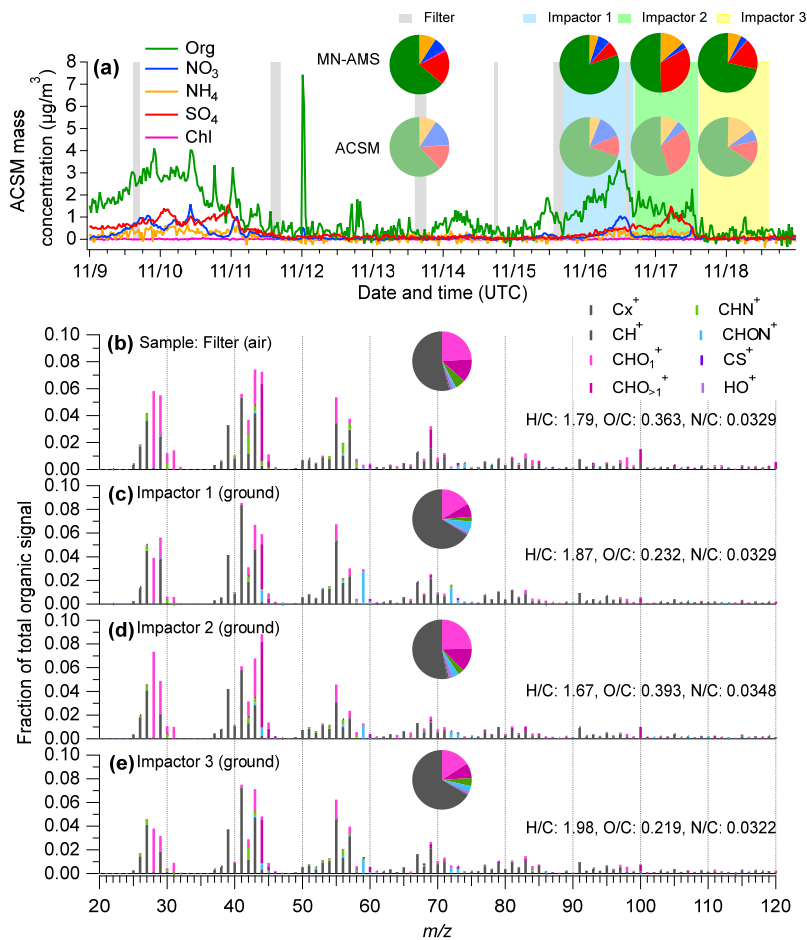
Figure 5. Comparison of offline \text{PM}_{2.5} composition measured offline using the MN-AMS vs. the real-time \text{PM}_1 measured using a Quadrupole ACSM. a) Time series of the ACSM-measured NR- \text{PM}_1 species at the SGP site. The inset pie charts compare the composition measurements by the MN-AMS (darker colors) and the ACSM (lighter colors) for the same time periods. b-e) High mass resolution organic spectra colored by 8 ion categories for the SGP filter and impactors measured by MN-AMS. The average atomic ratios in the organics of each samples are shown in the legends.
