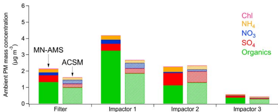
Figure 6. Comparison of the ACSM-measured ambient NR- \text{PM}_{10} mass concentration and the MN-AMS back-calculated ambient NR- \text{PM}_{2.5} mass concentration at the SGP site. Sampling time periods for the filter and impactors are shown as shaded areas in Fig. 5a.
