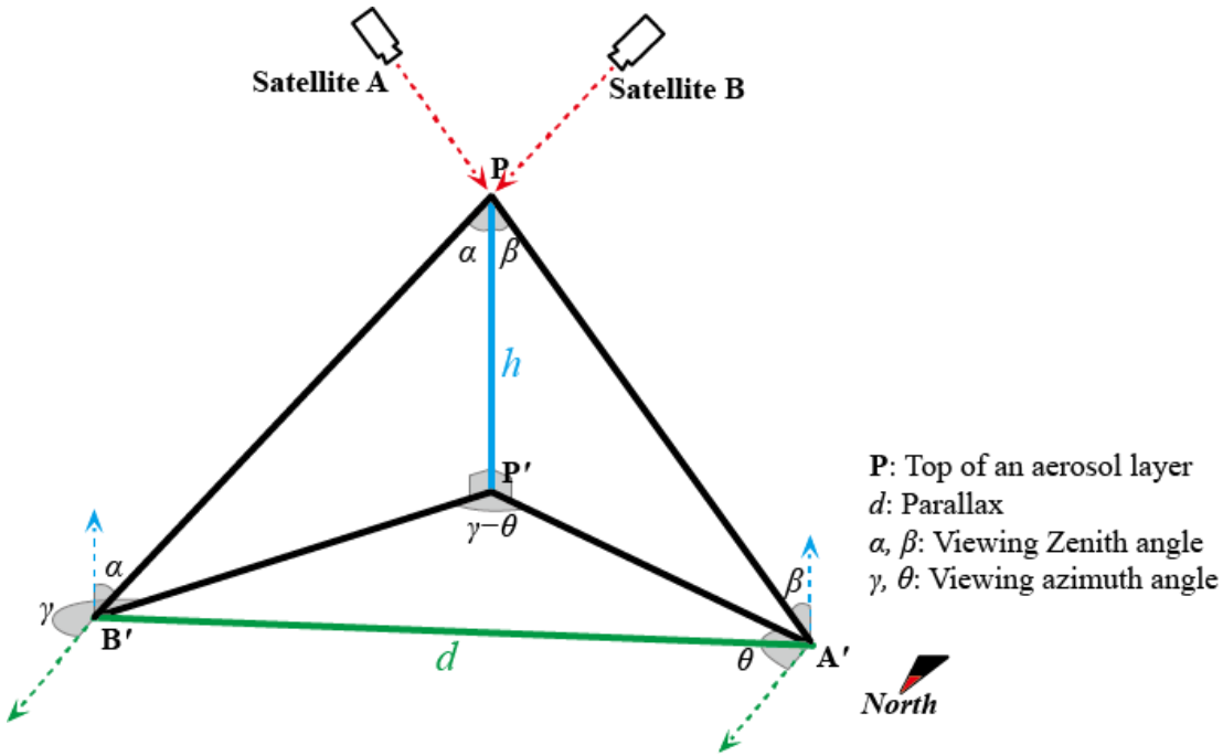
615 Figure 2: Graphical depiction of parallax from the top of the aerosol layer (P) observed using a pair of satellites (A and B).
