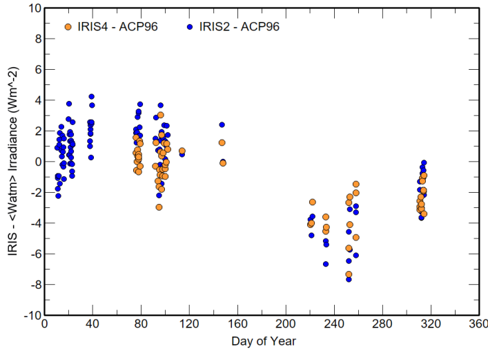
440 Figure 7. Daily mean irradiance differences ( W_{IRIS} - \langle W_{atm} \rangle ) between the mean IRIS ( W_{IRIS} ) and linear LSQ interpolated ACP96 ( \langle W_{atm} \rangle ), using the new equation with \epsilon_c = 0.0225 , \gamma = 6.5 , and \tau = 0.977 .
