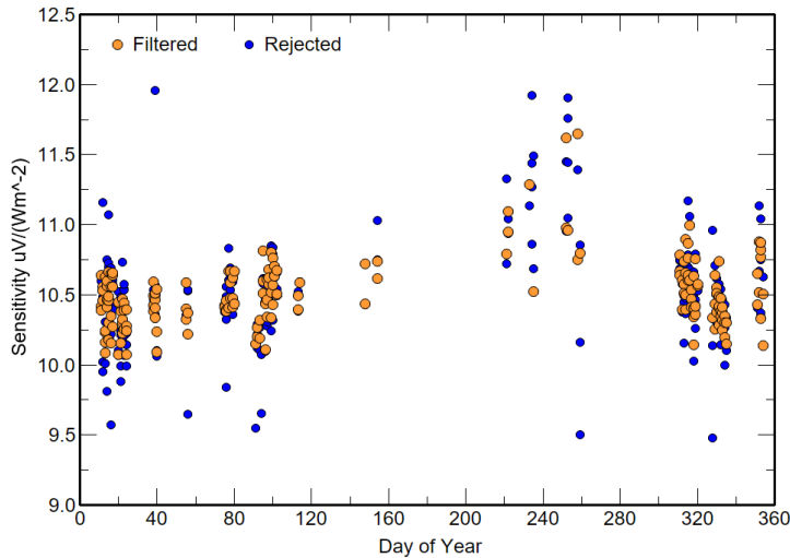
Figure 9. Responsivity \langle C \rangle values presented in figure 6 but filtered for standard deviations of ACP96 \tau W_{atm} during the cooling-heating period that are less than 0.6 \text{ Wm}^{-2} are gold, and those with higher standard deviations are in blue.
