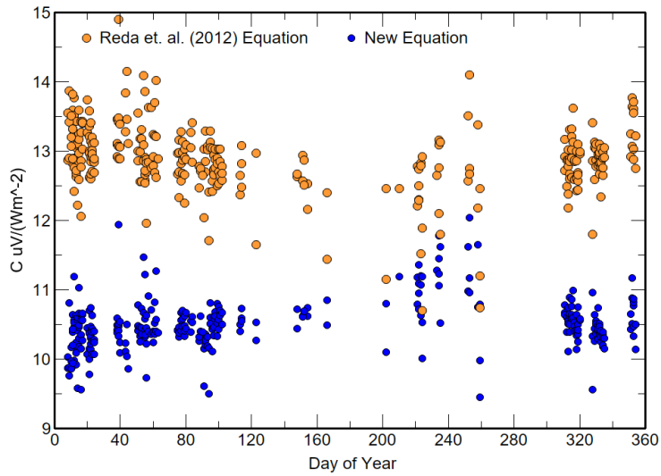
590 Figure 12. The derived C values derived from 244 linear LSQ calibration in 2020 for the Reda et al., 2012 and new equation using and concentrator emissivity of 0.0225 for both and a convection coefficient of 6.5 for the new equation.
