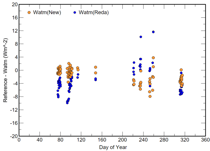
Figure 13: The comparison of \langle W_{atm} \rangle derived from the new and Reda et al., 2012 equations to the mean IRIS4 irradiances for each linear LSQ calibration period in 2020.
