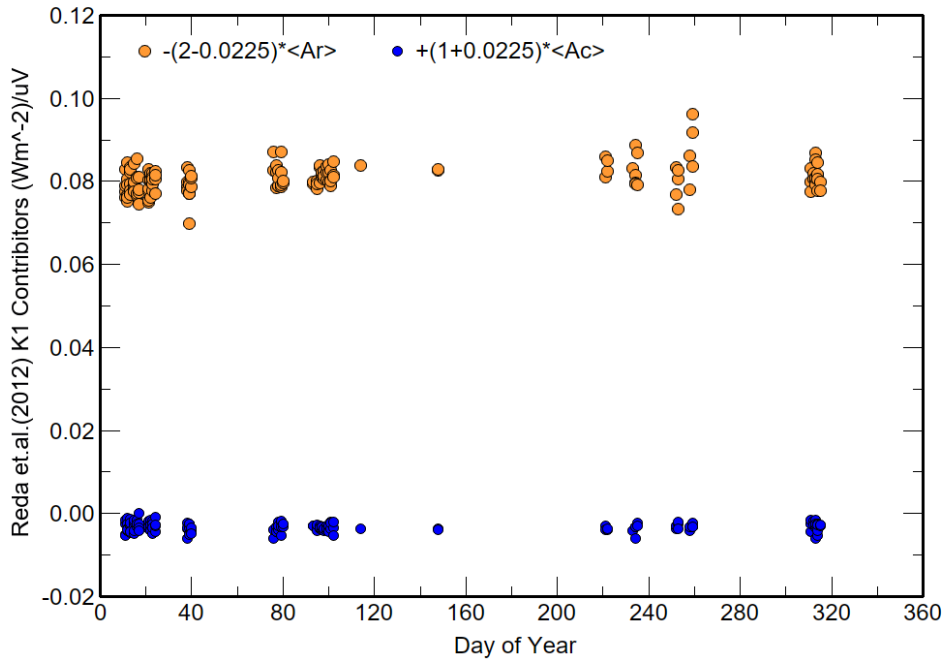
Figure11. The two slope contributions to \langle K_I \rangle for the equation developed by Reda et al., 2012.
