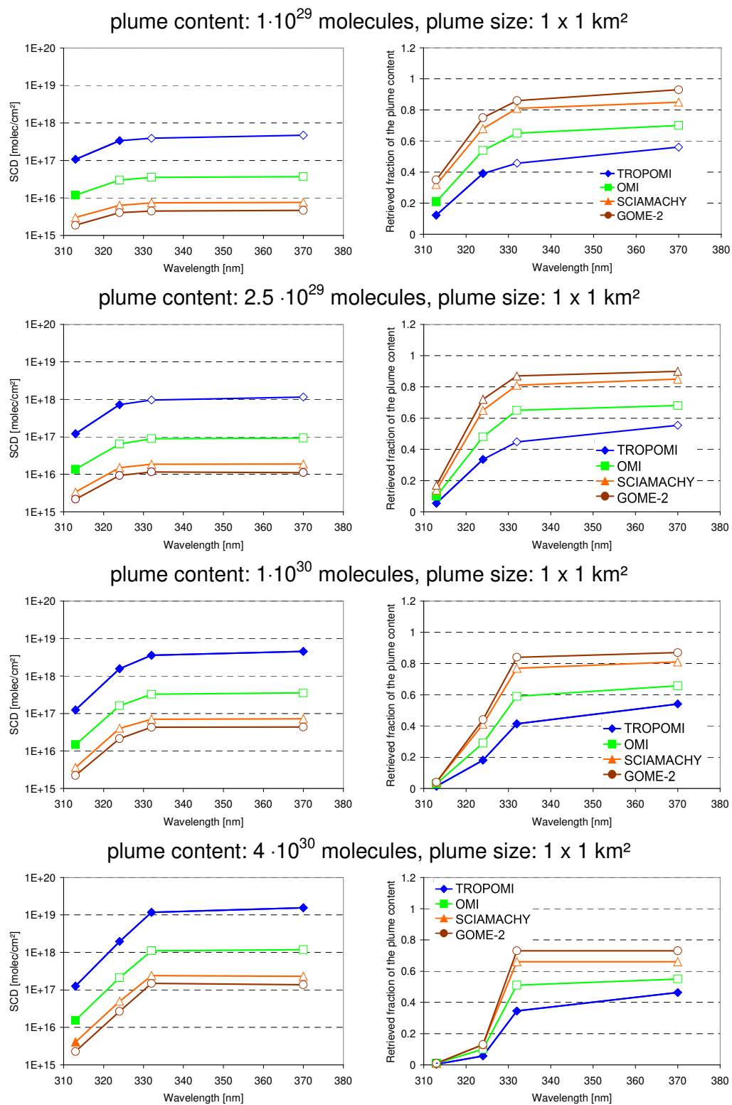
Fig. 15 Retrieved fractions of the plume content and \text{SO}_2 SCDs for different satellite instruments and for a plume size of 1 \times 1 \text{ km}^2 as function of the wavelength (plume altitude 5 – 6 km). The full symbols represent measurements with SCDs above the detection limit. Note that for the rather large ground pixel sizes of SCIAMACHY and GOME-2 the errors are between 5 and 10%. Results for other plume altitudes are shown in appendix C.
