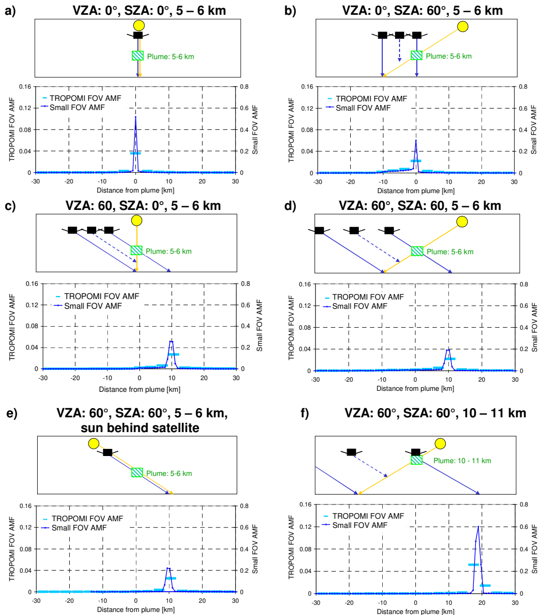
Fig. E1 AMFs for TROPOMI observations of elevated plumes for different combinations of SZA and VZA. The blue lines show the AMFs for observations with a narrow FOV (~0.014°) (right y axis); the bright blue symbols represent simulations with a TROPOMI FOV (left axis). All simulations are for SO 2 (weak) at 313 nm and plume sizes of 1 x 1 x 1 km 3 .
