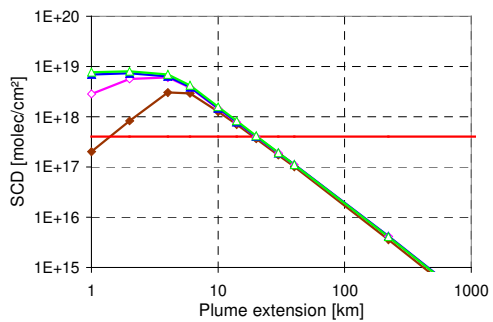
Fig. C5 Same as Fig. 14, but for additional plume heights: retrieved fraction of the plume content (top) and SO 2 SCDs (bottom) from TROPOMI measurements at different wavelengths as function of the plume size and for different amounts of molecules in the plume. The red horizontal line indicates the threshold, above which the operational SO 2 retrieval switches from the standard fit window to the first alternative fit window (at longer wavelengths).
