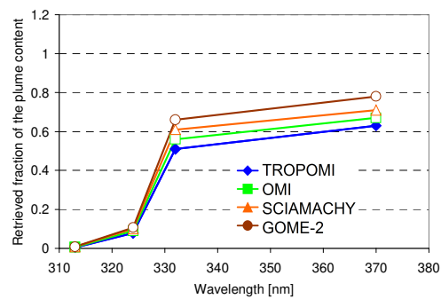
1865 Fig. C6 Same as Fig. 15, but for additional plume heights: Retrieved fractions of the plume content and SO 2 SCDs for different satellite instruments and for plume size of 1 x 1 km 2 as function of the wavelength. The full symbols represent measurements with SCDs above the detection limit. Note that for the rather large ground pixel sizes of SCIAMACHY and GOME-2 the errors are between 5 and 10%.
