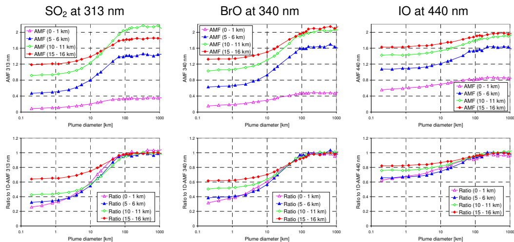
1095 Fig. 5: Dependence of the AMF on the horizontal plume extension. Top: AMFs for different plume altitudes and wavelengths; bottom: AMFs normalised by the corresponding 1D AMFs (assuming a horizontally extended plume). The simulations are performed for SZA: 0^\circ , VZA: 0^\circ , FOV: 0.014^\circ , satellite altitude: 824 km asl, no aerosols.
