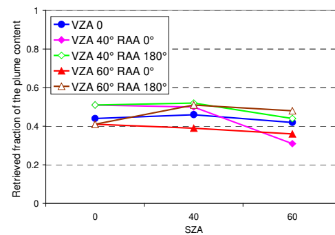
retrieved fraction of the plume content for IO (440 nm)
