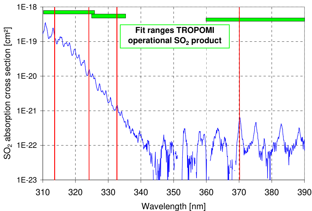
1085 Fig. 4 \text{SO}_2 absorption cross section (273K, Bogumil et al., 2000, see also https://www.iup.uni-remen.de/gruppen/molspec/databases/sciamachydata/index.html ). The green bars indicate different \text{SO}_2 fit ranges used in the operational TROPOMI product. The vertical bars indicate wavelengths used in the 3D RTM simulations.
