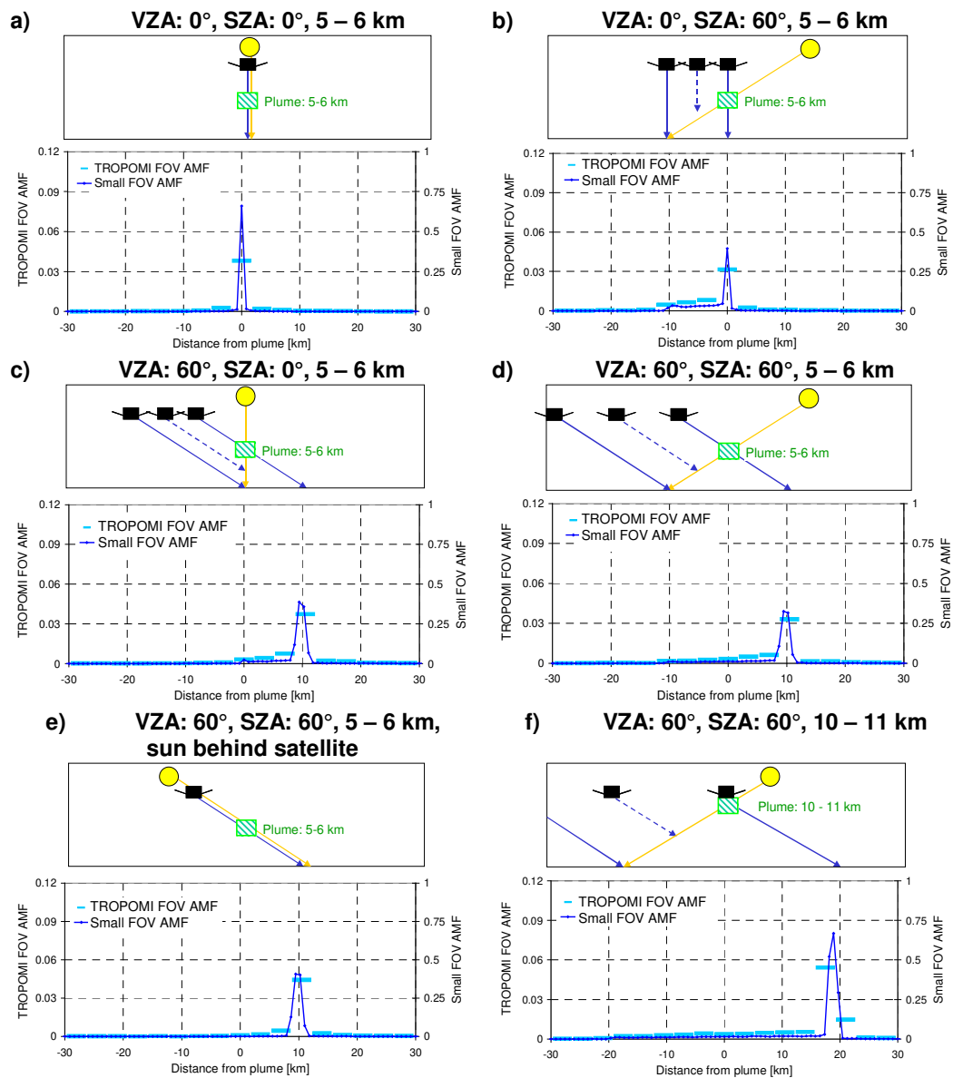
Fig. E2 AMFs for TROPOMI observations of elevated plumes for different combinations of SZA and VZA. The blue lines show the AMFs for observations with a narrow FOV (~ 0.014°) (right y axis); the bright blue symbols represent simulations with a TROPOMI FOV (left axis). All simulations are for BrO at 340 nm and plume sizes of 1 x 1 x 1 km 3 .
