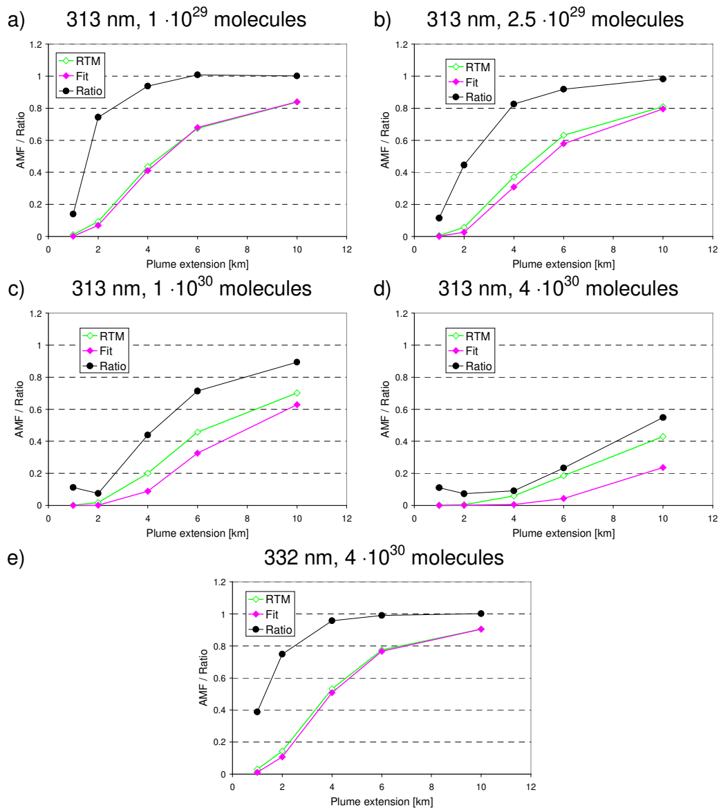
1920 Fig. D1 True AMFs (magenta lines) and monochromatic AMFs (green lines) as function of the horizontal plume extension for different SO 2 scenarios. Also the ratios of both AMFs are shown (black lines). The AMFs and AMF ratios depend on the wavelength and the SO 2 amount.
