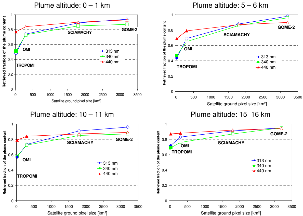
1195 Fig. 10 retrieved fraction of the plume content for different satellite sensors (for a 1 x 1 x 1 km 3 plume at different altitudes). Full symbols indicate observations above the detection limit. For the relatively large ground pixel sizes of SCIAMACHY and GOME-2 the errors are between 5 and 10%.
