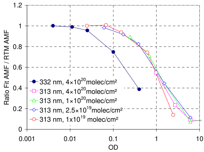
1930 Fig. D2 Ratio between true AMFs and monochromatic AMFs as function of the vertical optical depth of SO 2 in the plume.
