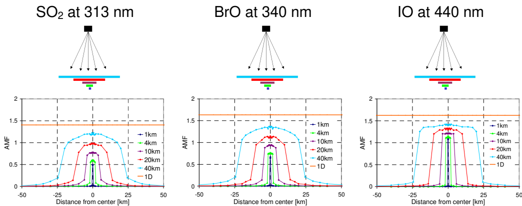
Fig. 6 AMFs for plume scans in near-nadir viewing geometry (SZA= 0^\circ , VZA= 0^\circ ) at different wavelengths. It is assumed that the satellite scans the plume with a narrow FOV ( \sim 0.014^\circ ). The different colours represent AMFs for plumes at 5-6 km altitude and with different horizontal extensions (from 1 \times 1 \text{ km}^2 to 40 \times 40 \text{ km}^2 ). Results for other plume altitudes are shown in appendix C.
