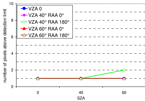
number of pixels above the detection limit for BrO (340 nm)
