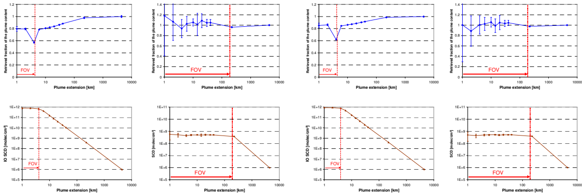
Fig. C2 Same as Fig. 8, but for additional plume heights and wavelengths: Top: Retrieved fraction of the plume content as a function of the horizontal plume extension (note the logarithmic scale). Bottom: measured trace gas SCDs (for a 1 x 1 km 2 pixel). The horizontal dashed line indicates the detection limits (see section 2.1). Left: results for a TROPOMI ground pixel; right: results for a large ground pixel of 200 x 200 km 2 . Note that in the case of plume size > ground pixel size, only the fraction of the plume within the ground pixel size is considered. Simulations for VZA=0, and SZA=0°. The error bars represent the standard deviation calculated from 40 individual simulations.
