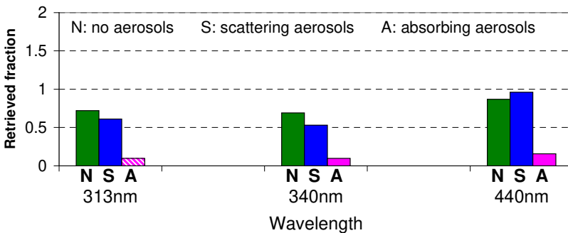
1230 Fig. 12 Retrieved fraction of the plume content at different wavelengths for different plume heights and aerosol scenarios for TROPOMI observations (horizontal plume extension 1 x 1 km 2 ). Hatched bars indicate scenarios, for which the absorption is below the detection limit for the weak trace gas scenarios described in section 2.1 (results for the satellite pixel directly above the plume).
