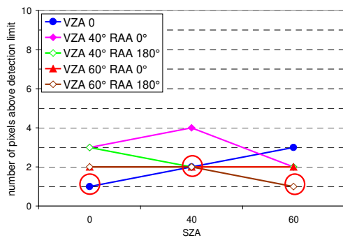
number of pixels above the detection limit for IO (440 nm)
