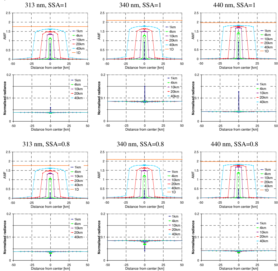
Fig. C3 Same as Fig. 11, but for additional plume heights: AMFs and normalised radiances for plume scans in near-nadir viewing geometry ( SZA=0^\circ ) for different wavelengths and aerosol contents. The satellite scans the plume with a narrow FOV ( \sim 0.014^\circ ). The different colours represent AMFs for plumes with different horizontal extensions (from 1 \times 1 \text{ km}^2 to 40 \times 40 \text{ km}^2 ). The rather low radiance at 313 nm (in spite of the high probability of Rayleigh scattering) is caused by the stratospheric ozone absorption.
