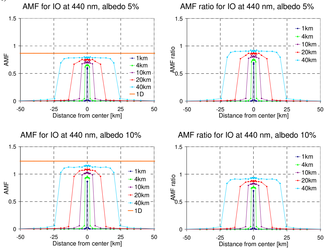
Fig. A2 AMFs (left) and corresponding ratios to the 1D-AMFs (right) for plume scans in near-nadir viewing geometry (SZA=0°, VZA=0°) for (a) SO 2 at 313 nm, (b) BrO at 340 nm, and (c) IO at 440 nm. It is assumed that the satellite scans the plume with a narrow FOV (~ 0.014°). The different colours represent AMFs for plumes at 5-6 km altitude and with different horizontal extensions (from 1 x 1 km 2 to 40 x 40 km 2 ). Results are shown for a surface albedo of 5% (as used in general in this study) and 10%. The ratios of the AMFs for narrow plumes to the corresponding 1D-AMFs hardly depend on the surface albedo.
