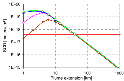
Fig. C5 Same as Fig. 14, but for additional plume heights: retrieved fraction of the plume content (top) and SO 2 SCDs (bottom) from TROPOMI measurements at different wavelengths as function of the plume size and for different amounts of molecules in the plume. The red horizontal line indicates the threshold, above which the operational SO 2 retrieval switches from the standard fit window to the first alternative fit window (at longer wavelengths).
