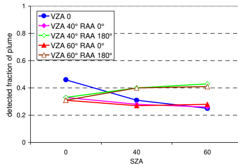
retrieved fraction of the plume content for BrO (340 nm)
