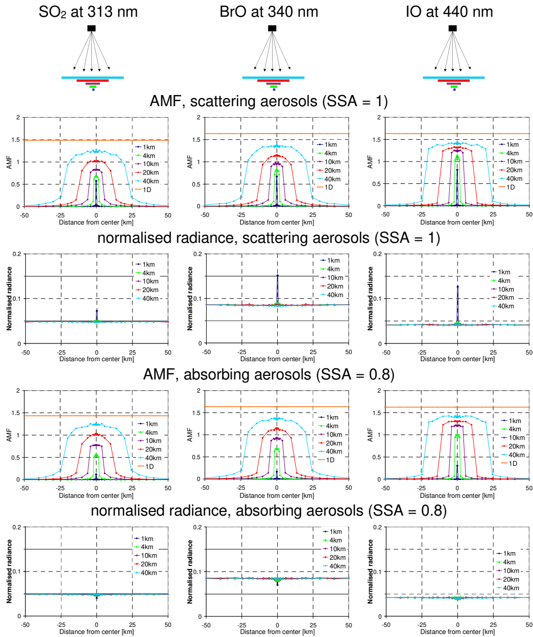
1205 Fig. 11 AMFs and normalised radiances for plume scans in near-nadir viewing geometry ( SZA=0^\circ ) for different 1210 wavelengths and aerosol contents. The satellite scans the plume with a narrow FOV ( \sim 0.014^\circ ). The different colours represent AMFs for plumes at 5 – 6 km altitude and with different horizontal extensions (from 1 x 1 km 2 to 40 x 40 km 2 ). The rather low radiance at 313 nm (in spite of the high probability of Rayleigh scattering) is caused by the stratospheric ozone absorption. Results for other plume altitudes are shown in appendix C.
