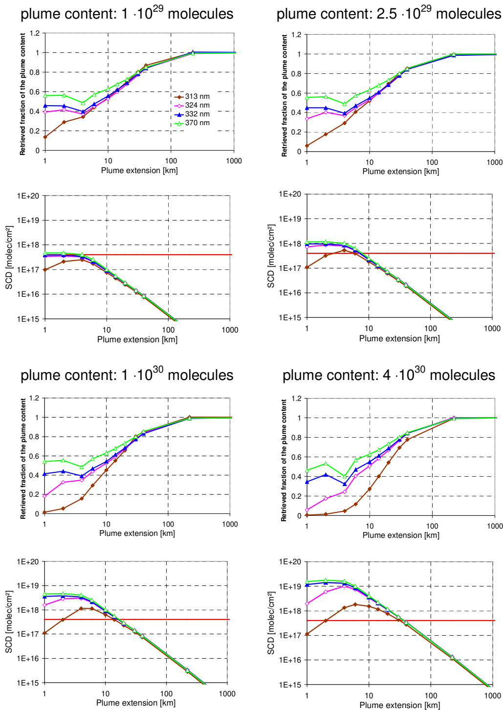
1255 Fig. 14 Retrieved fraction of the plume content (top) and SO 2 SCDs (bottom) from TROPOMI measurements at different wavelengths as function of the plume size and for different amounts of molecules in the plume (plume height: 5 – 6 km). The red horizontal line indicates the threshold, above which the operational SO 2 retrieval switches from the standard fit window to the first alternative fit window (at longer wavelengths). Results for other plume altitudes are shown in appendix C.
