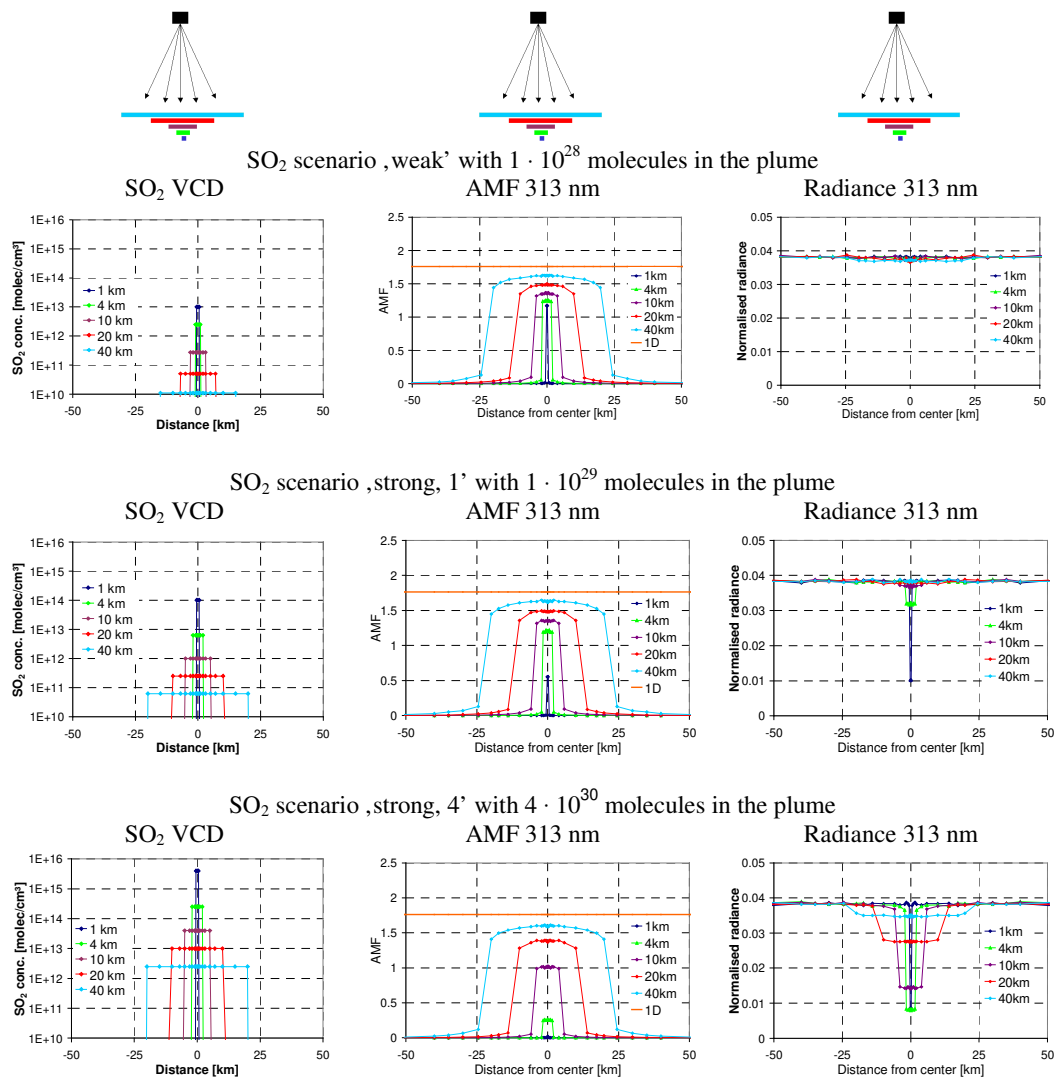
Fig. C4 Same as Fig. 13, but for additional plume heights: Plume scans for SO 2 plumes with different amounts of molecules and different horizontal extensions (for the different SO 2 scenarios, see table 3). Left: SO 2 VCDs of the plumes, middle: AMFs at 313 nm; right: normalised radiances at 313 nm.
