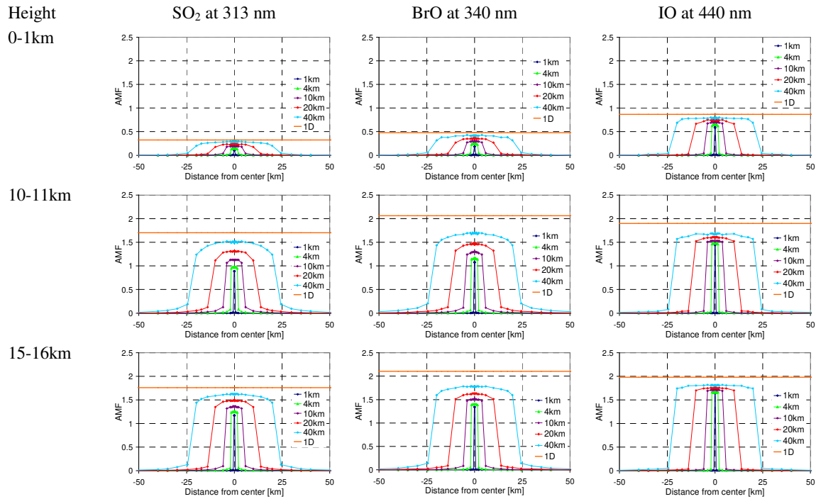
Fig. C1 Same as Fig. 5, but for additional plume heights: AMFs for plume scans in near-nadir viewing geometry (SZA=0°, VZA=0°) at different wavelengths. It is assumed that the satellite scans the plume with a narrow FOV (~0.014°). The different colours represent AMFs for plumes with different horizontal extensions (from 1 x 1 km 2 to 40 x 40 km 2 ).
