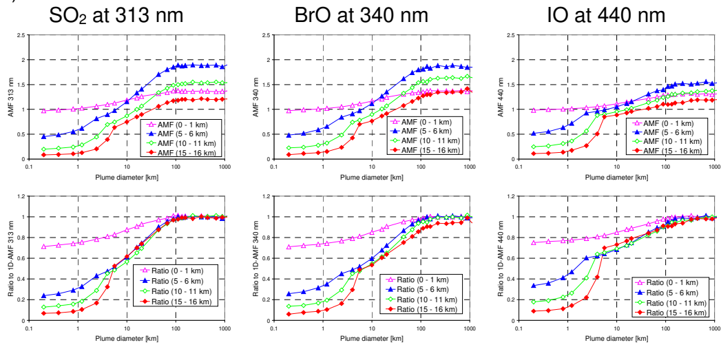
1410 Fig. 21 Dependence of the AMF on the horizontal plume extension for ground based observations (FOV: 0.014^\circ , VZA = 0^\circ , \text{SZA} = 0.3^\circ (a) and \text{SZA} = 10^\circ (b). In the upper panels the AMFs for different plume altitudes and wavelengths are shown. In the bottom panels the AMFs normalised by the corresponding 1D AMFs are shown.
