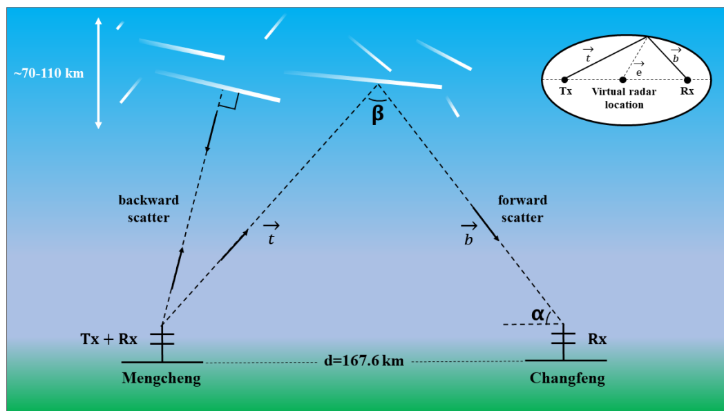
Figure 1. Schematic diagram of a backward scatter and forward scatter geometry for
