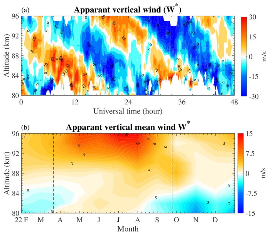
Figure R1. The vertical velocity of (a) October 16 and 17, 2021, and (b) February 1, 2022, to February 1, 2023. The thin black dashed lines in each panel present the equinoxes.
