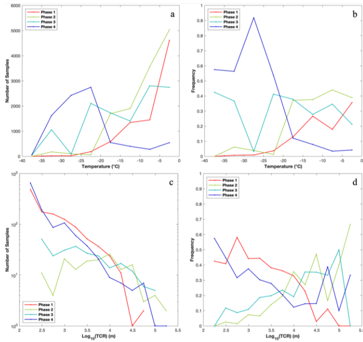
760 Figure 3. Distributions of four transition phases at various temperatures in terms of (a) number of 1-Hz samples and (b) frequency of each phase. In (b), the frequency of each phase is normalized by the number of samples of all phases in each 5-degree temperature bin. (c) Number of 1-Hz samples and (d) frequency distribution of TCR lengths in logarithmic scale. In (d), frequency is calculated as the number of 1-Hz samples of a specific phase divided by the total number of 1-Hz in-cloud samples in each 10^{0.25} bin.
