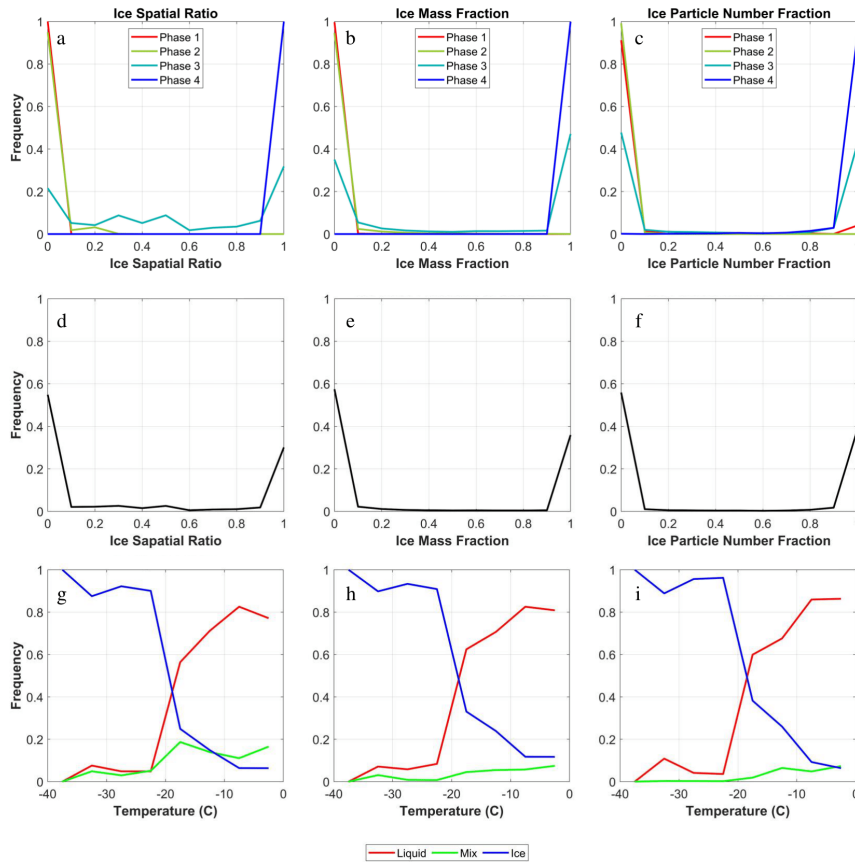
800 Figure 89. Frequency distributions of (a) ice spatial ratios calculated for individual consecutive TCR, (b) ice mass fraction per second, and (c) ice particle number fraction per second for four phases. (d-f) Similar to (a-c), but for all the phases combined representing the entire in-cloud conditions. (g-i) cloud phase frequency distributions defined based on the respective parameter in each column. Cloud phase occurrence frequencies at various temperatures. Cloud phase identification methods are based on (a) ice mass fraction per second, (b) ice particle number fraction per second, and (c) ice 805 spatial ratio calculated for individual consecutive TCR.
