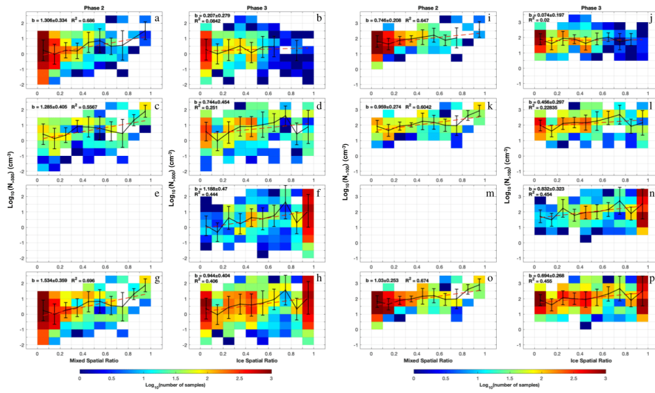
810 Figure 910. Similar to Figure 67, but showing logarithmic scale (a-h) N_{500} and (i-p) N_{100} in relation to mixed spatial ratio or ice spatial ratio, separated by the transition phase phases and cloud regions. The first, second, and third rows represent LCR, MCR, and ICR, respectively. The last row represents all cloud regions in a specific transition phase . The aerosol number concentrations represent the moving average values of every 50 seconds.
