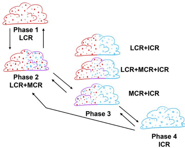
Figure 2. A conceptual diagram of the four transition phase phases for the phase exchange between supercooled liquid water and ice particles in mixed-phase clouds. Red, blue, and purple shading indicates liquid cloud region (LCR), ice cloud region (ICR) and mixed cloud region (MCR), respectively.
