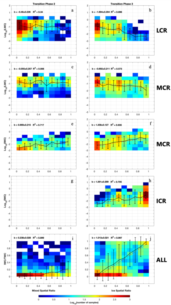
795 Figure 78. Similar to Figure 67, but showing (a-d) LWC, (e-h) IWC, and (i and j) ice mass fraction in relation to mixed spatial ratio for phase 2 and ice spatial ratio for phase 3, separated by the transition phase phases and cloud regions.
