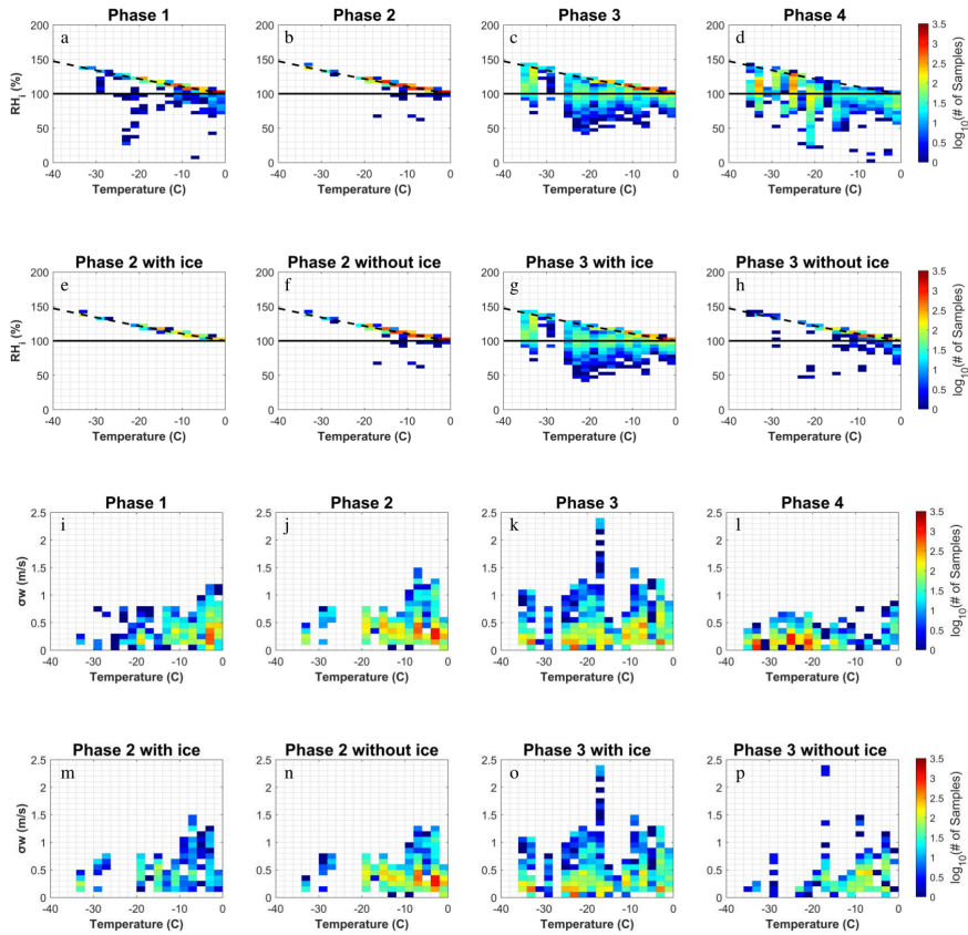
770 Figure 4. Distributions of (a-h) RH_i and (i-p) \sigma_w in various transition phase phases as a function of temperature. Dashed lines in (a) – (h) indicate liquid saturation.
