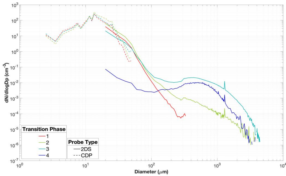
Figure 65. Particle size distribution of the four phases for mixed-phase clouds separated by probe types and temperature ranges. The entire dataset at the temperature range of -40^\circ\text{C} to 0^\circ\text{C} is shown. Phase 4 only shows 2DS measurements because ice particles measured by CDP are excluded from the analysis.
