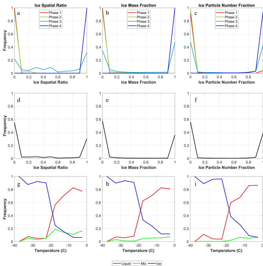
Figure 98. Frequency distributions of (a) ice spatial ratios calculated for individual consecutive TCR, (b) ice mass fraction per second, and (c) ice particle number fraction per second for four phases. (d-f) Similar to (a-c), but for all the four phases combined representing the entire in-cloud conditions. (g-i) cloud phase frequency distributions defined based on the respective parameter in each column.
