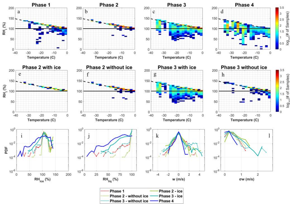
Figure 54. (a-h) Distributions of (a-h) RH i as a function of temperature. (i-l) PDFs of RH i , RH liq , vertical velocity (w) and \sigma_w in various phases, respectively as a function of temperature. Dashed lines in (a) – (h) indicate liquid saturation.
