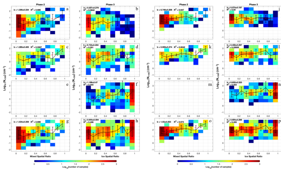
860 Figure 109. Similar to Figure 76, but showing logarithmic scale (a-h) N_{>500} and (i-p) N_{>100} in relation to mixed spatial ratio or ice spatial ratio, separated by the phases and cloud regions. The first, second, and third rows represent LCR, MCR, and ICR, respectively. The last row represents all cloud regions in a specific phase. The aerosol number concentrations represent the moving average values of every 50 seconds.
