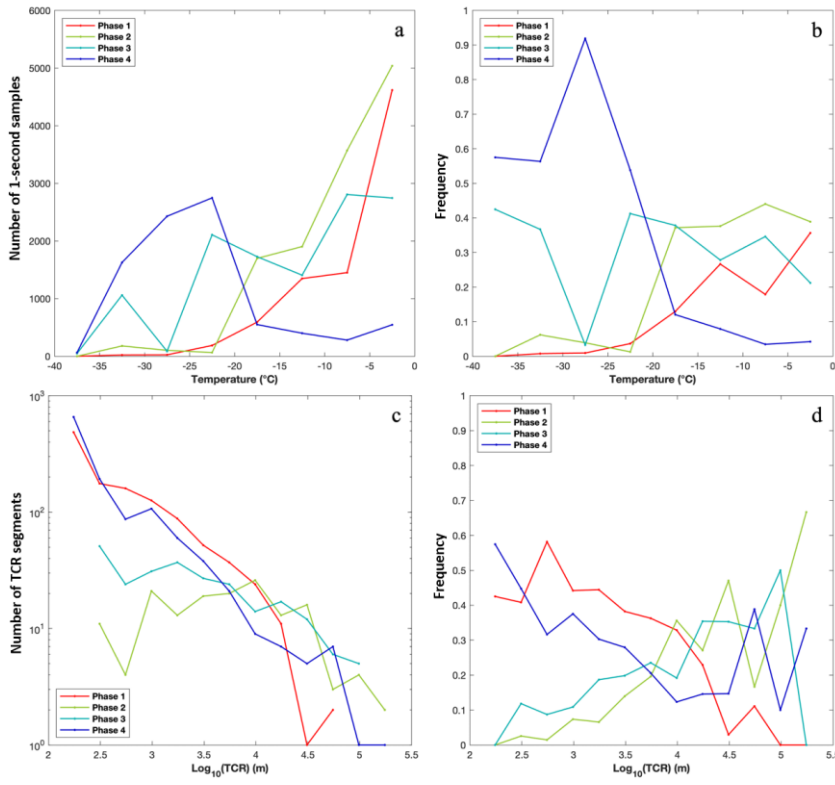
815 Figure 43. Distributions of 1-Hz samples in four phases at various temperatures in terms of the top row . (a) Number of 1-second samples and (b) frequency of 1-second samples in each phase within various temperature bins . In (b), the frequency of 1-second samples in each phase is normalized by the total number of 1-second samples of all phases in each 5-degree temperature bin. Distributions of various lengths of TCR segments are analysed in the bottom row. (c) Number of TCR segments and (d) frequency of cloud segments in each phase associated with various lengths in log 10 -scale . (e) Number of 1-Hz samples and (d) frequency distribution of TCR lengths in logarithmic scale . In (d), frequency is calculated as the number of 1-Hz samples/segments of a specific phase divided by the total number of 1-Hz in cloud samples/segments in each 10 0.25 bin. 820
