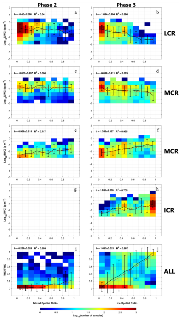
850 Figure 87. Similar to Figure 76, but showing (a-d) LWC (unit: \text{g m}^{-3} ), (e-h) IWC (unit: \text{g m}^{-3} ), and (i and j) ice mass fraction in relation to mixed spatial ratio for phase 2 and ice spatial ratio for phase 3, separated by the phase types and cloud regions.
