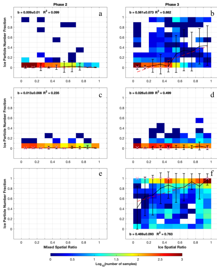
Figure 76. Relationship between ice particle number fraction (IPNF) and mixed spatial ratio or ice spatial ratio, separated by the phase types (phase 2 in column 1 and phase 3 in column 2), and by various cloud segments – (a, b) LCR, (c, d) MCR and (e, f) ICR. Average values for each ice spatial ratio bin are shown in black solid lines, with vertical bars representing standard deviations. Linear fit is shown in red dashed line. Average values of generating cells (time series obtained from Wang et al. (2020)) are in pink “X” markers. The slope value b , its associated standard deviation, and the ordinary R-squared value are shown in the legend.
