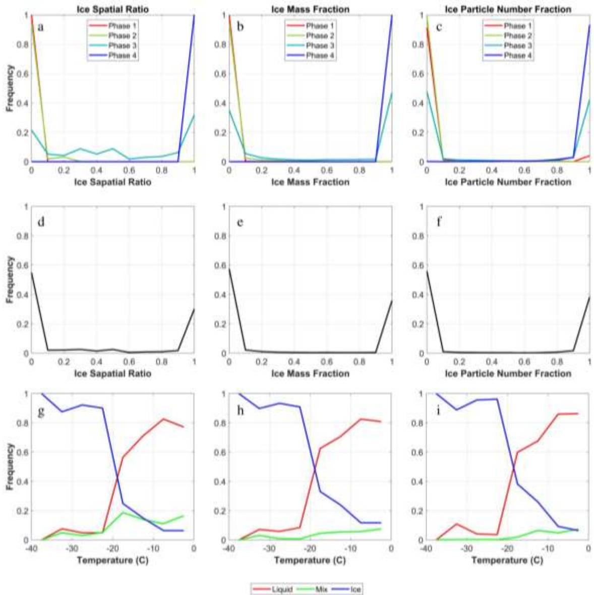
Figure 9. Frequency distributions of (a) ice spatial ratios calculated for individual consecutive TCR, (b) ice mass fraction per second, and (c) ice particle number fraction IPNF per second for four phases. (d-f) Similar to (a-c), but for the four phases combined representing the entire in-cloud conditions. (g-i) cloud phase frequency distributions defined based on the respective parameter in each column.
