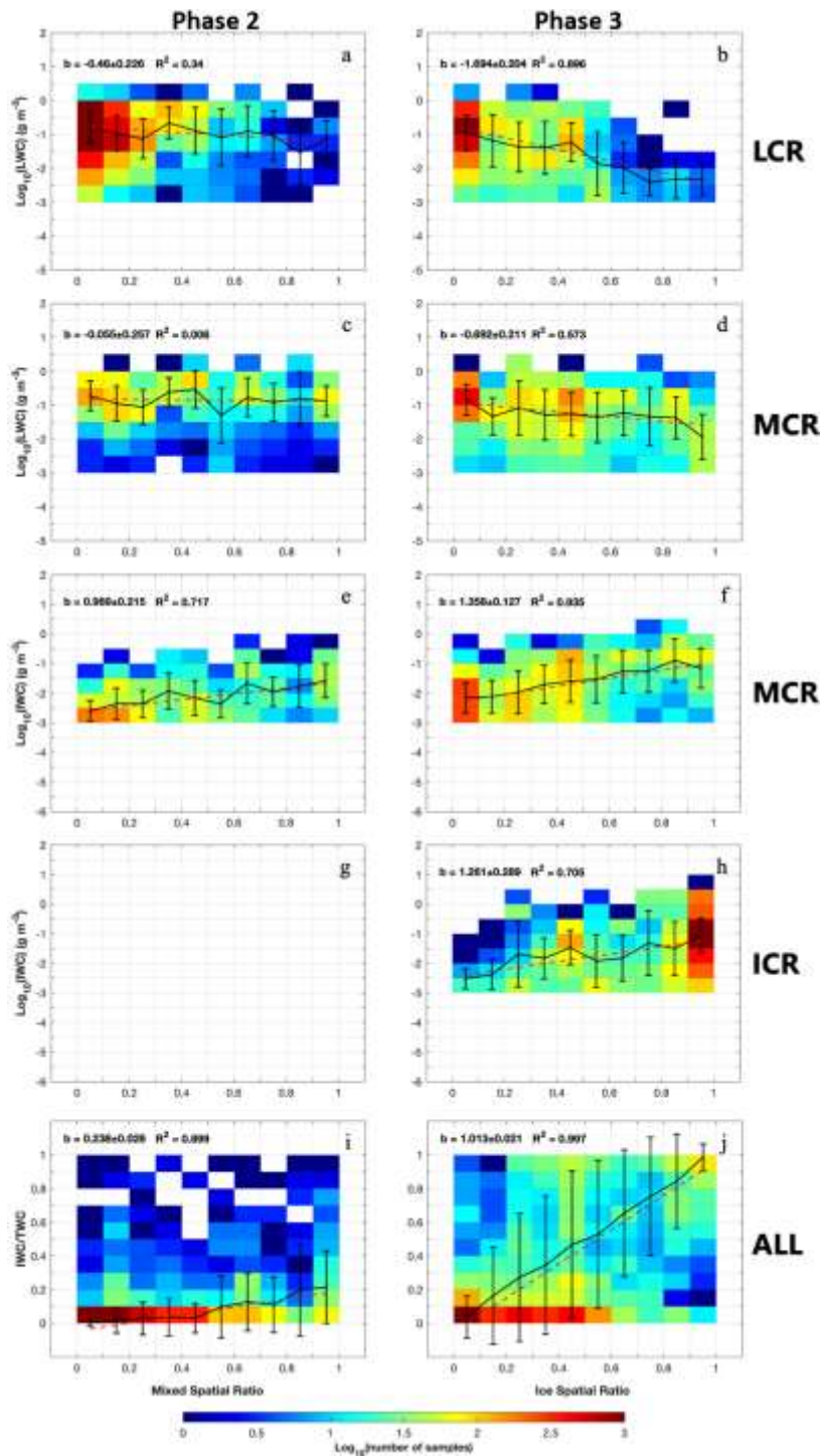
Figure 8. Similar to Figure 7, but showing (a-d) LWC (unit: \text{g m}^{-3} ), (e-h) IWC (unit: \text{g m}^{-3} ), and (i and j) ice mass fraction in relation to mixed spatial ratio for phase 2 and ice spatial ratio for phase 3, separated by the phase type and cloud regions.
