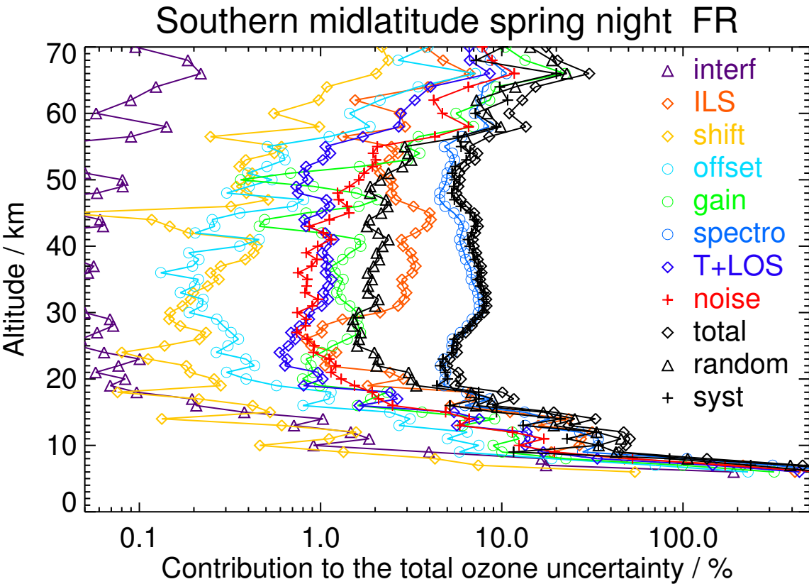
Figure S22. V8H_O3_61 Southern midlatitude spring night
