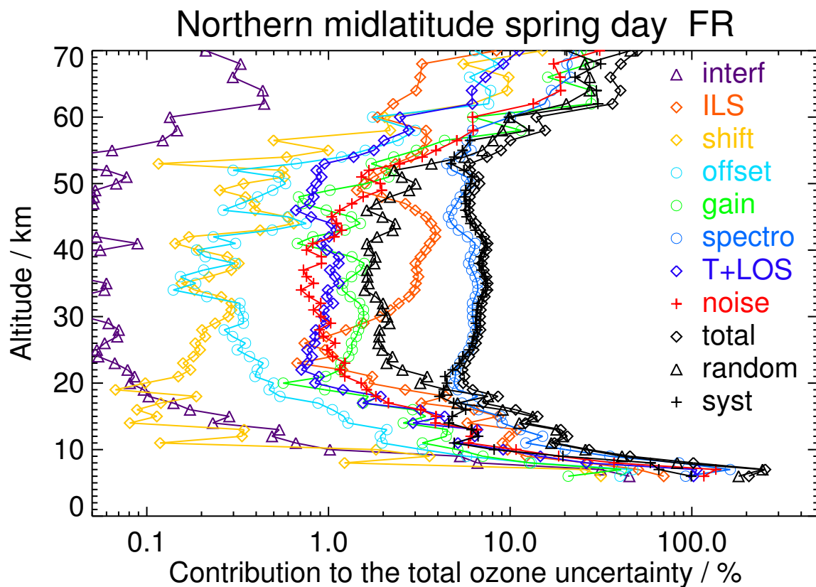
Figure S11. V8H_O3_61 Northern midlatitude spring day
