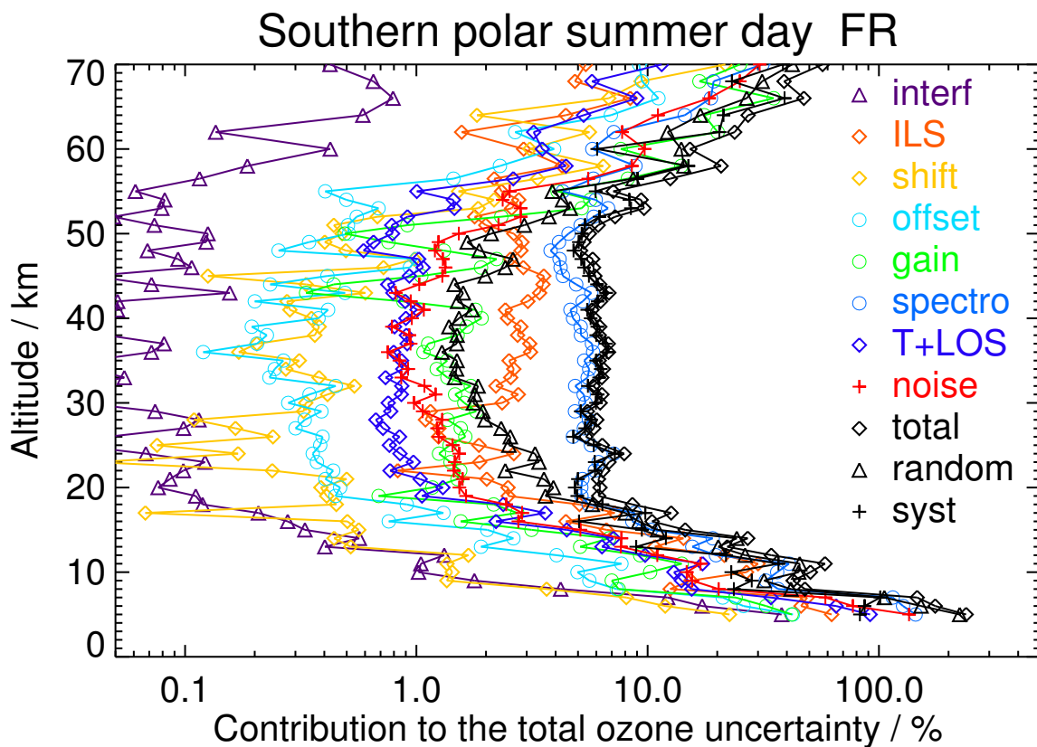
Figure S31. V8H_O3_61 Southern polar summer day
