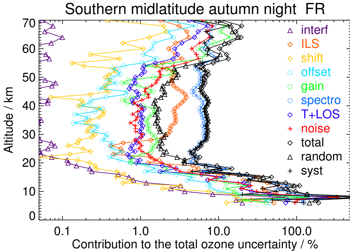
Figure S26. V8H_O3_61 Southern midlatitude autumn night
