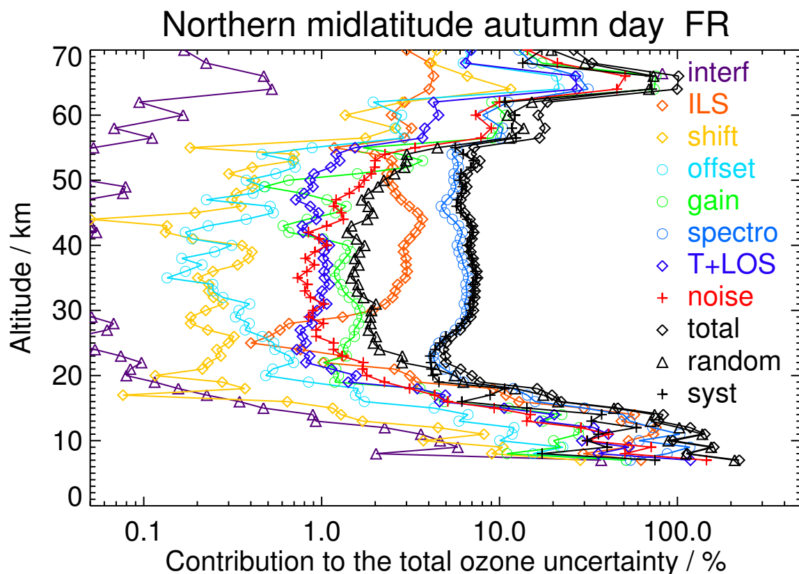
Figure S15. V8H_O3_61 Northern midlatitude autumn day
