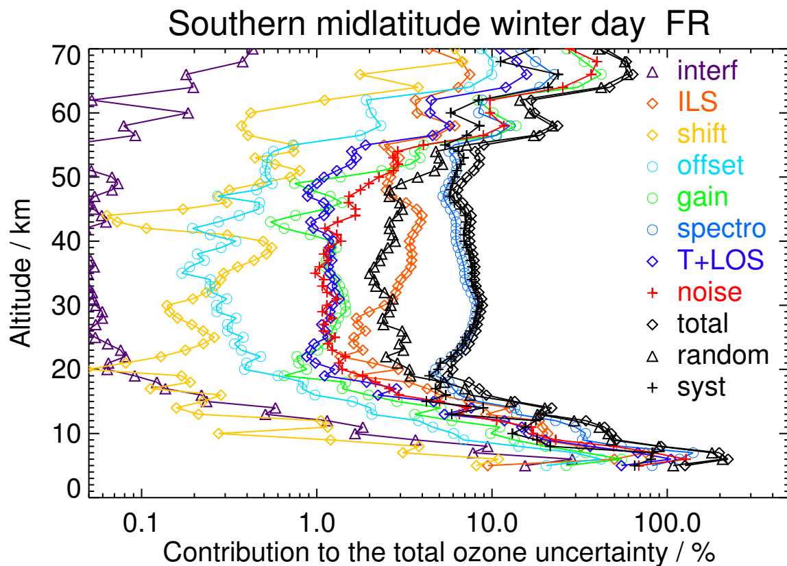
Figure S19. V8H_O3_61 Southern midlatitude winter day
