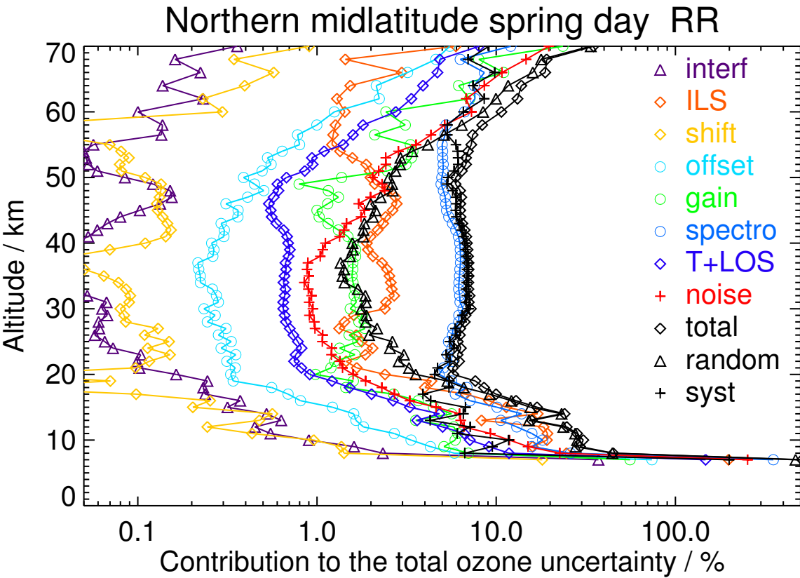
Figure S45. V8R_O3_261 Northern midlatitude spring day
