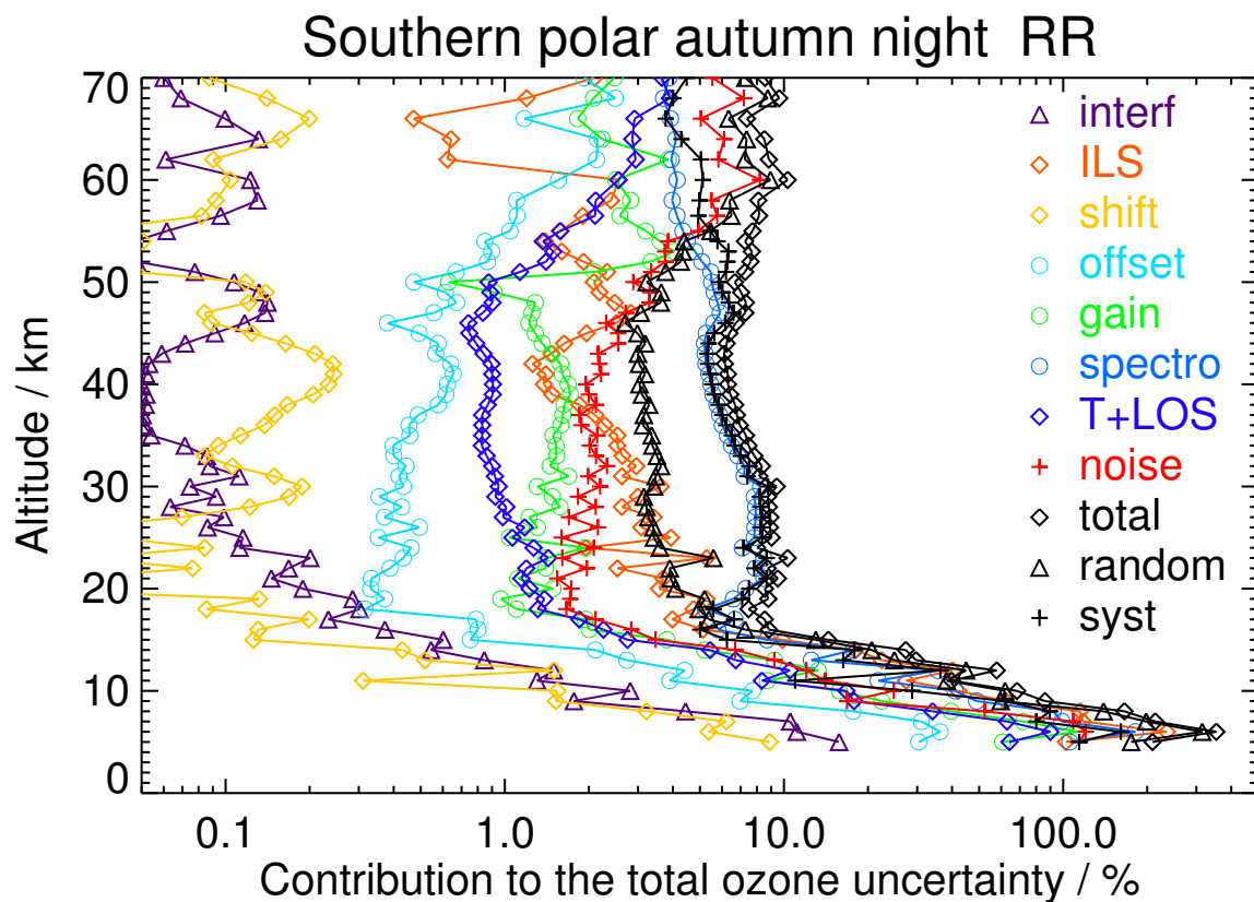
Figure S68. V8R_O3_261 Southern polar autumn night
