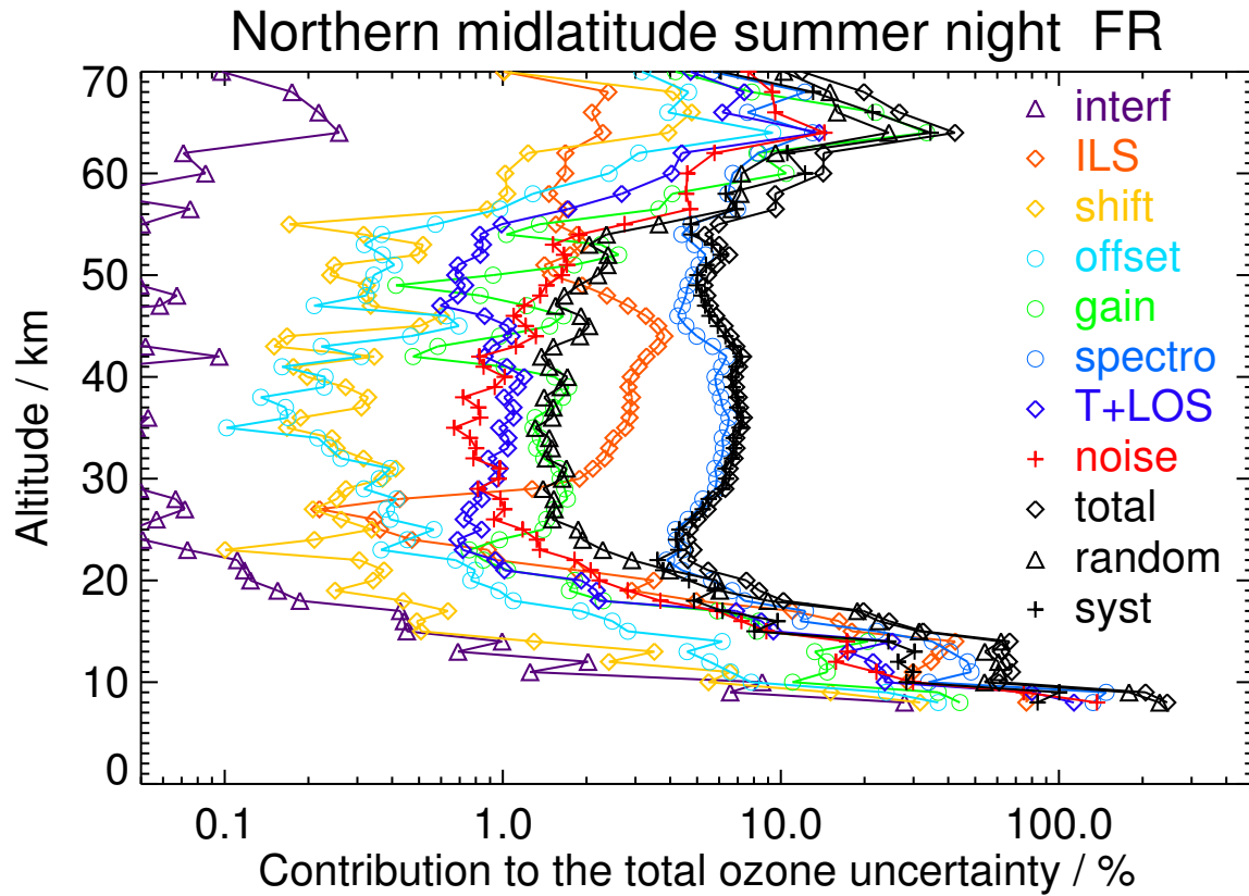
Figure S14. V8H_O3_61 Northern midlatitude summer night
