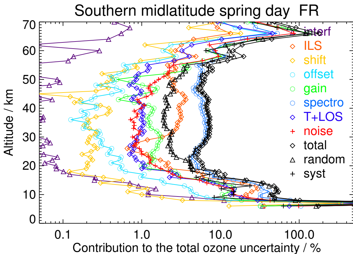
Figure S21. V8H_O3_61 Southern midlatitude spring day
