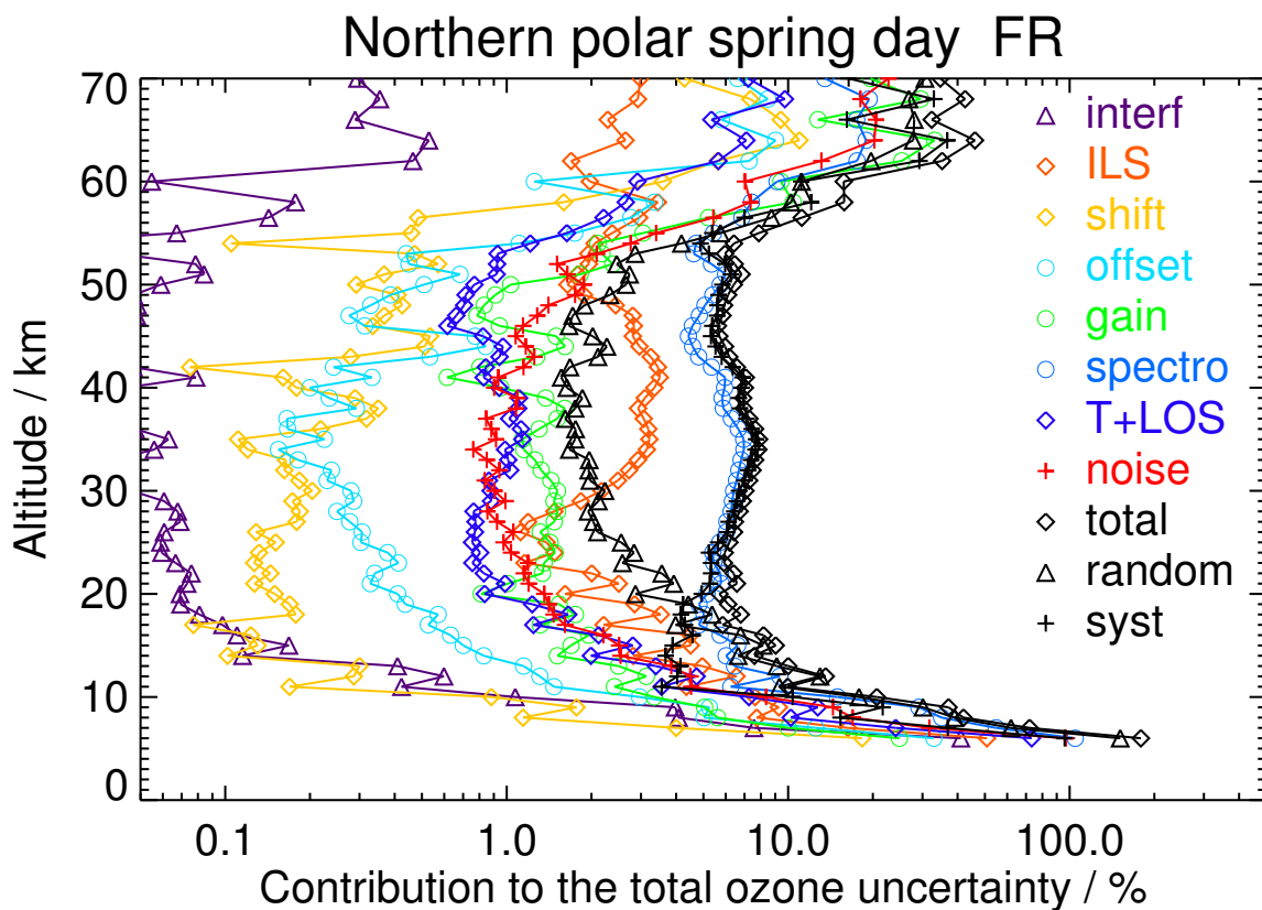
Figure S3. V8H_O3_61 Northern polar spring day
