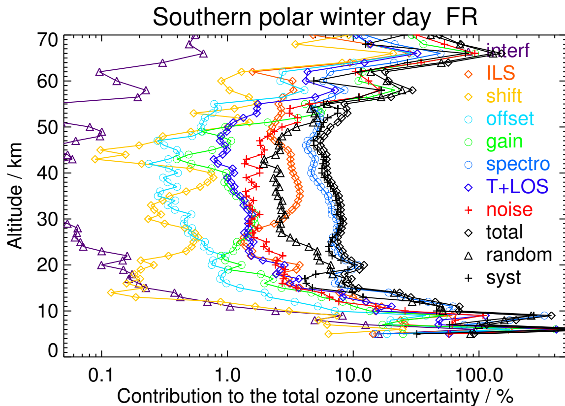
Figure S27. V8H_O3_61 Southern polar winter day
