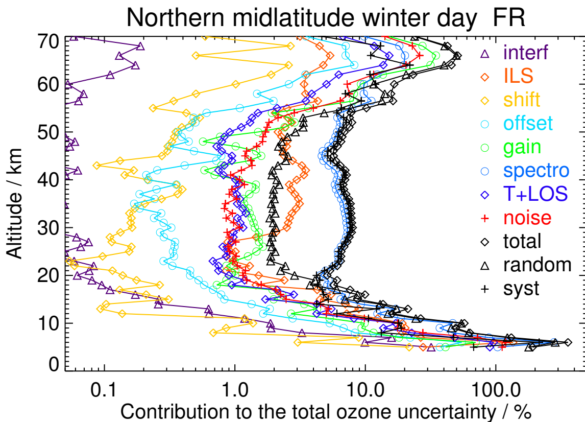
Figure S9. V8H_O3_61 Northern midlatitude winter day
