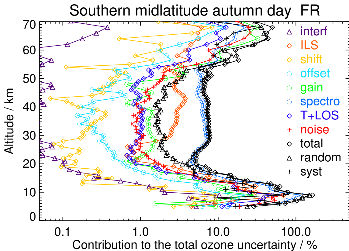
Figure S25. V8H_O3_61 Southern midlatitude autumn day
