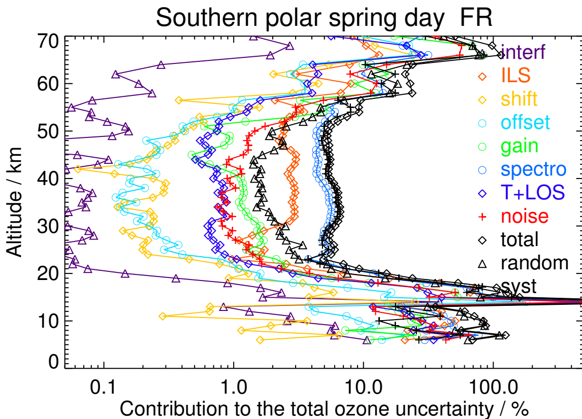
Figure S29. V8H_O3_61 Southern polar spring day
