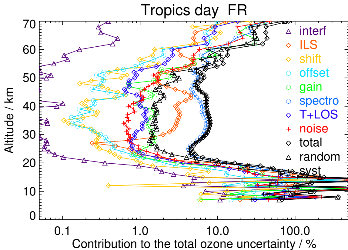
Figure S17. V8H_O3_61 Tropics day
