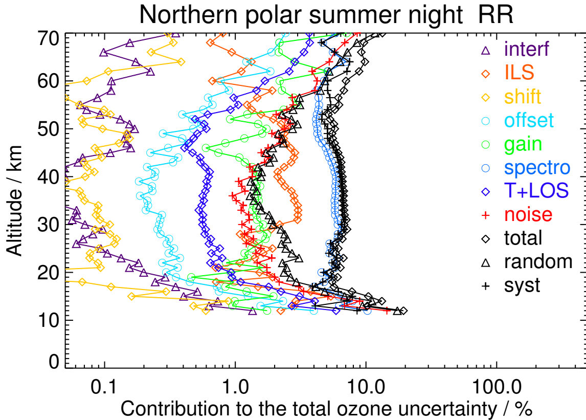
Figure S40. V8R_O3_261 Northern polar summer night
