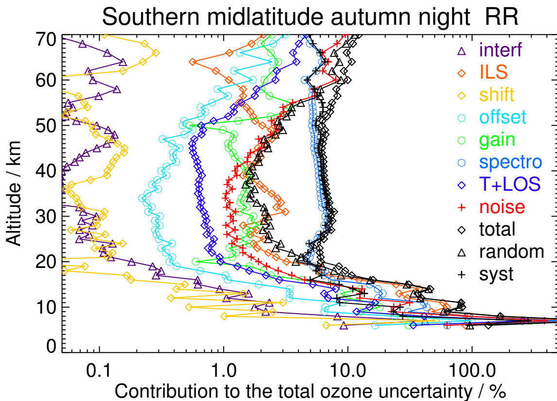
Figure S60. V8R_O3_261 Southern midlatitude autumn night
