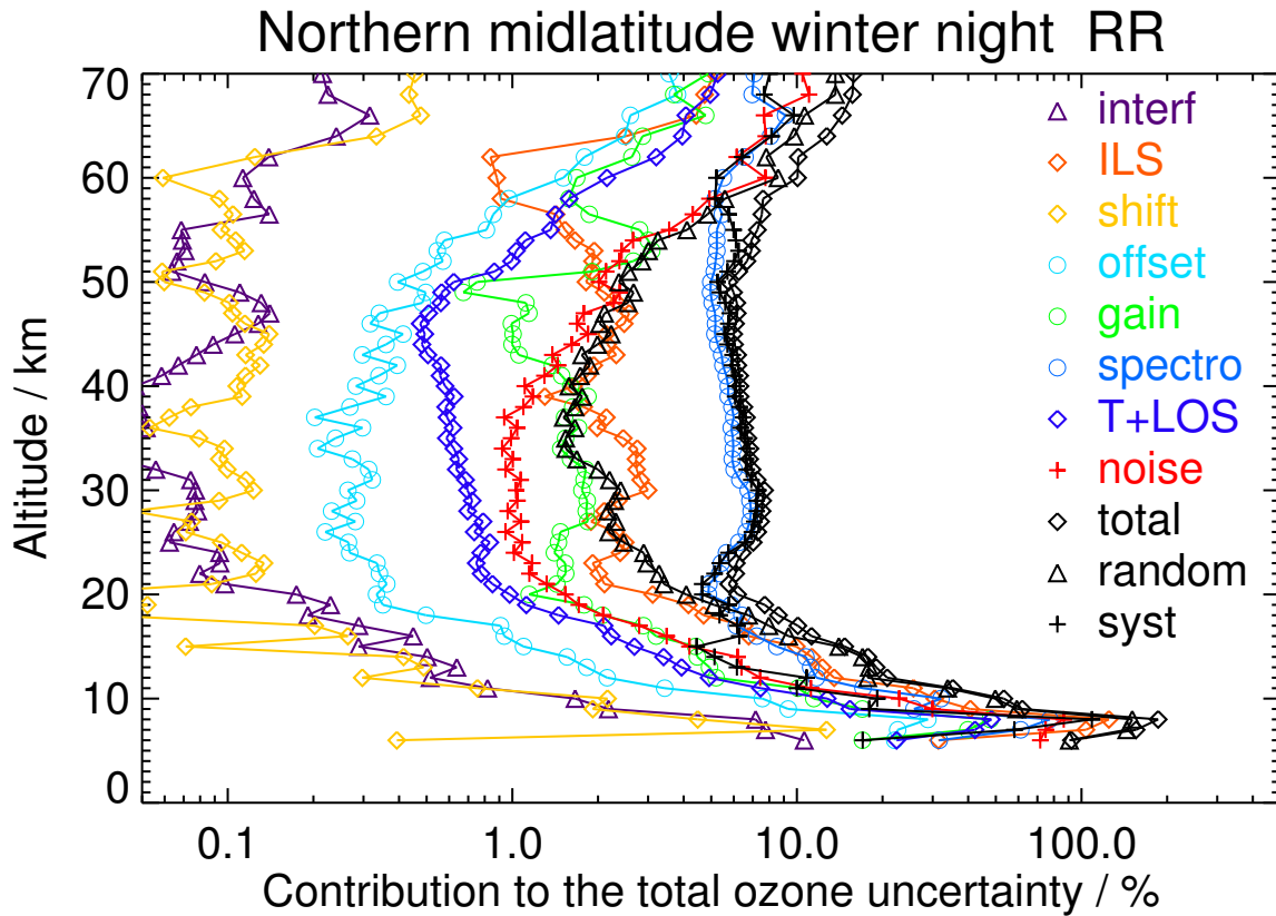
Figure S44. V8R_O3_261 Northern midlatitude winter night
