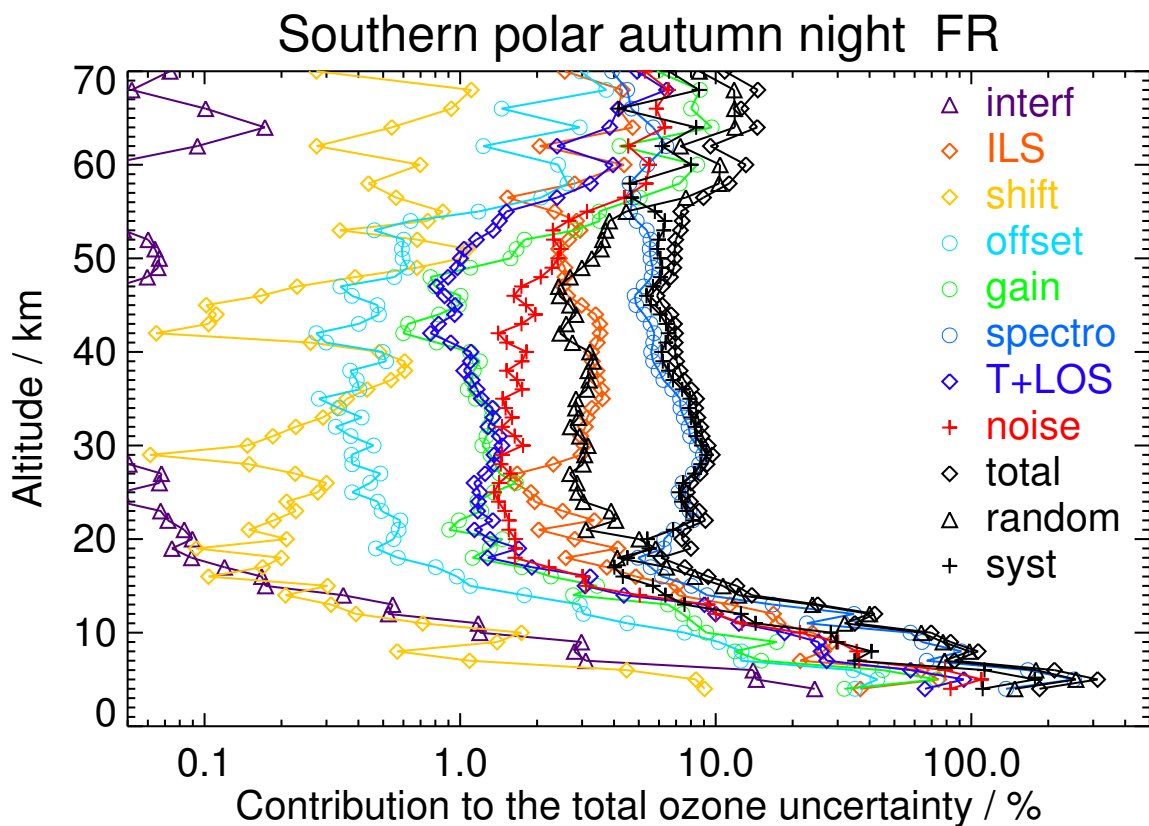
Figure S34. V8H_O3_61 Southern polar autumn night
