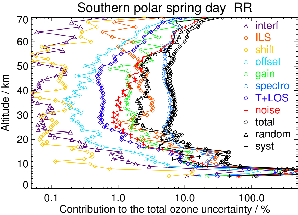
Figure S63. V8R_O3_261 Southern polar spring day
