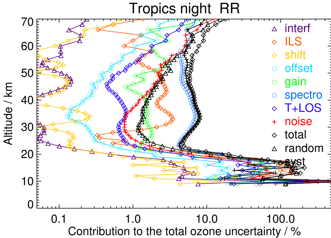
Figure S52. V8R_O3_261 Tropics night
