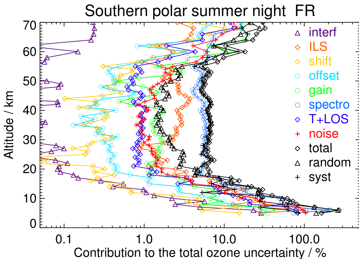
Figure S32. V8H_O3_61 Southern polar summer night
