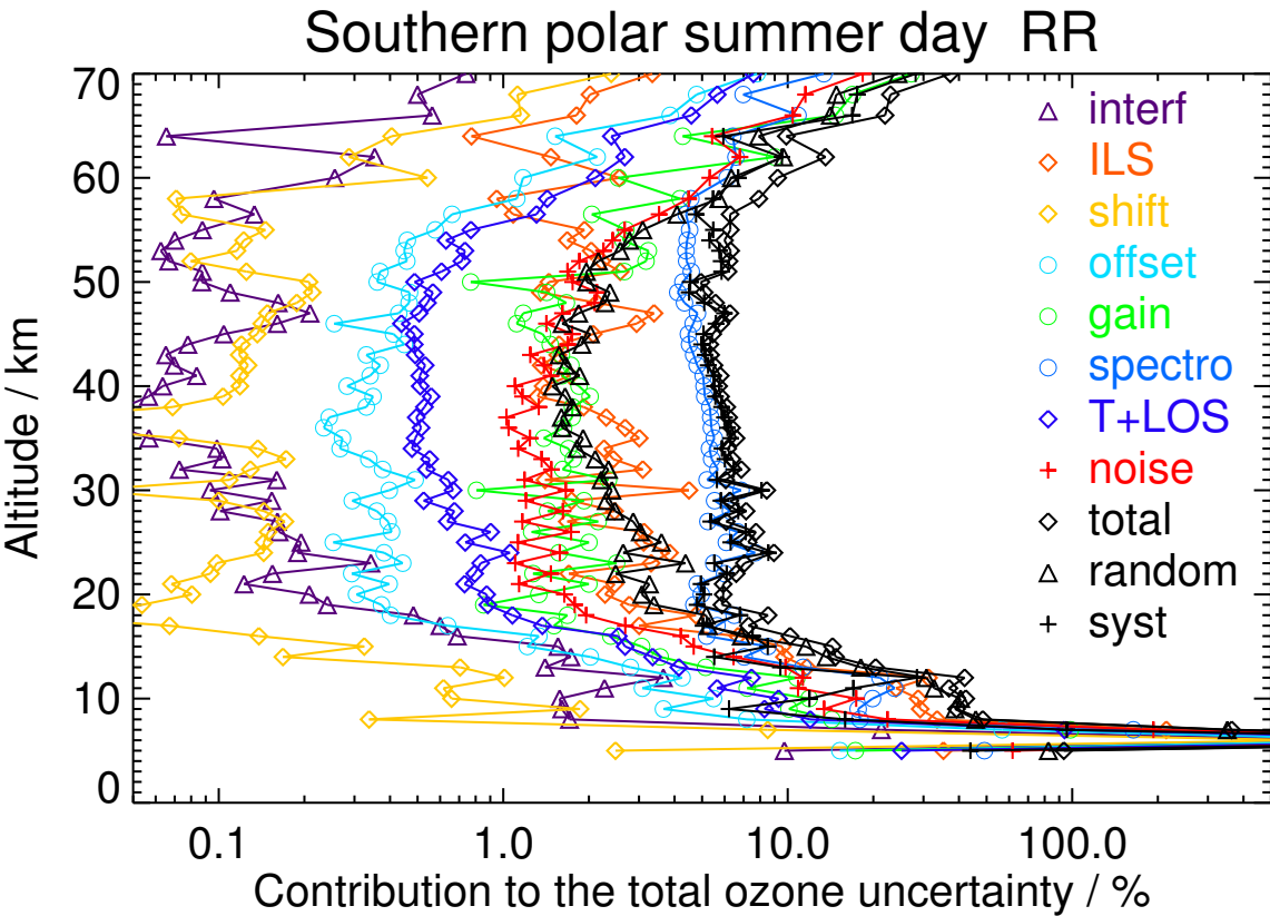
Figure S65. V8R_O3_261 Southern polar summer day
