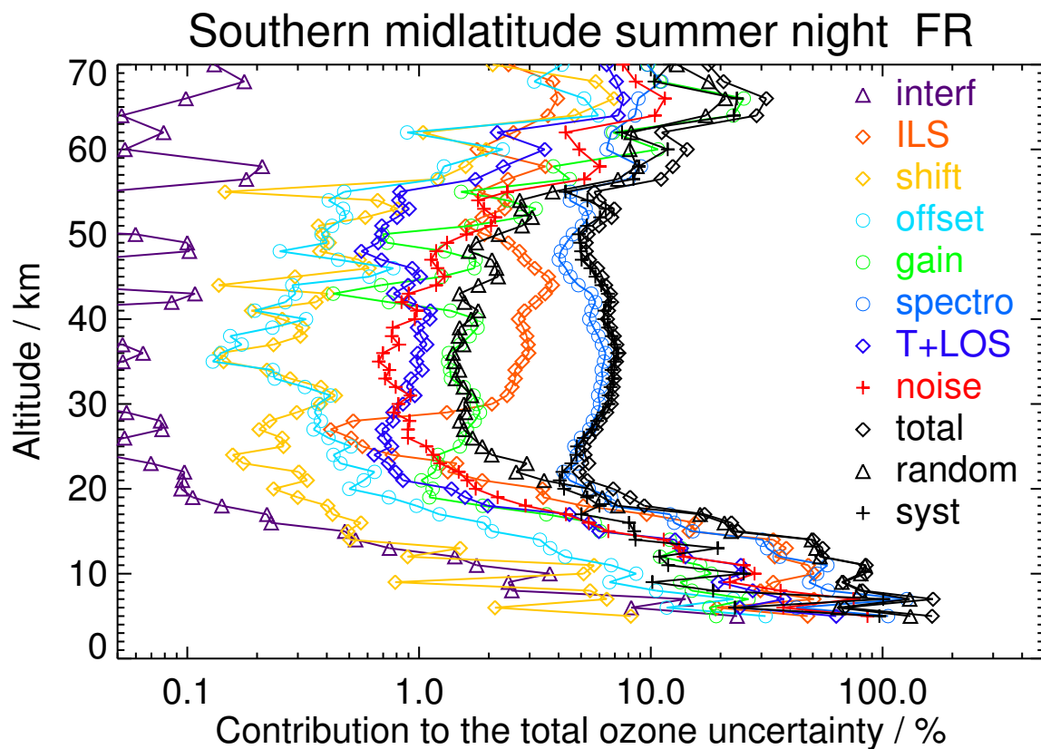
Figure S24. V8H_O3_61 Southern midlatitude summer night
