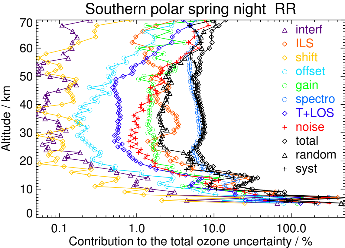
Figure S64. V8R_O3_261 Southern polar spring night
