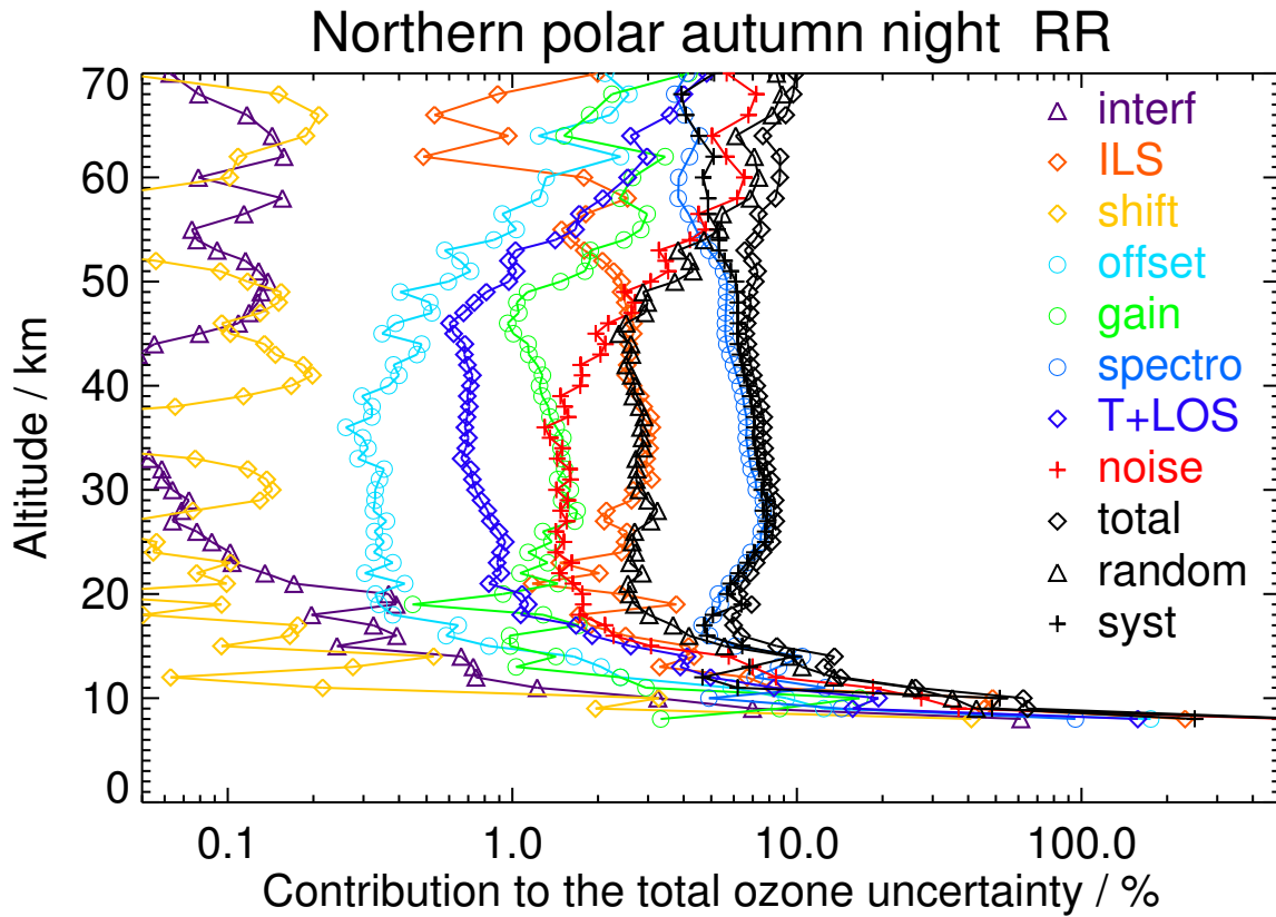
Figure S42. V8R_O3_261 Northern polar autumn night
