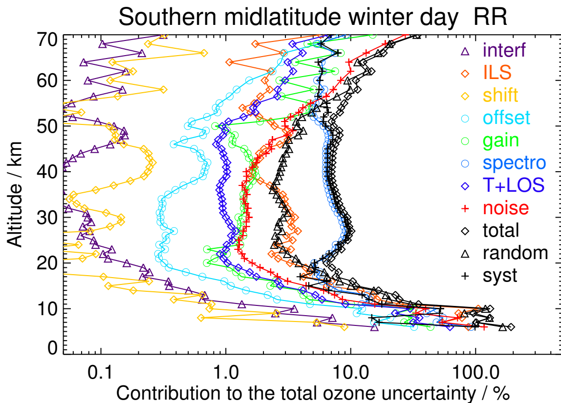
Figure S53. V8R_O3_261 Southern midlatitude winter day
