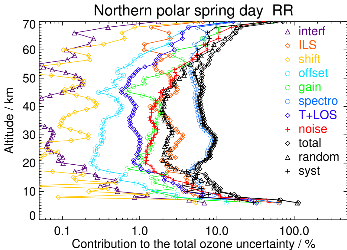
Figure S37. V8R_O3_261 Northern polar spring day
