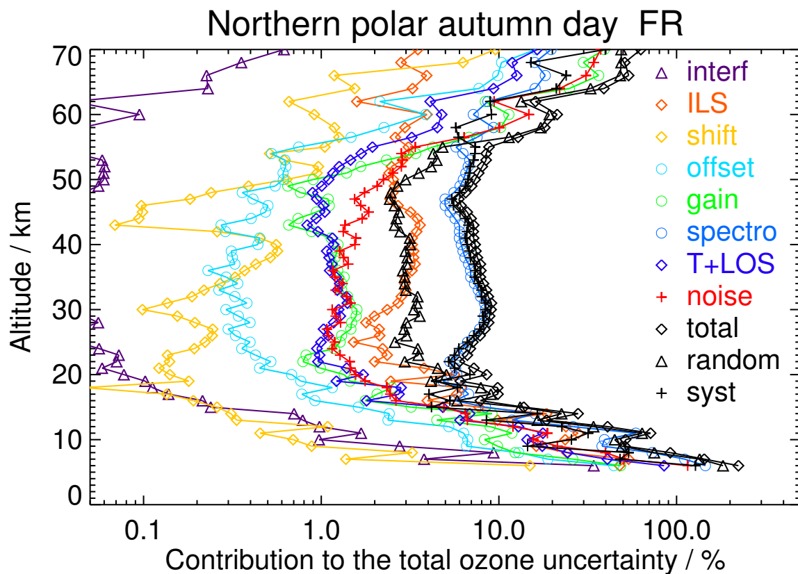
Figure S7. V8H_O3_61 Northern polar autumn day
