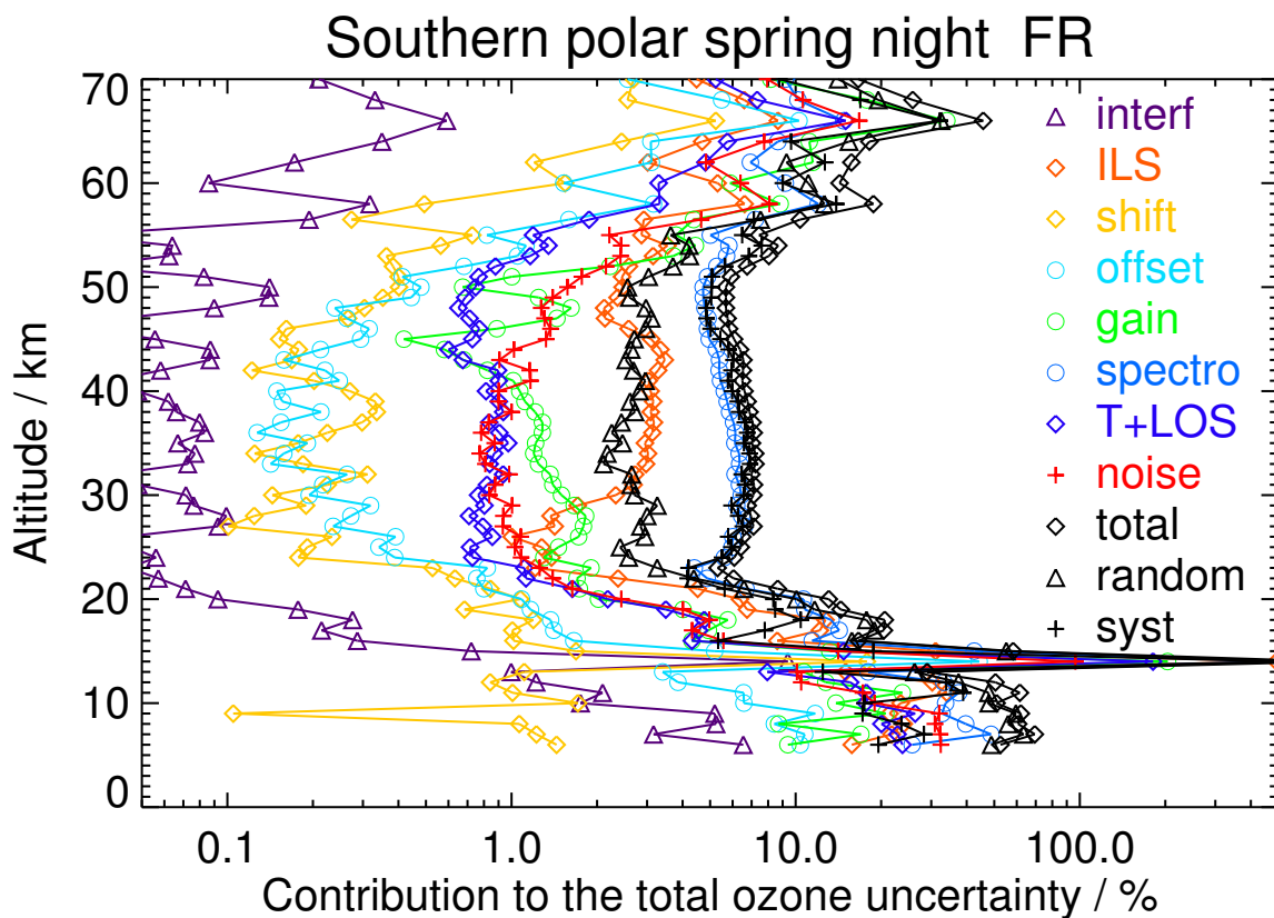
Figure S30. V8H_O3_61 Southern polar spring night
