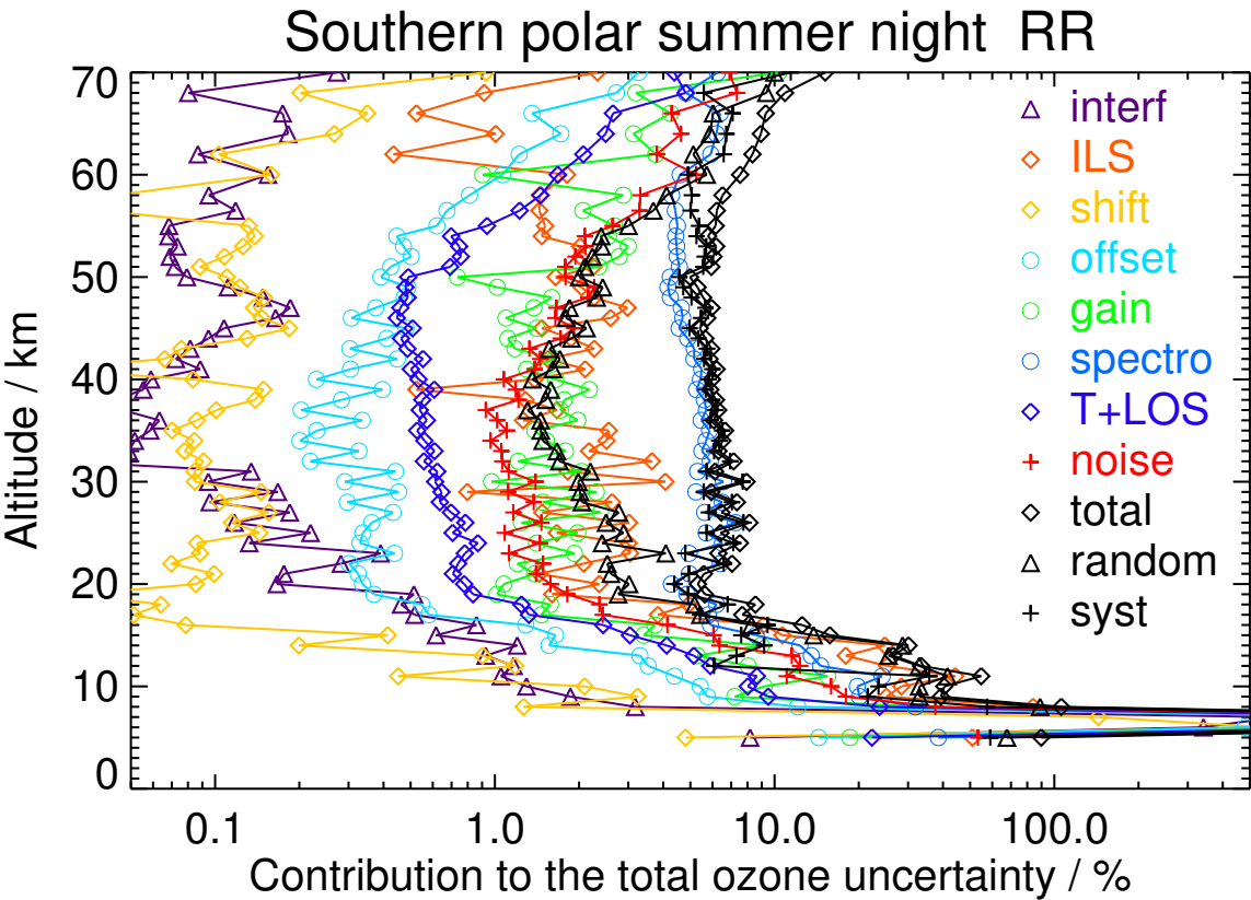
Figure S66. V8R_O3_261 Southern polar summer night
