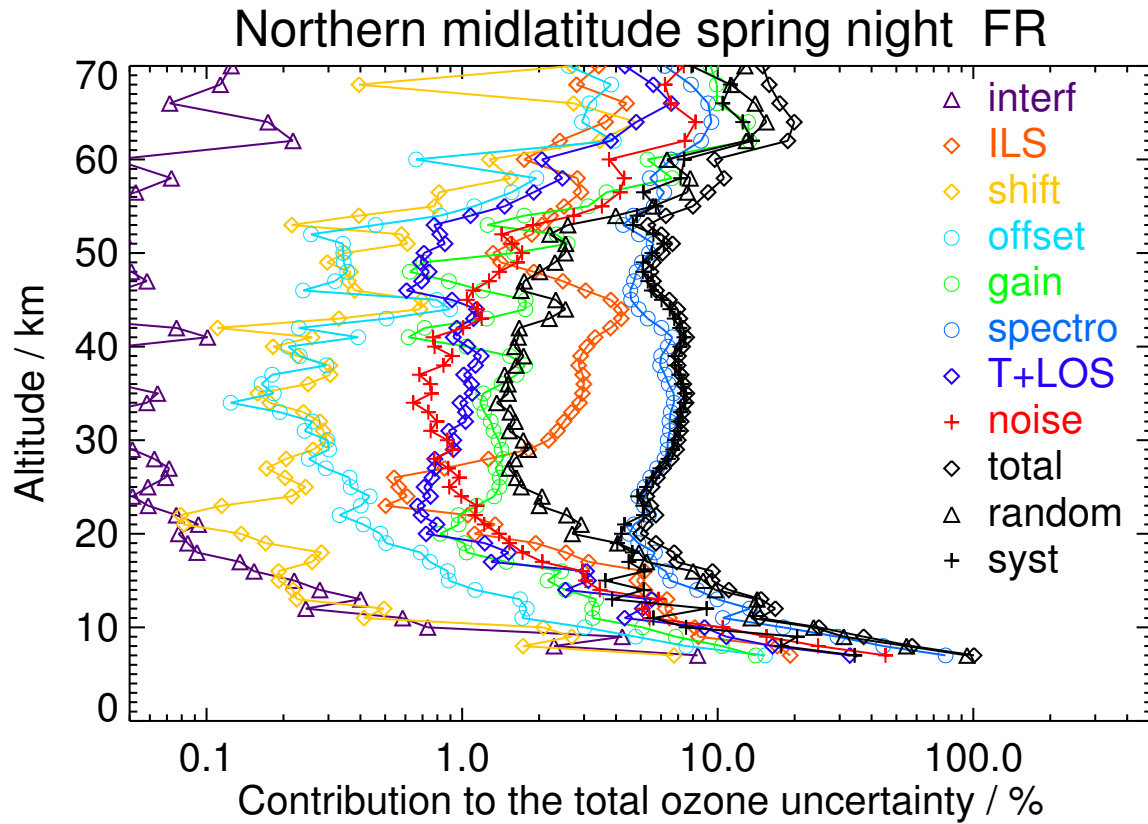
Figure S12. V8H_O3_61 Northern midlatitude spring night
