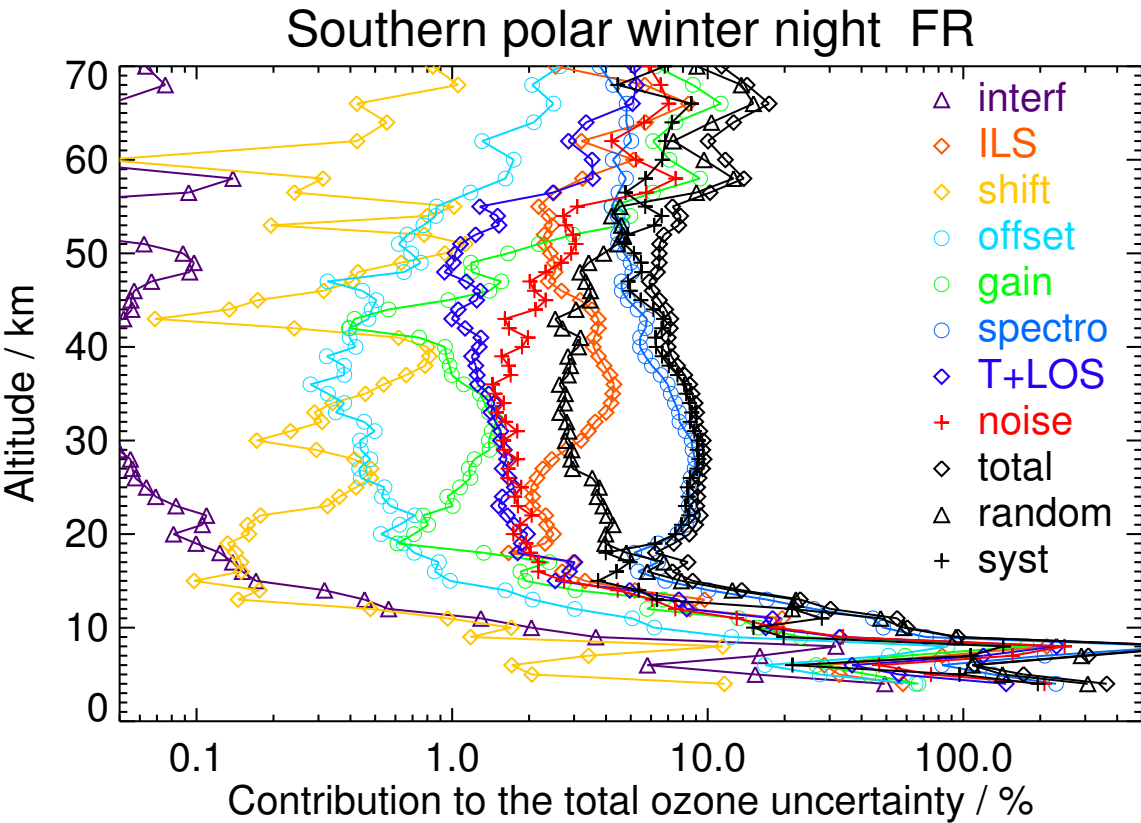
Figure S28. V8H_O3_61 Southern polar winter night
