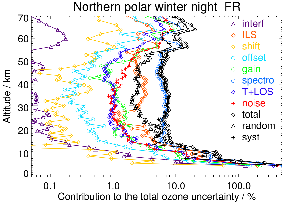
Figure S2. V8H_O3_61 Northern polar winter night
