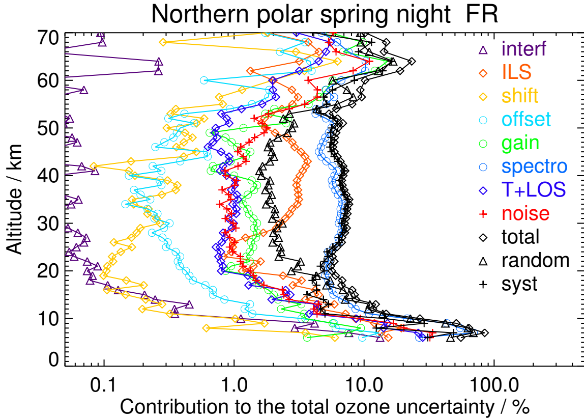
Figure S4. V8H_O3_61 Northern polar spring night
