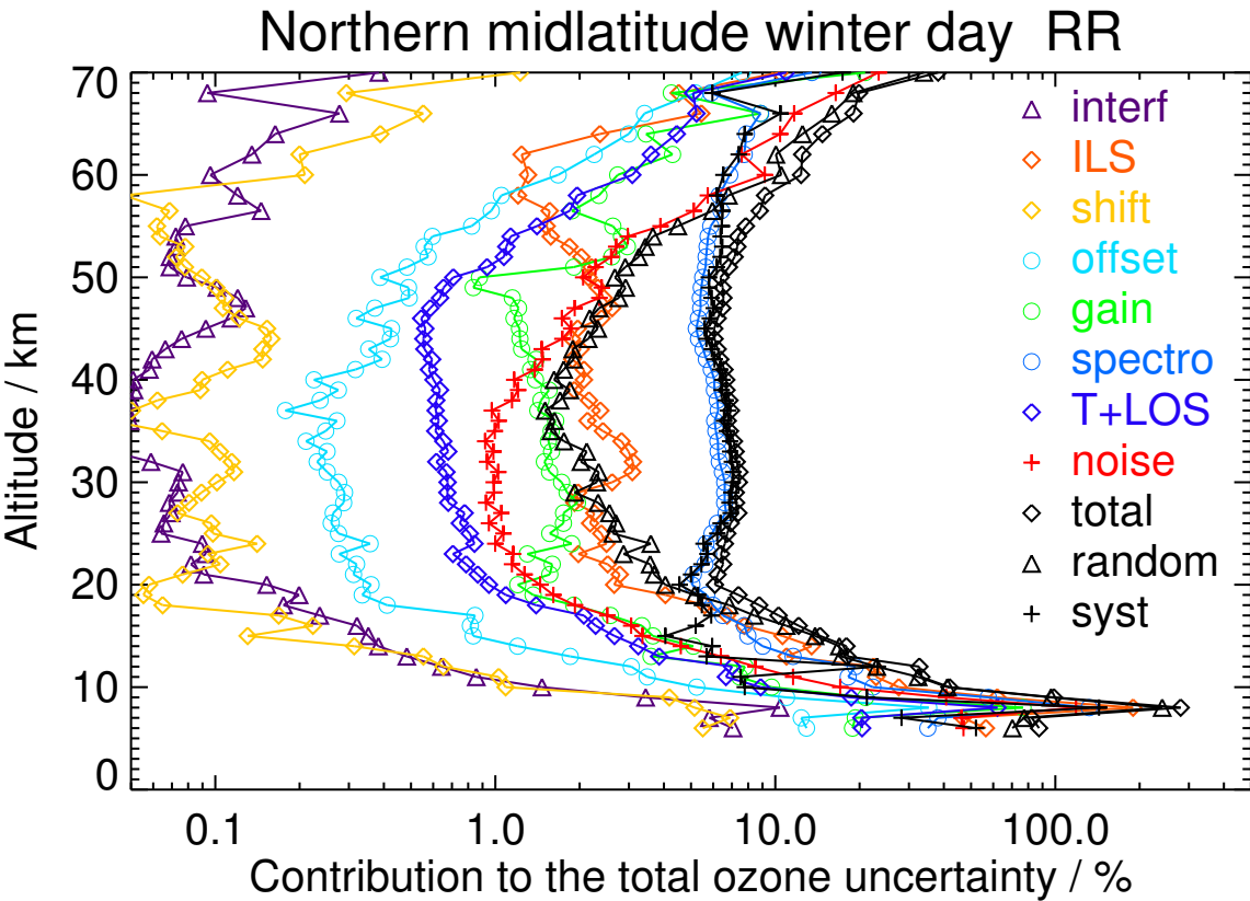
Figure S43. V8R_O3_261 Northern midlatitude winter day
