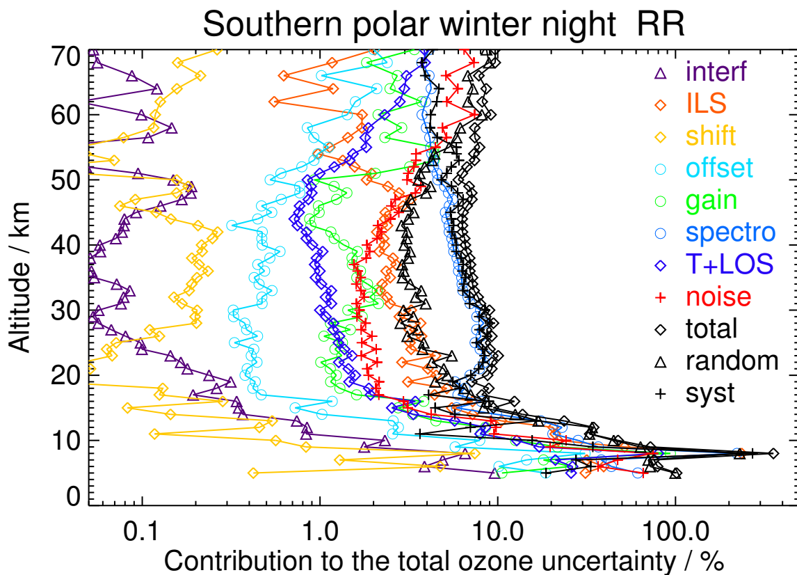
Figure S62. V8R_O3_261 Southern polar winter night
