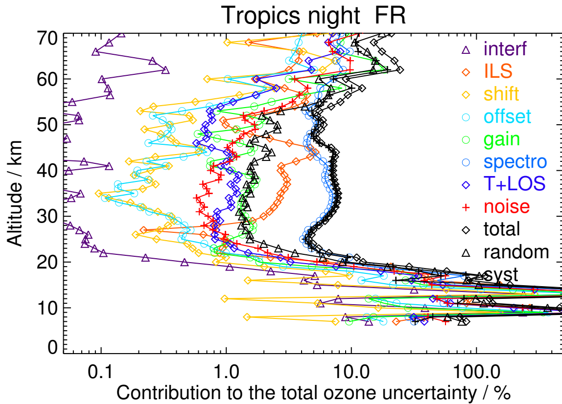
Figure S18. V8H_O3_61 Tropics night
