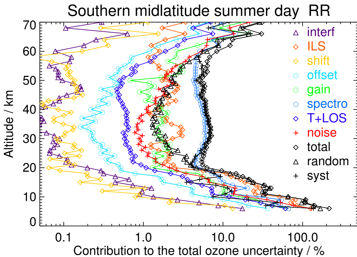
Figure S57. V8R_O3_261 Southern midlatitude summer day
