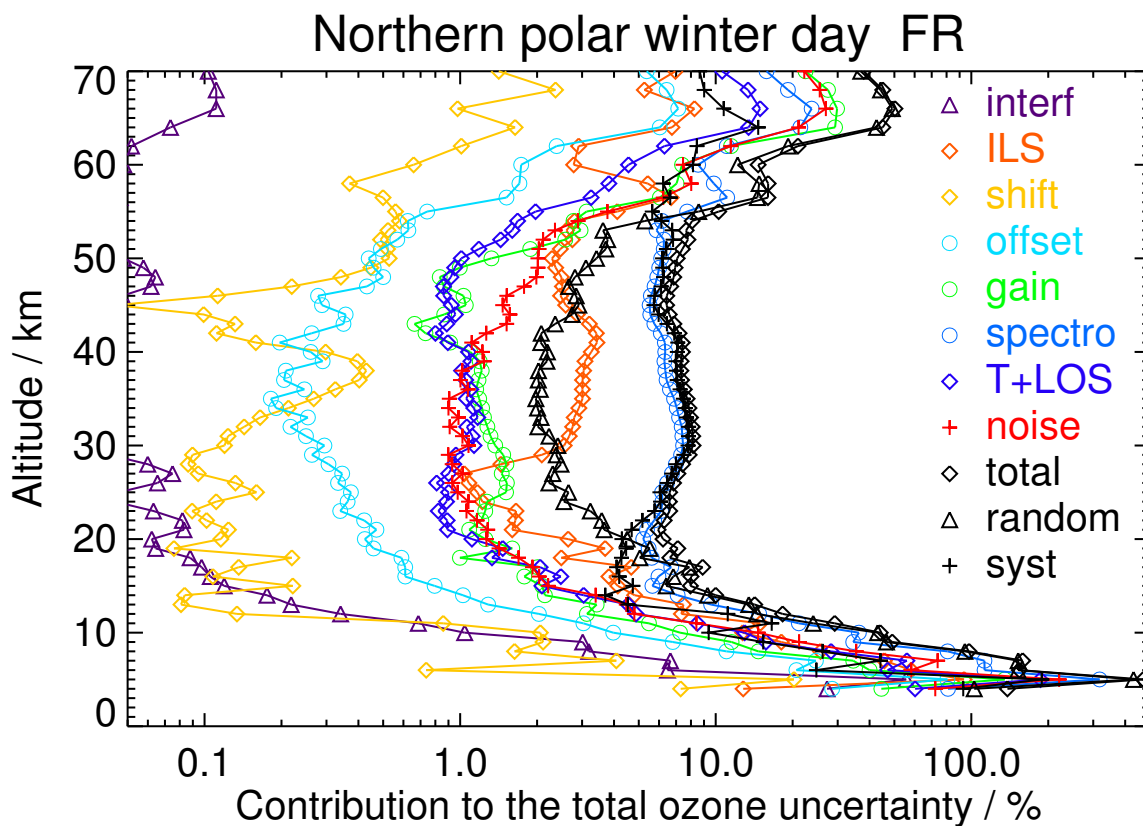
Figure S1. V8H_O3_61 Northern polar winter day
