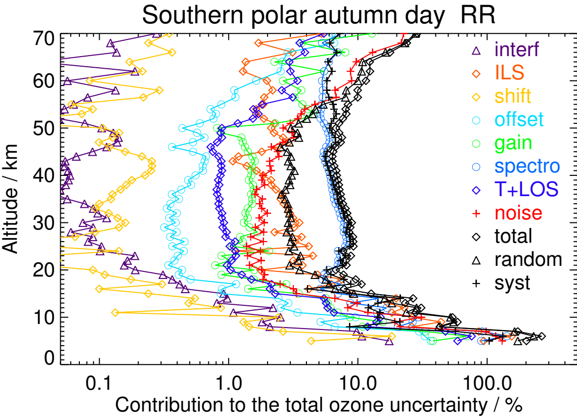
Figure S67. V8R_O3_261 Southern polar autumn day
