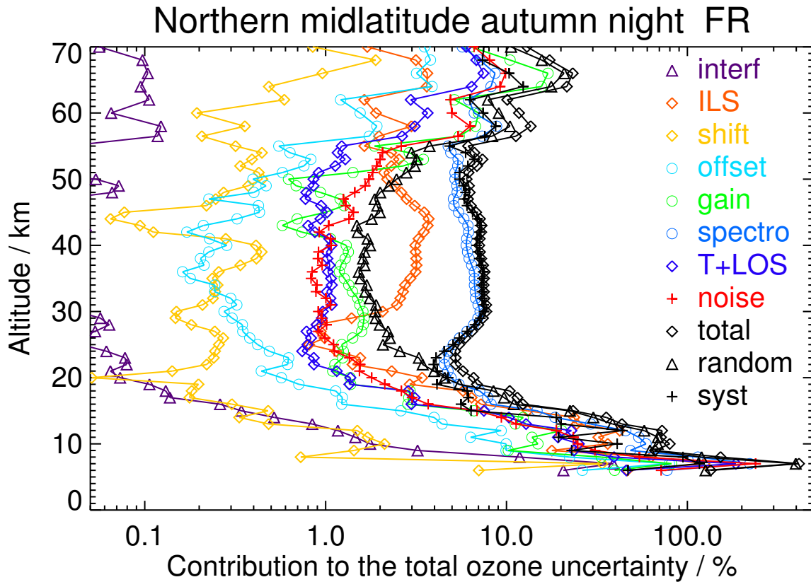
Figure S16. V8H_O3_61 Northern midlatitude autumn night
