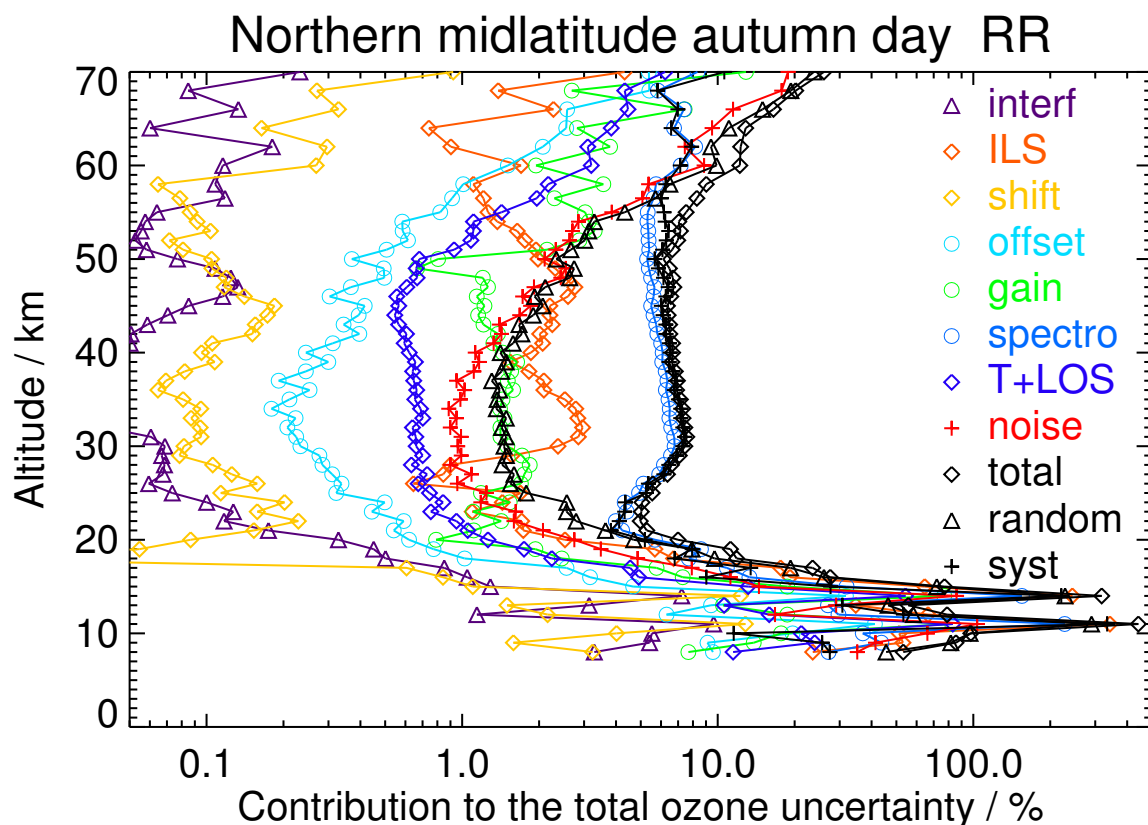
Figure S49. V8R_O3_261 Northern midlatitude autumn day
