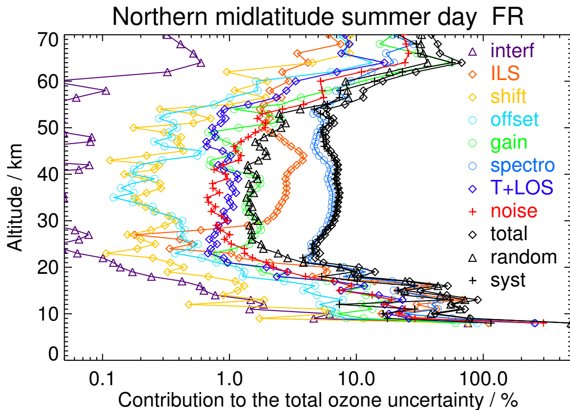
Figure S13. V8H_O3_61 Northern midlatitude summer day
