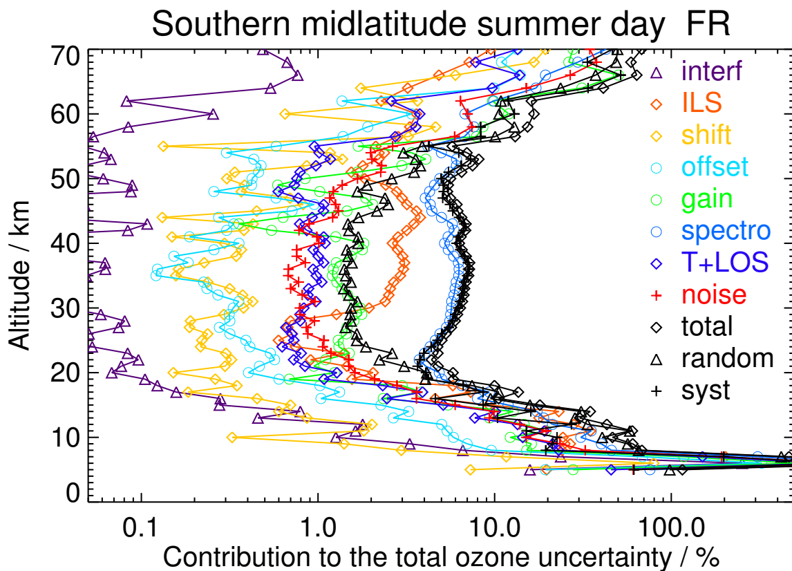
Figure S23. V8H_O3_61 Southern midlatitude summer day
