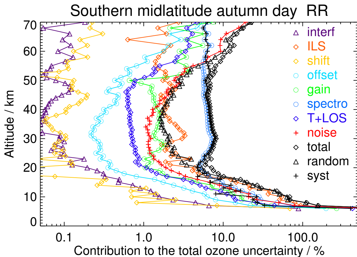
Figure S59. V8R_O3_261 Southern midlatitude autumn day
