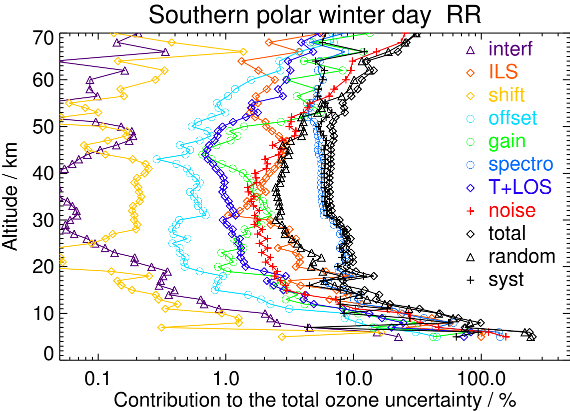
Figure S61. V8R_O3_261 Southern polar winter day
