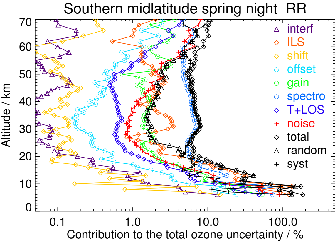
Figure S56. V8R_O3_261 Southern midlatitude spring night
