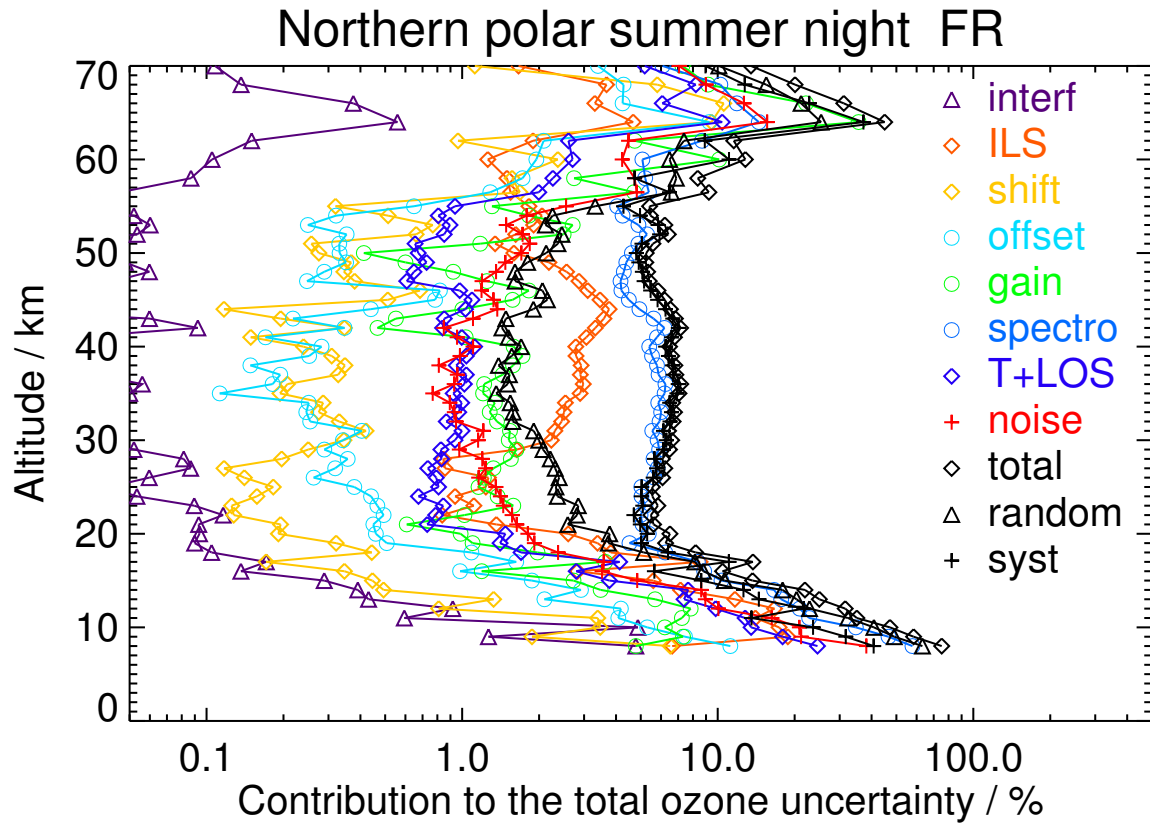
Figure S6. V8H_O3_61 Northern polar summer night
