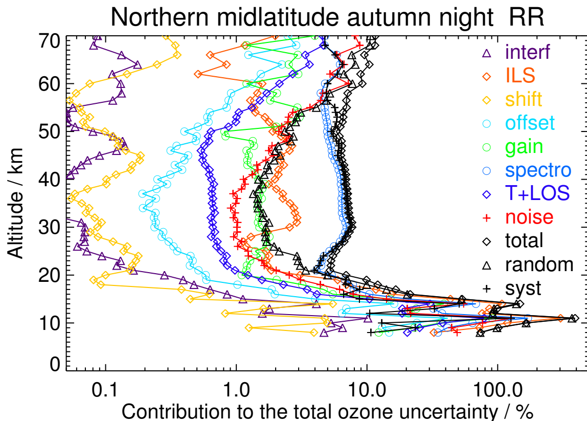
Figure S50. V8R_O3_261 Northern midlatitude autumn night
