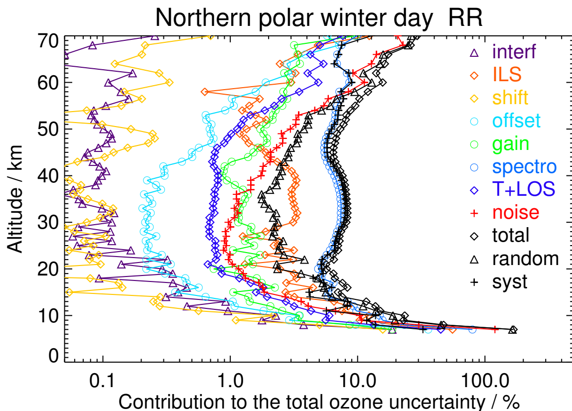
Figure S35. V8R_O3_261 Northern polar winter day
