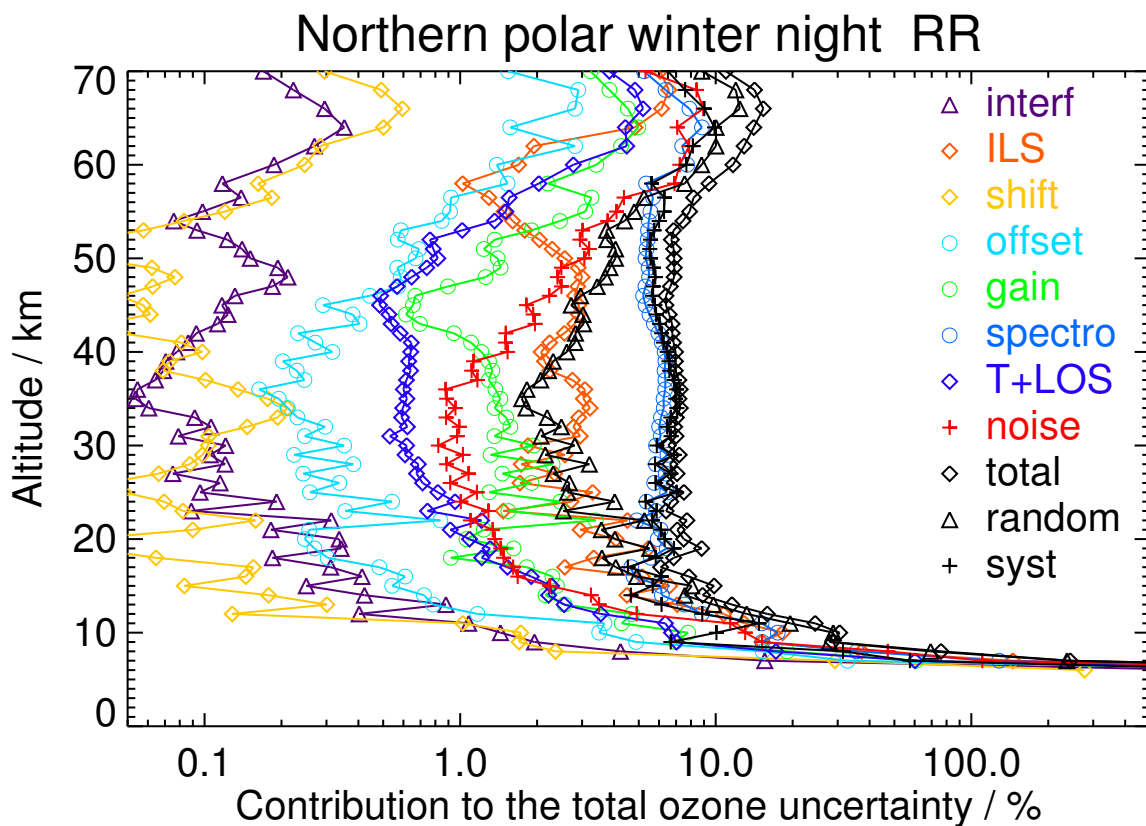
Figure S36. V8R_O3_261 Northern polar winter night
