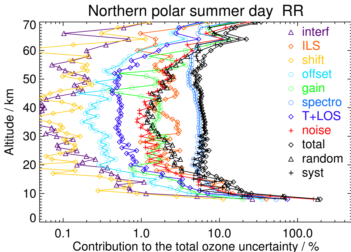
Figure S39. V8R_O3_261 Northern polar summer day
