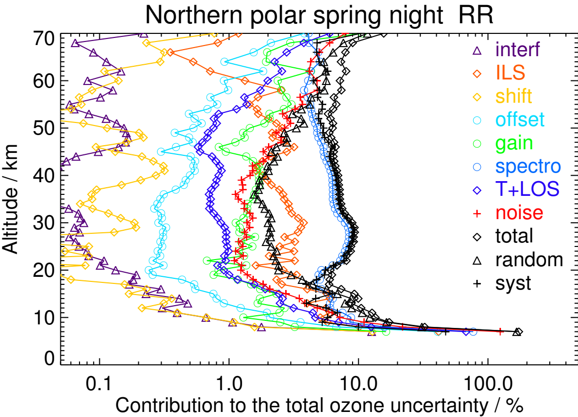
Figure S38. V8R_O3_261 Northern polar spring night
