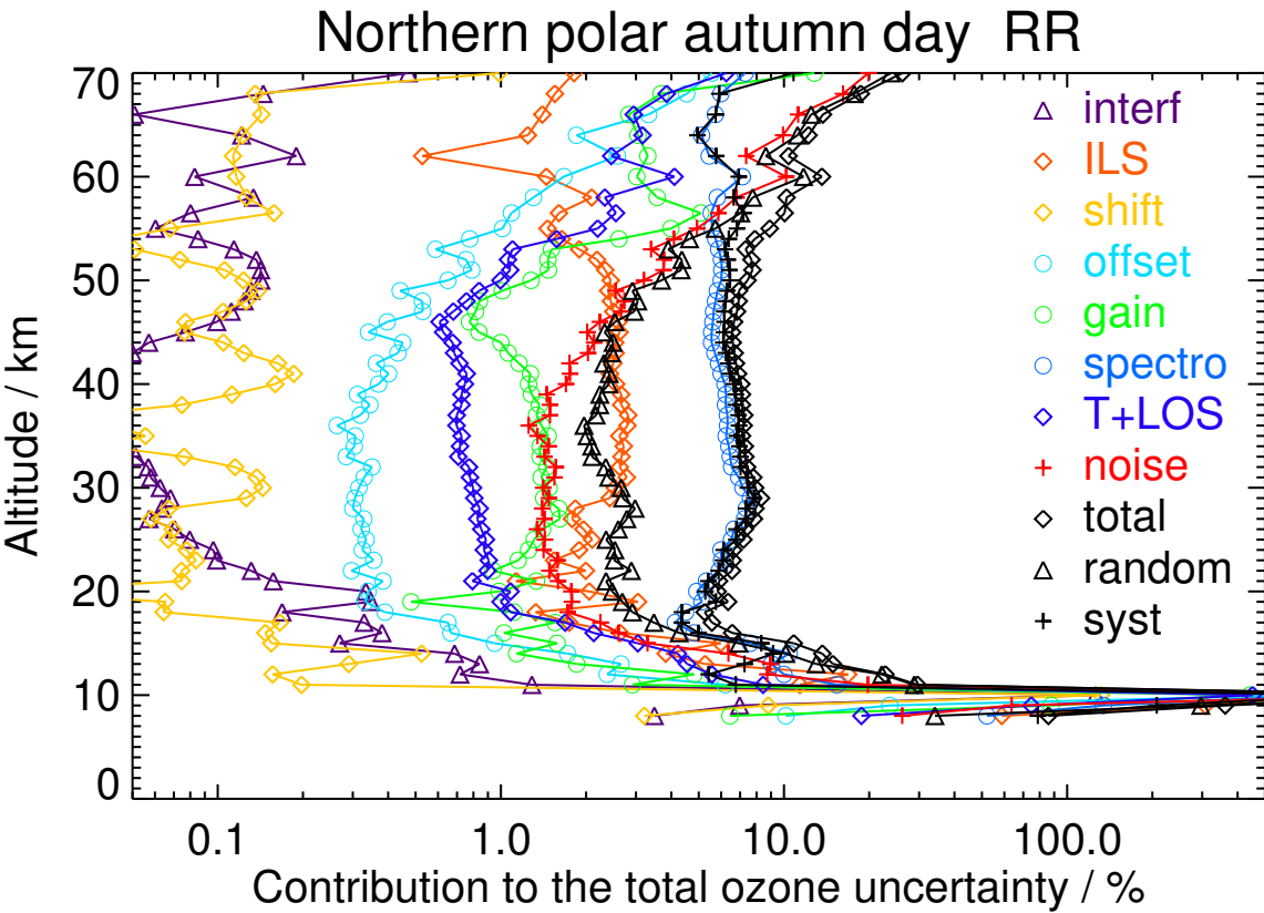
Figure S41. V8R_O3_261 Northern polar autumn day
