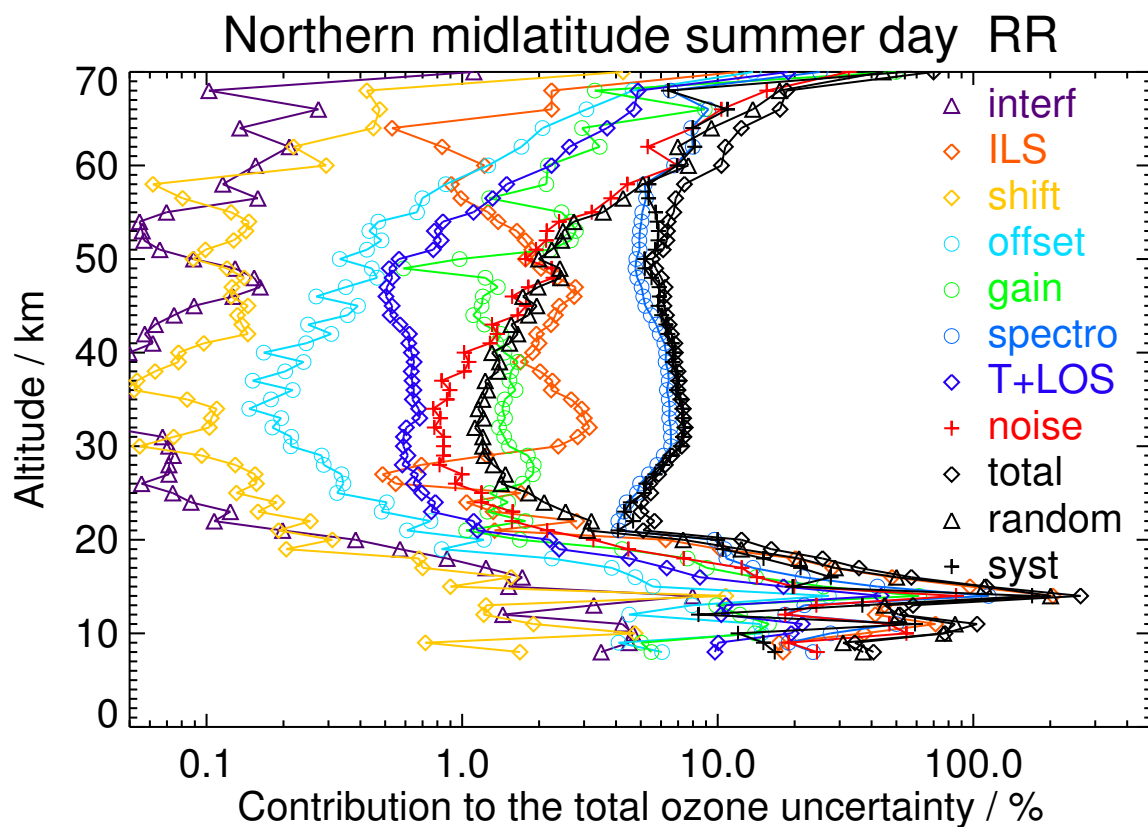
Figure S47. V8R_O3_261 Northern midlatitude summer day
