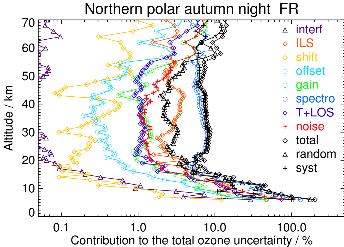
Figure S8. V8H_O3_61 Northern polar autumn night
