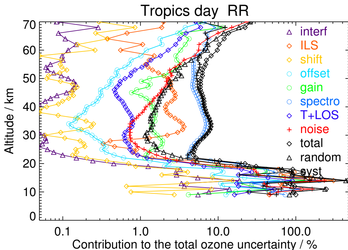
Figure S51. V8R_O3_261 Tropics day
