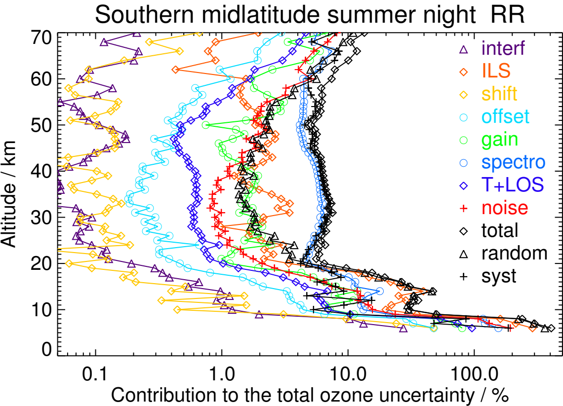
Figure S58. V8R_O3_261 Southern midlatitude summer night
