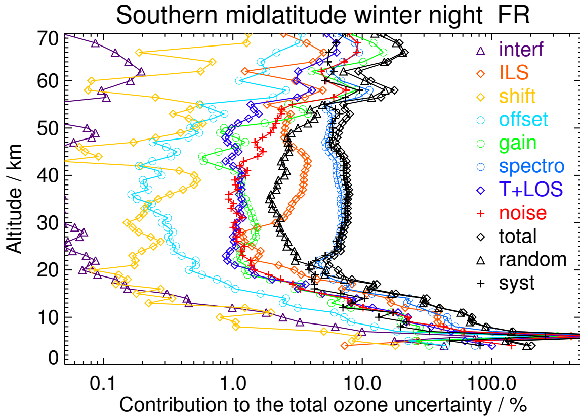
Figure S20. V8H_O3_61 Southern midlatitude winter night
