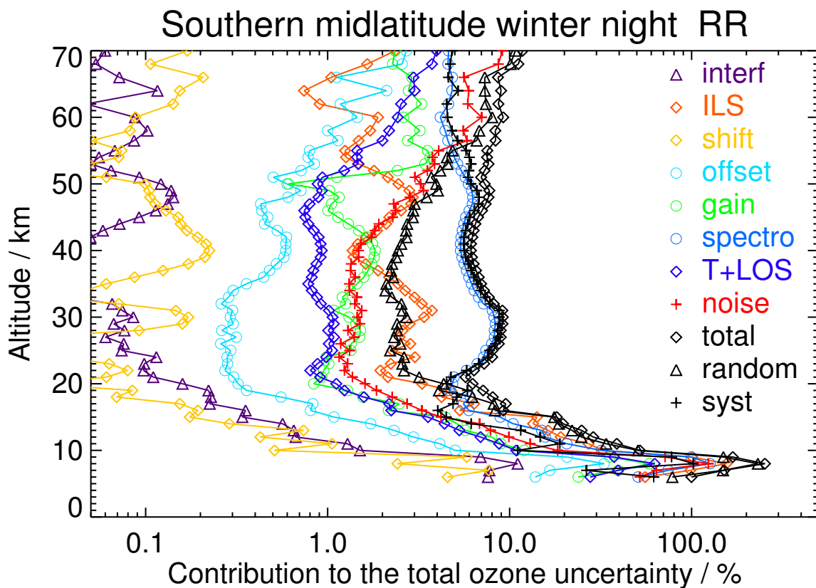
Figure S54. V8R_O3_261 Southern midlatitude winter night
