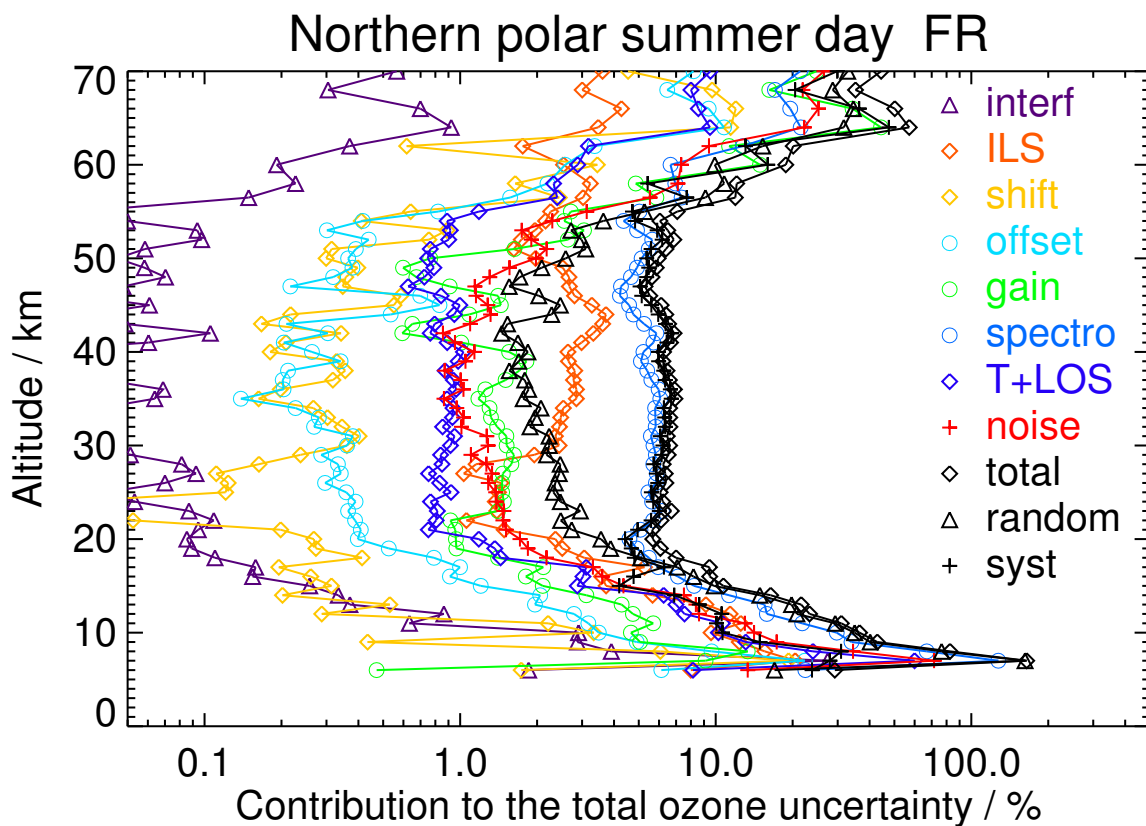
Figure S5. V8H_O3_61 Northern polar summer day
