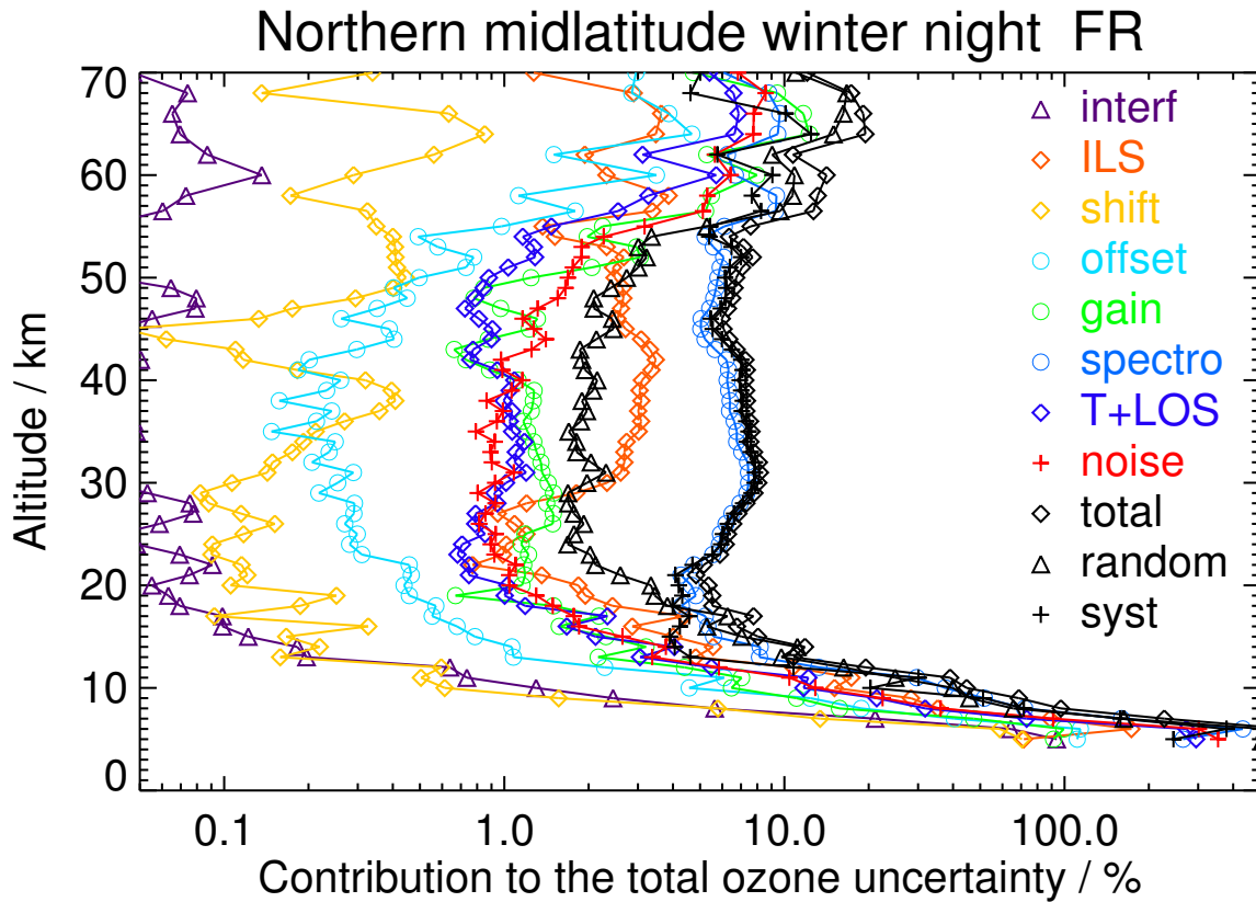
Figure S10. V8H_O3_61 Northern midlatitude winter night
