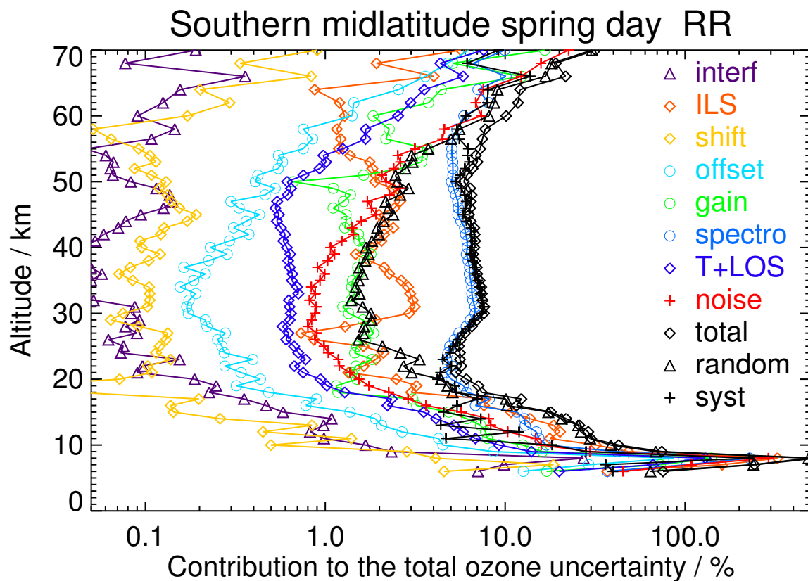
Figure S55. V8R_O3_261 Southern midlatitude spring day
