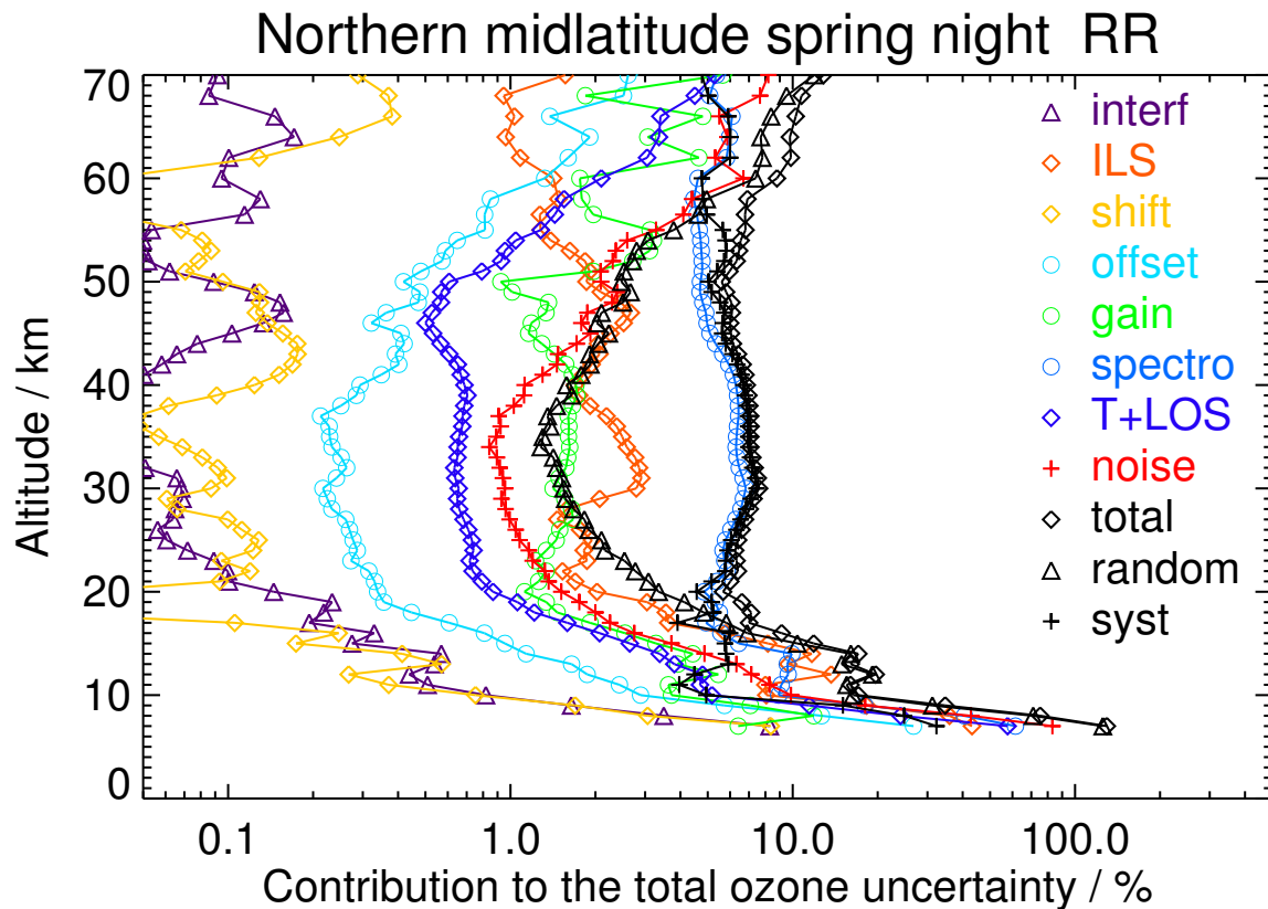
Figure S46. V8R_O3_261 Northern midlatitude spring night
