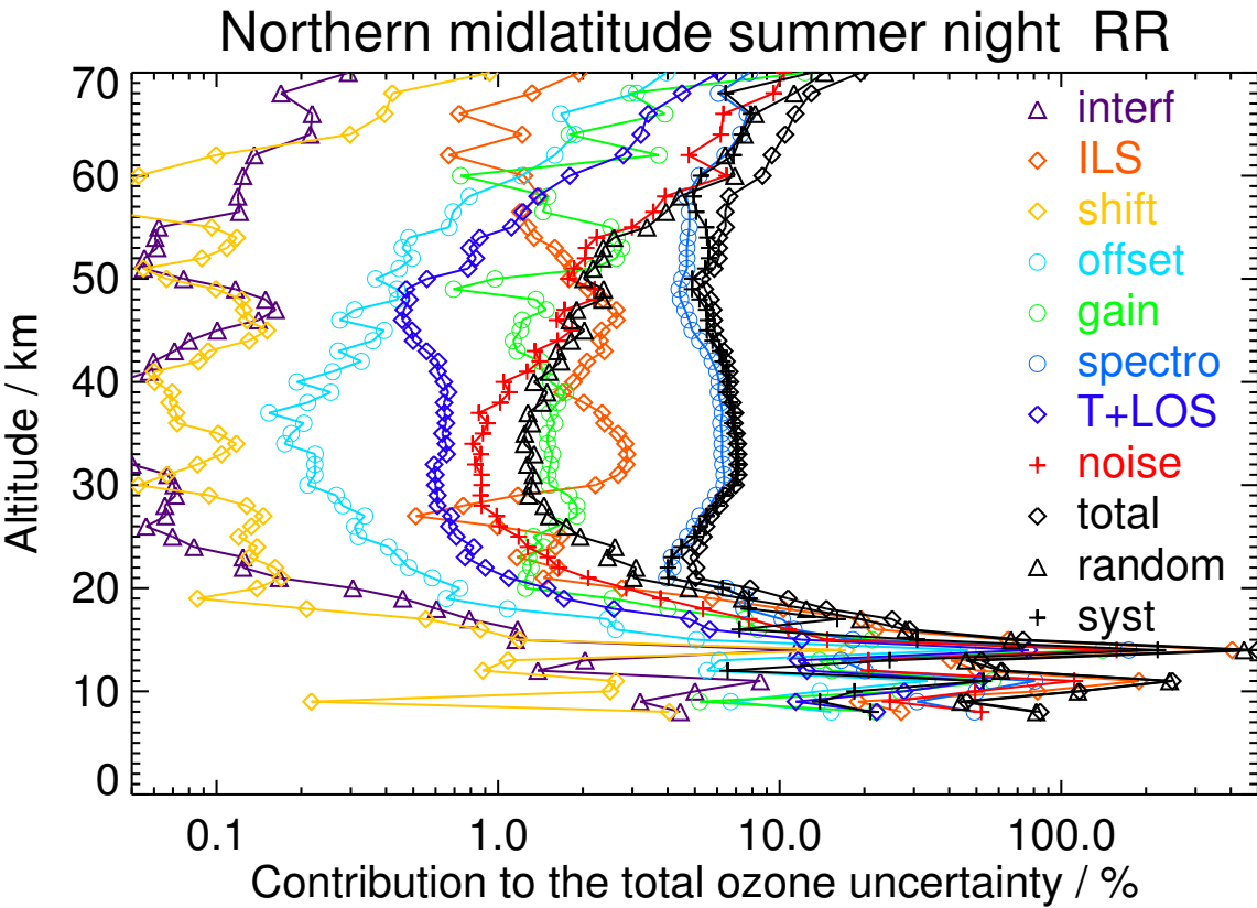
Figure S48. V8R_O3_261 Northern midlatitude summer night
