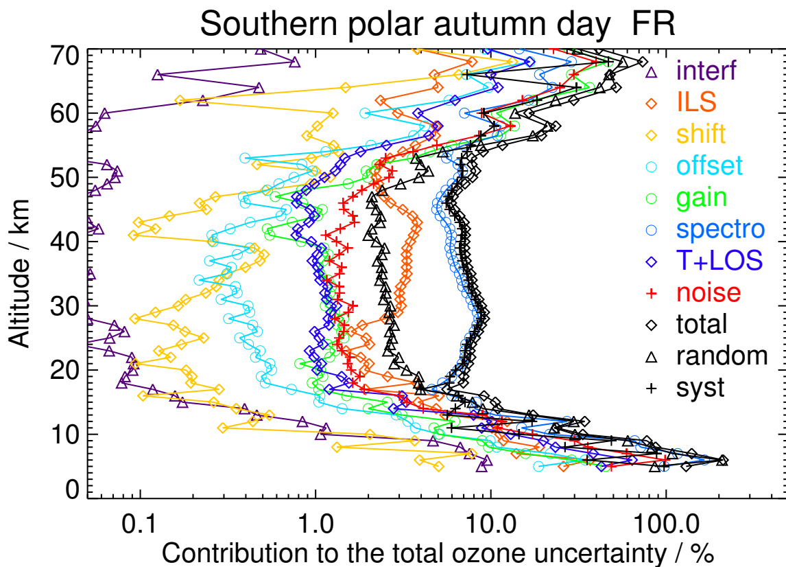
Figure S33. V8H_O3_61 Southern polar autumn day
