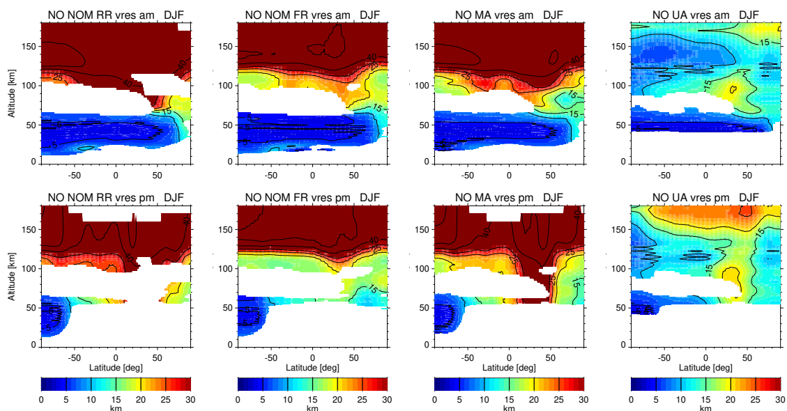
Figure 2. Zonal mean vertical resolution (in terms of full width at half maximum of the AK rows) of NO during the Northern winter season (DJF) from NOM RR measurements, NOM FR measurements, MA measurements and UA measurements as a function of latitude and altitude, separated for (top) am and (bottom) pm. White areas indicate data with insignificant information content (AK diagonal < 0.03 ). Note that NOM FR measurements are averaged over the 2002–2004 period, while measurements from other observation modes and periods are averaged over the 2006–2012 period.
