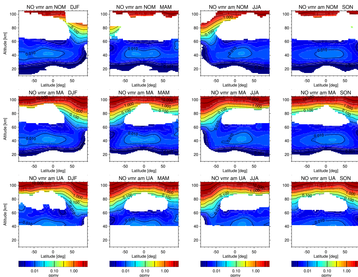
Figure 8. Seasonal composite zonal mean distributions of retrieved NO vmrs from (top to bottom) NOM RR, MA, and UA measurements at as function of latitude and altitude for am observations. White areas indicate data with insignificant information content (AK diagonal < 0.03 ).
