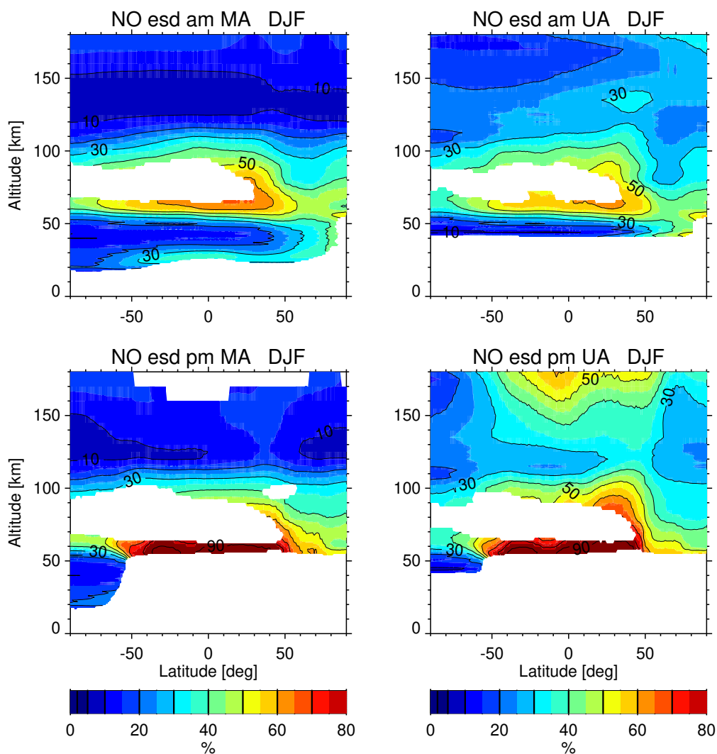
Figure 6. The measurement noise component of the NO retrieval error during the Northern winter season (DJF) for (left) MA and (right) UA measurements as function of latitude and altitude, separated for (top) am and (bottom) pm. White areas indicate data with insignificant information content (AK diagonal < 0.03).
