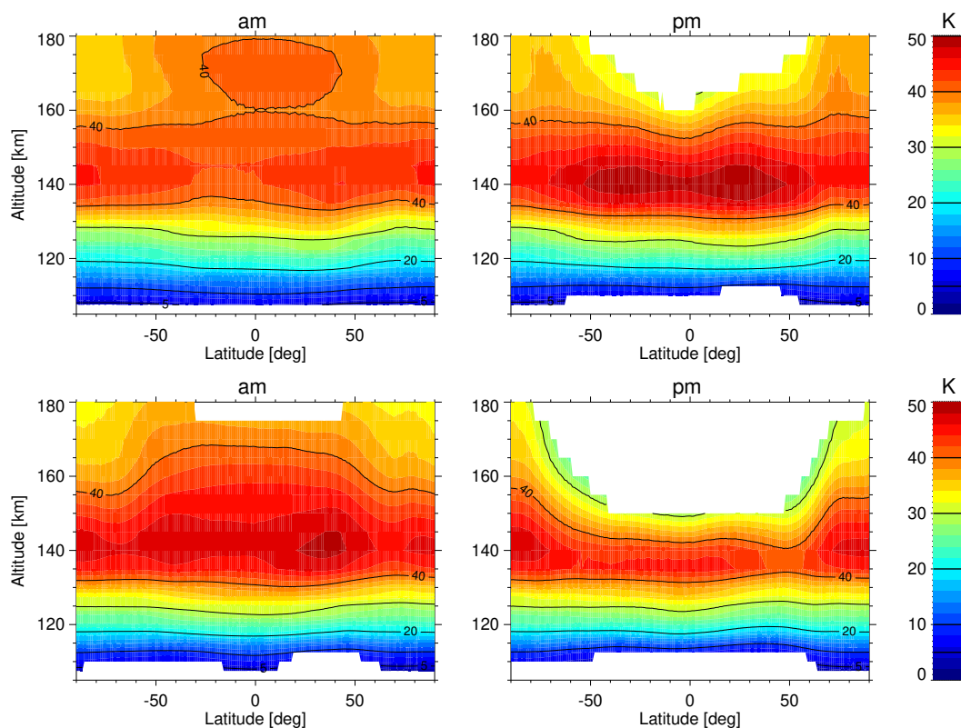
Figure 7. The noise component of the UA temperature retrieval error in the lower thermosphere as function of latitude and altitude, separated for (left) am and (right) pm, as well as for high solar activity conditions (averaged over the years 2005, 2006, 2011, 2012, top) and low solar activity conditions (averaged over the years 2007-2010, bottom). White areas indicate data with insignificant information content (AK diagonal < 0.03 ).
