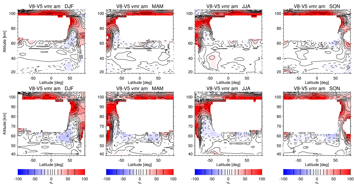
Figure 11. Seasonal composite zonal mean distributions of the relative NO vmr differences between am observations of version 8 and version 5 as a function of latitude and altitude for (top) MA and (bottom) UA. Specifically, version 5 data used here are V5r_NO_521 (MA) and V5r_NO_622 (UA).
