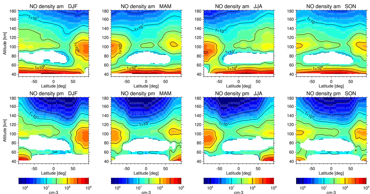
Figure 12. Seasonal composite zonal mean distributions of retrieved NO densities from UA measurements as a function of latitude and altitude, separated for (top) am and (bottom) pm. White areas indicate data with insignificant information content (AK diagonal < 0.03).
