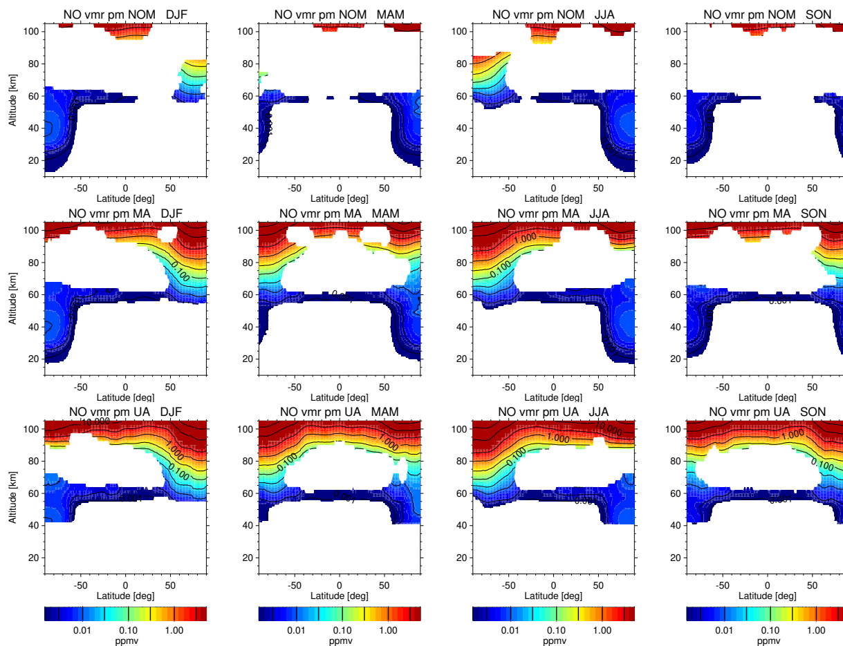
Figure 9. As Figure 8, but for pm observations.
