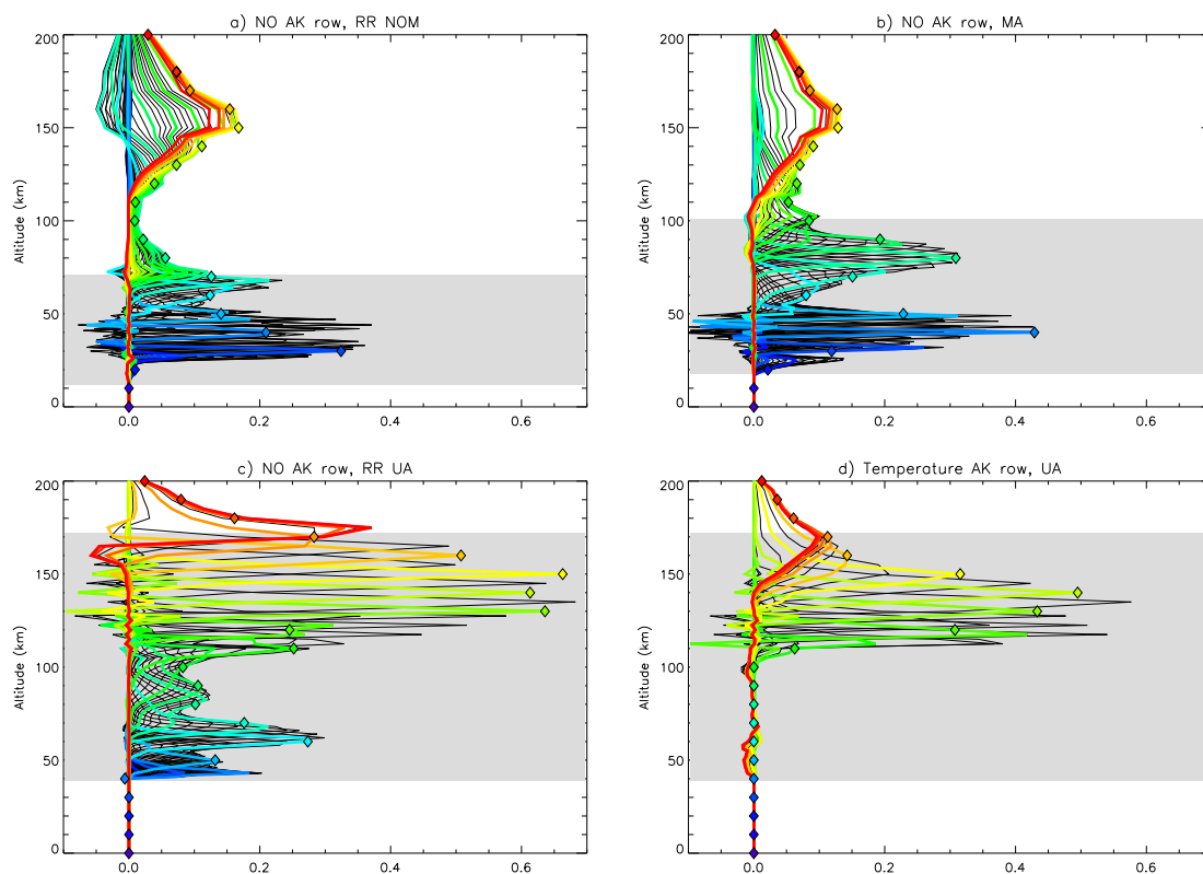
Figure 1. Example averaging kernel rows of the retrieved NO from (a) NOM RR measurements, (b) MA measurements, (c) UA measurements, and (d) of the retrieved temperature from UA measurements. Rows corresponding to profile altitudes of 0,10,20,...200 km are highlighted with colored lines. The corresponding averaging kernel diagonal elements are indicated by symbols. The vertical scan range of the respective measurements is indicated by grey-shading. All averaging kernels shown belong to daytime measurements taken in January 2012 at latitudes around 55°N.
