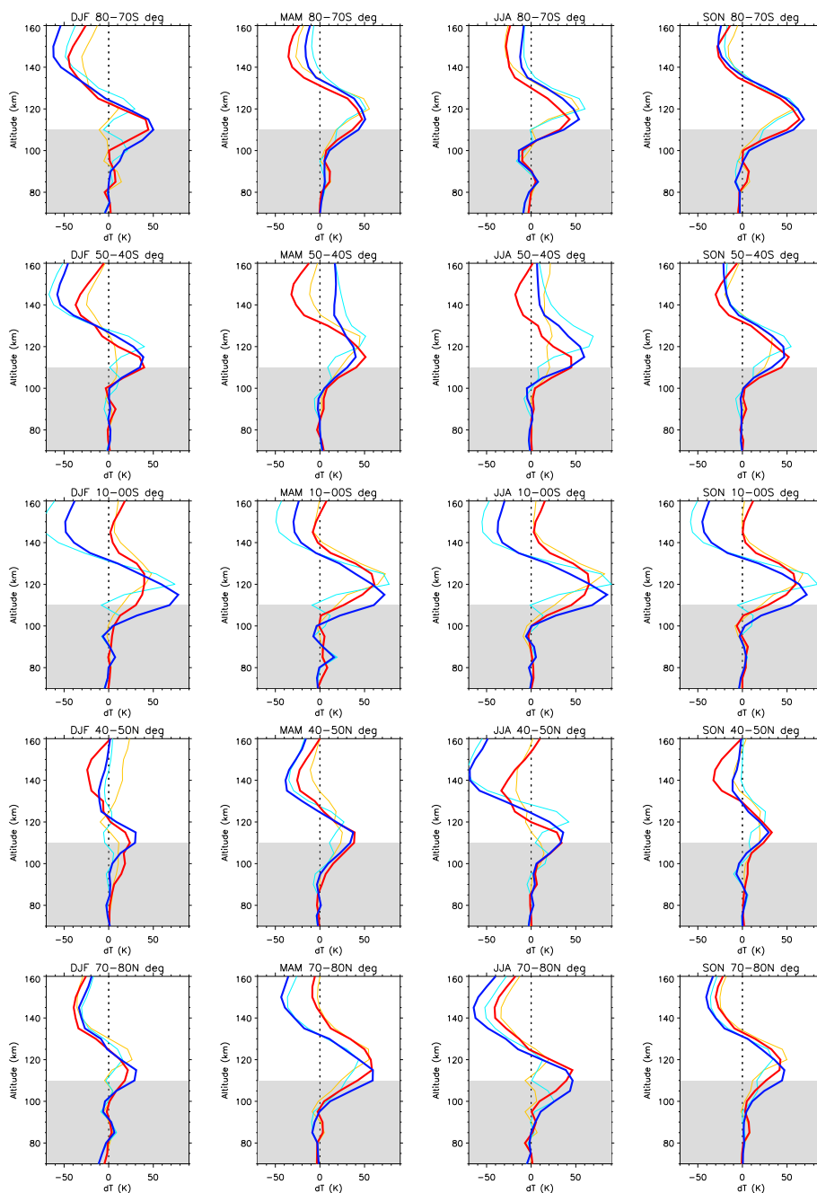
Figure 19. Seasonal mean temperature differences between MIPAS and NRLMSIS2.0 temperatures for various latitude bands. MIPAS version 8–NRLMSIS2.0 is shown for am (red) and pm (dark blue) observations. MIPAS version 5–NRLMSIS2.0 is shown for am (orange) and pm (light blue) for comparison. The grey-shaded areas indicate the vertical range where MIPAS temperatures are from the 15\ \mu\text{m} retrievals.
