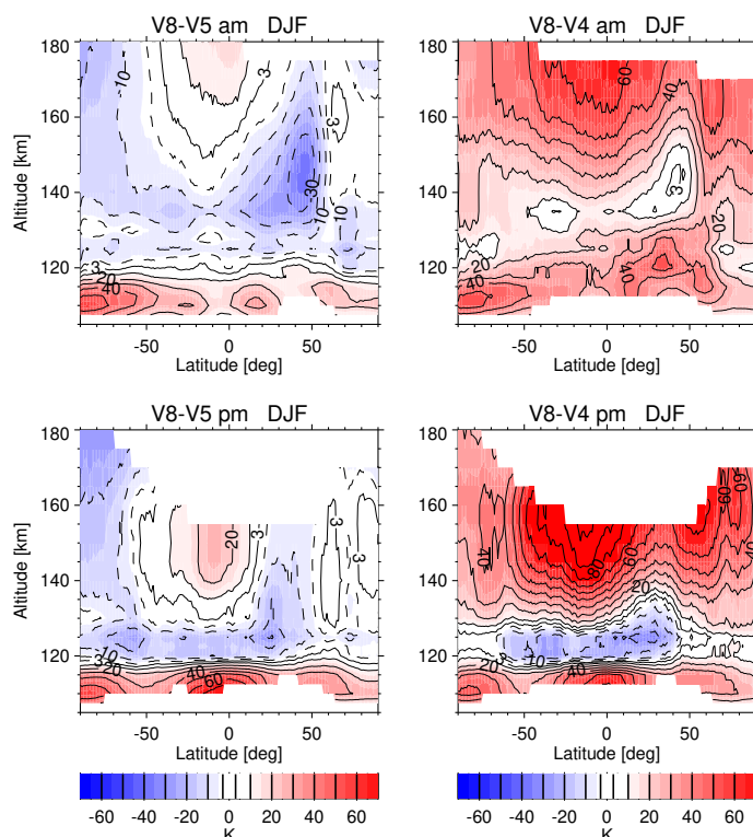
Figure 17. Northern winter (DJF) composite zonal mean distributions of the temperature differences between UA data version 8 with respect to (left) version 5 (V5r_TwNO_622) and (right) version 4 (V4r_TwNO_611) as function of latitude and altitude, separated for am (top) and pm (bottom).
