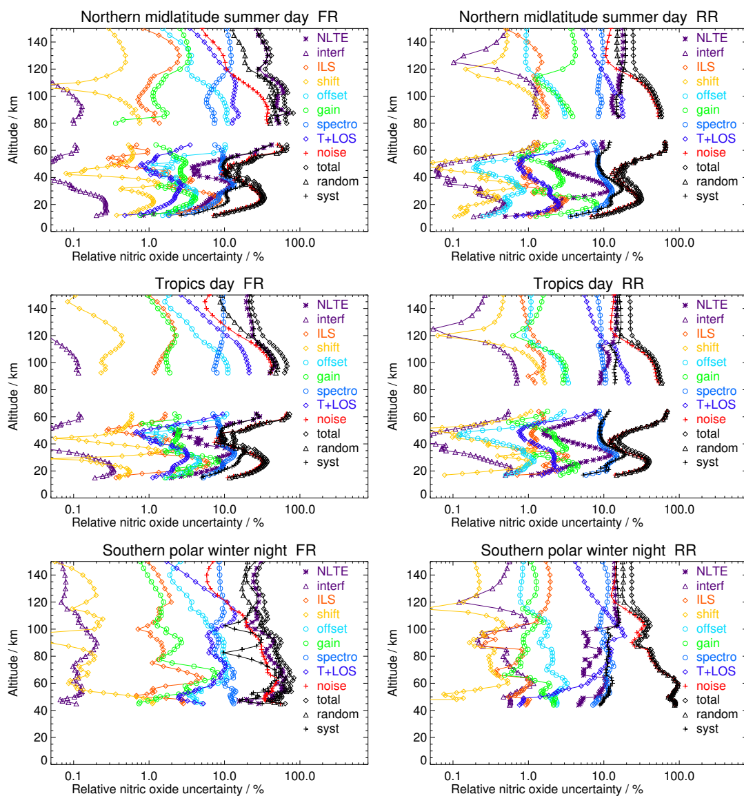
Figure 5. NO error budget for FR (a, c, e) and RR (b, d, f) NOM data. Additive and multiplicative errors are shown as relative errors of the respective NO vmr profiles. All error estimates are 1-\sigma uncertainties. Error contributions are marked “T+LOS” for the propagated error from the T+LOS retrieval, “noise” for error due to measurement noise, “spectro” for spectroscopic error, “gain” for gain calibration error (see text), “shift” for spectral shift error (see text), “ILS” for instrument line shape error (see text), “offset” for error due to spectral offset (see text), “interf” for the error due to interfering gases, and “NLTE” for non-LTE related errors. (a, b) northern midlatitude summer day, (c, d) tropical day, and (e, f) southern polar winter night.
