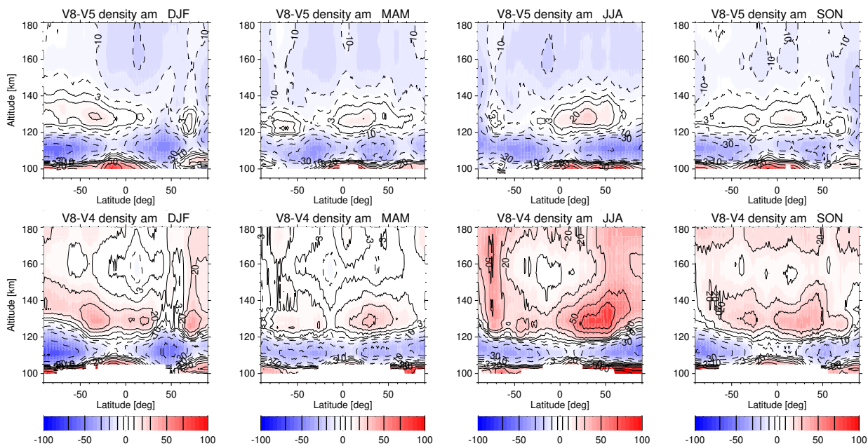
Figure 13. Seasonal composite zonal mean distributions of the relative NO density differences between am measurements of different UA data versions as a function of latitude and altitude: (top) V8R_NOwT_662 versus V5r_NOwT_622 and (bottom) V8r_NOwT_662 versus V4R_NOwT_611.
