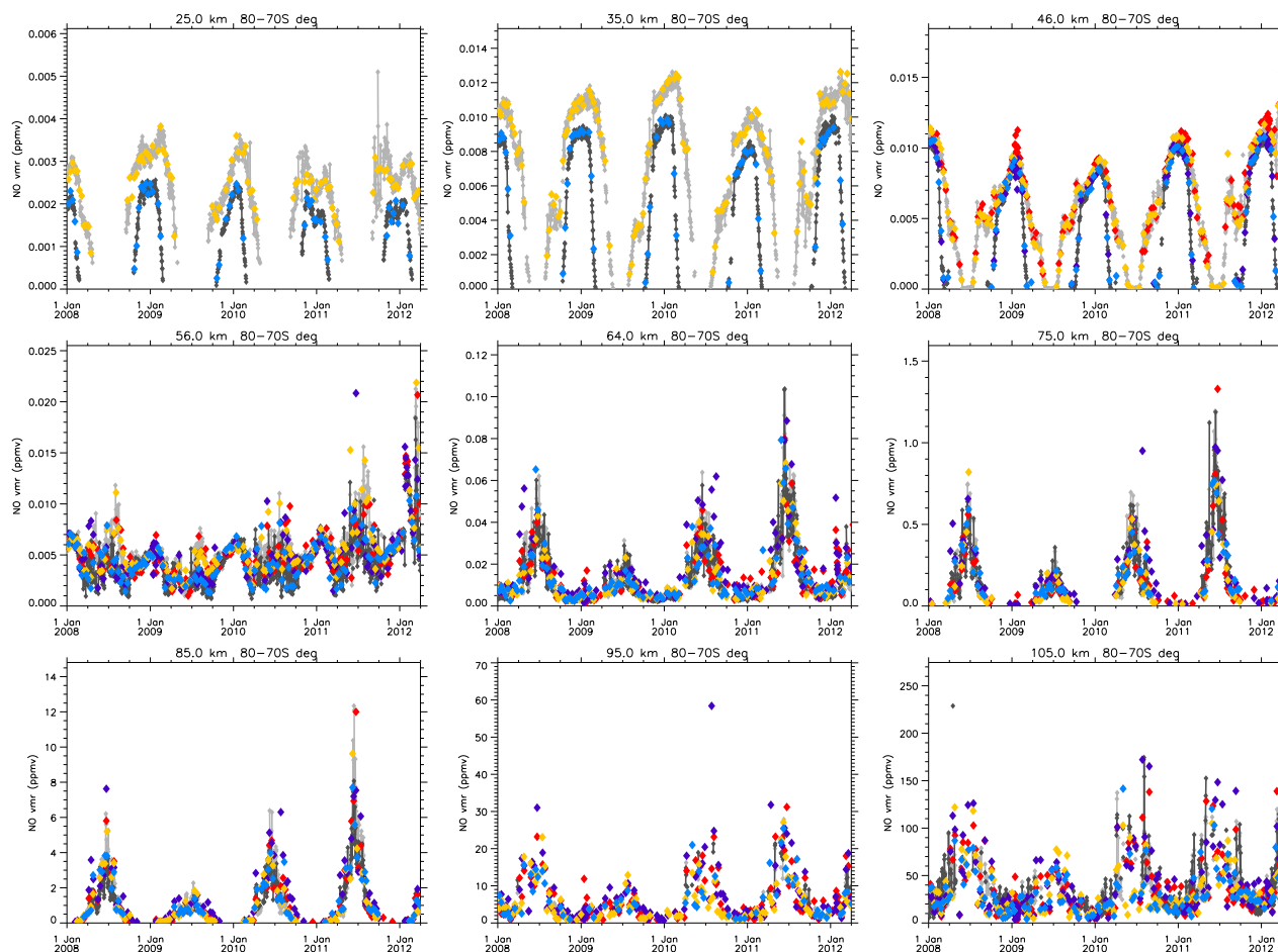
Figure 15. Time series of daily zonal mean NO vmr at various altitudes (as indicated in the plot titles) from NOM RR (grey: am, black: pm), MA (orange: am, light blue: pm), and UA (red: am, dark blue: pm) measurements during 2008–2012 at 70°S–80°S latitude.
