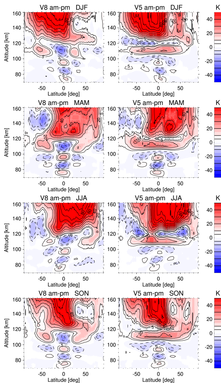
Figure 18. Seasonal composites of zonal mean temperature differences between am and pm observations of (left) version 8 and (right) version 5.
