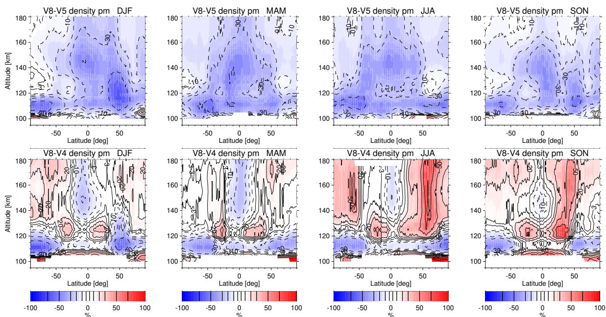
Figure 14. As Fig. 13, but for pm observations.
