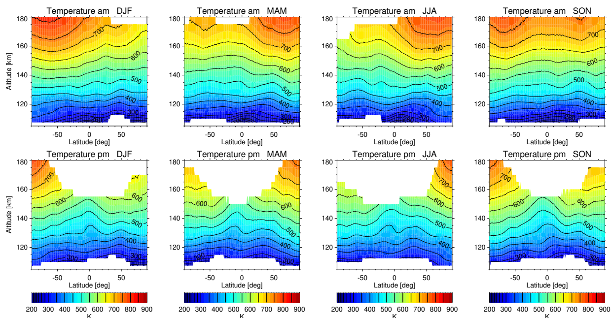
Figure 16. Seasonal composite zonal mean distributions of retrieved temperatures from UA observations as function of latitude and altitude, separated for am (top) and pm (bottom). White areas indicate data with insignificant information content (AK diagonal < 0.03).
