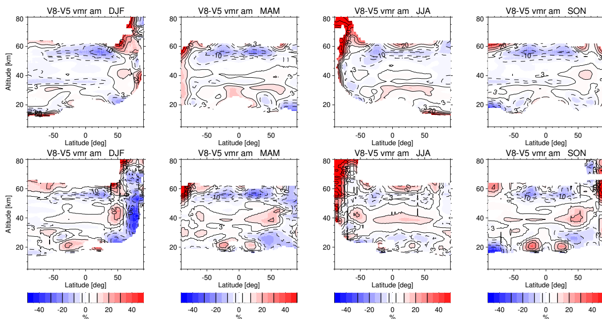
Figure 10. Seasonal composite zonal mean distributions of the relative NO vmr differences between version 8 and version 5 as a function of latitude and altitude for (top) NOM RR and (bottom) NOM FR am observations. Specifically, version 5 data used here are V5r_NO_221/220 (RR) and V5h_NO_20 (FR).
